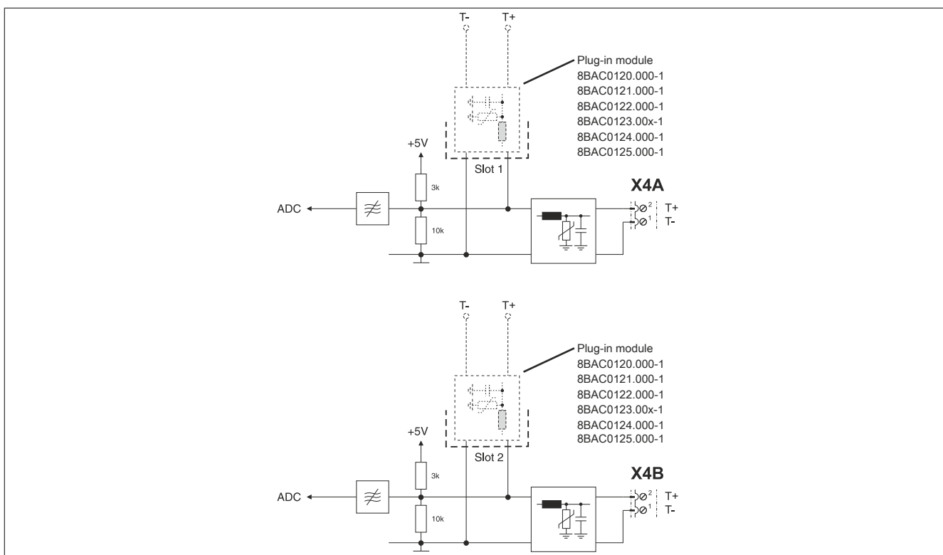
Figure 8: Temperature sensor
