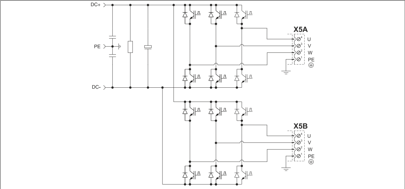
Figure 9: Motor
