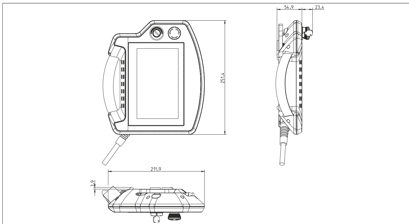
Figure 17: 5MP7140.070N-000 - Dimensions
