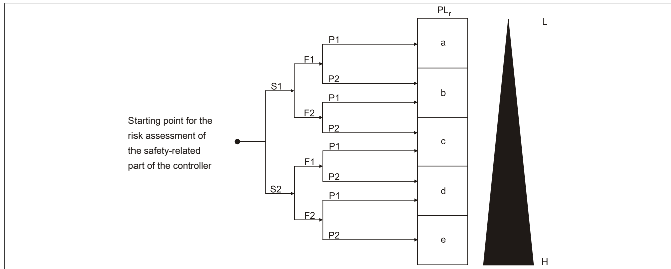
Figure 40: Risk graph for determining the PLr for each safety function
