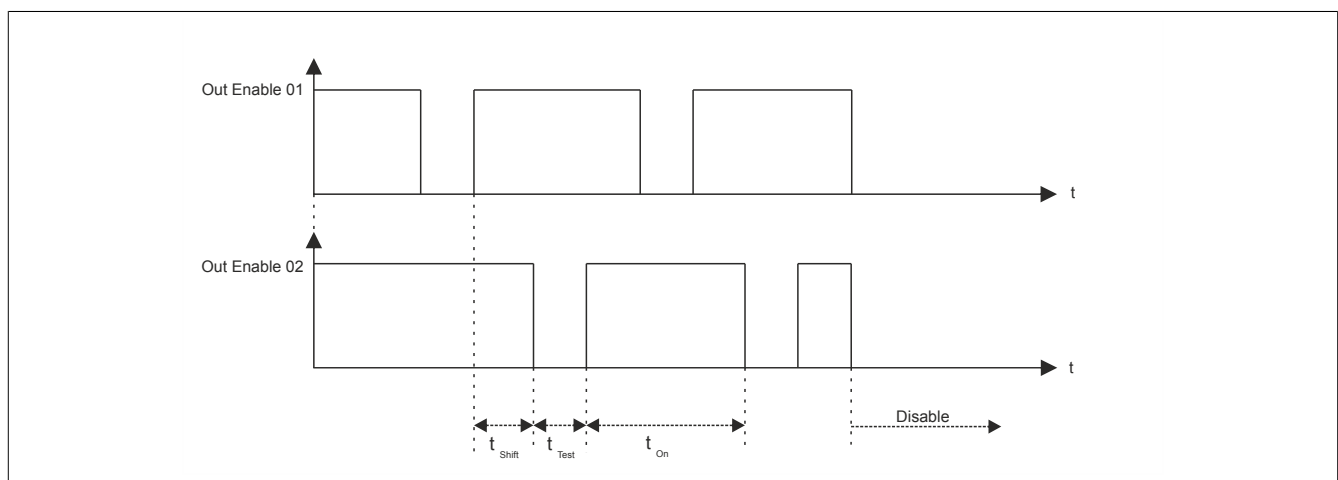
Figure 6: Enabling electronics - Testing for short circuits and cross faults
