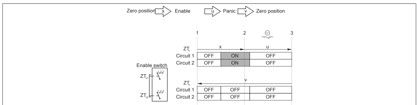
Figure 5: Contact travel diagram for panic actuation
