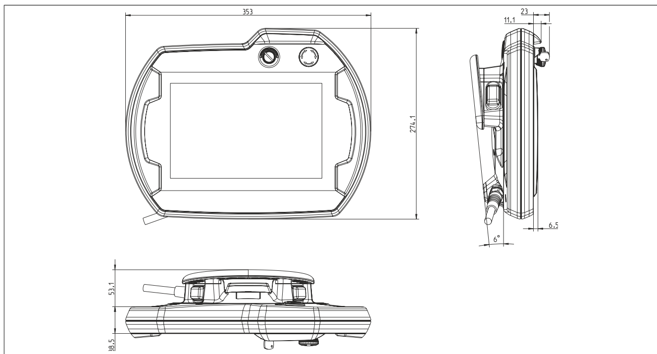
Figure 23: 5MP7151.101E-000 - Dimensions
