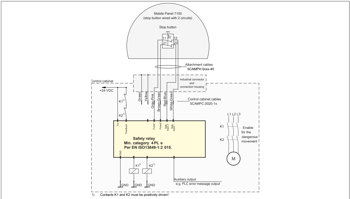
Figure 28: Connection example for stop button for MP7100
