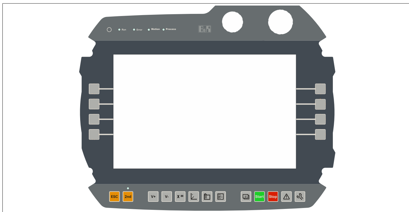
Figure 10: MP7150 - Membrane keypad
