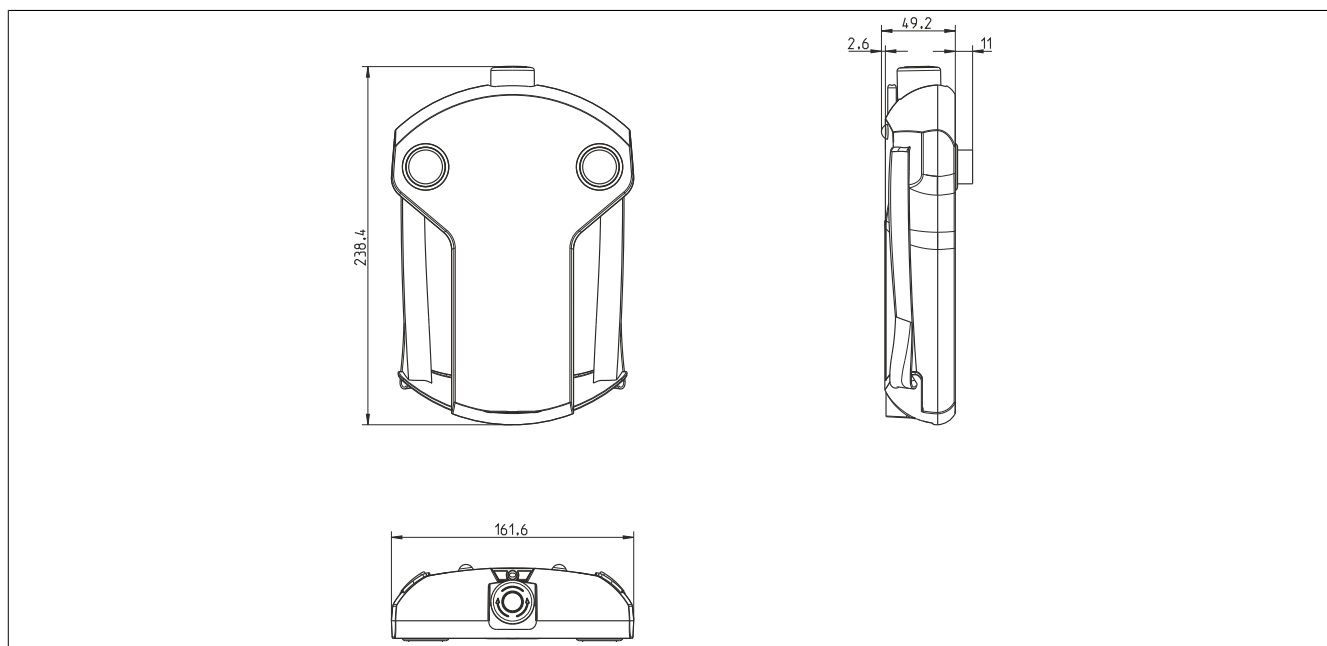
Figure 13: 5MP7120.034F-000 - Dimensions
