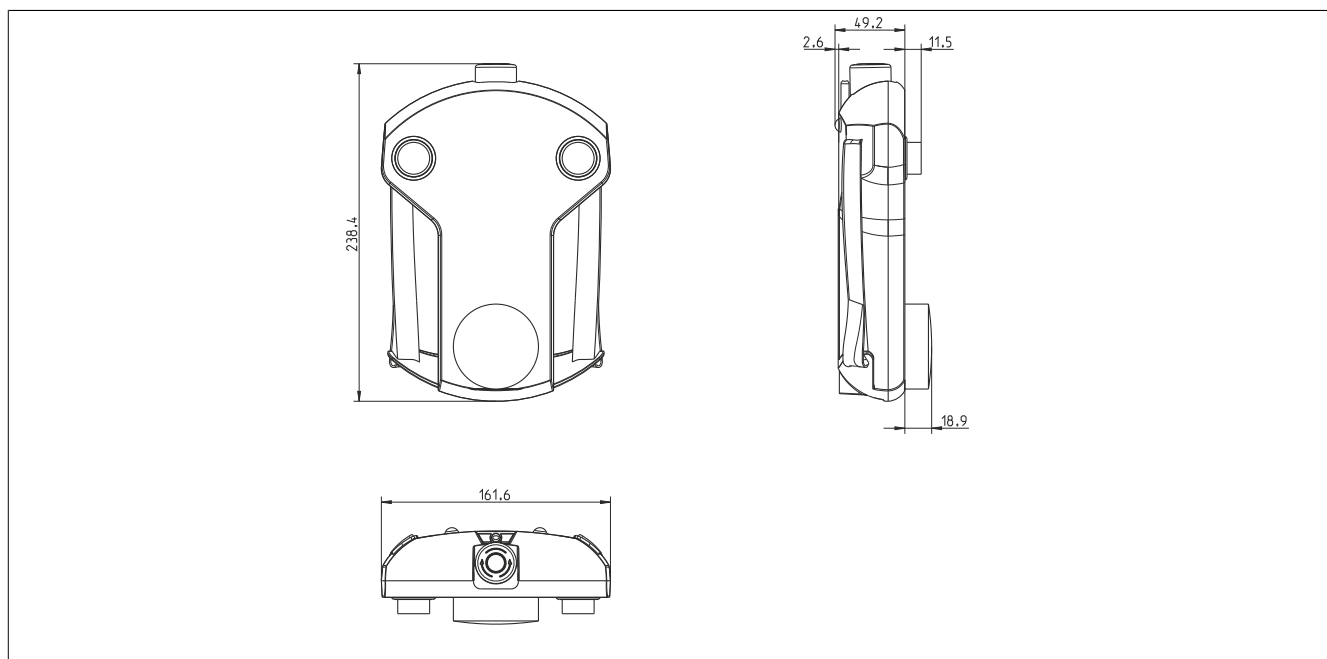
Figure 15: 5MP7121.034F-000 - Dimensions
