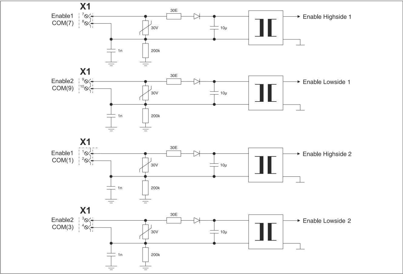
Figure 6: Enable
