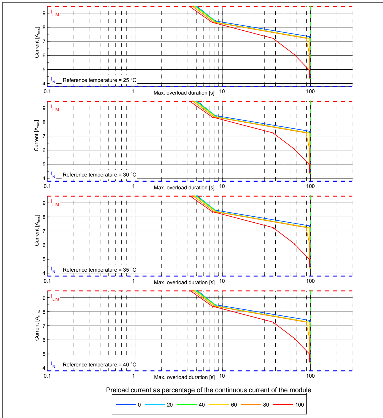
Figure 2: 8BVI0028HWDx.000-1 - Overload characteristics, overload response - ERROR+STOP
