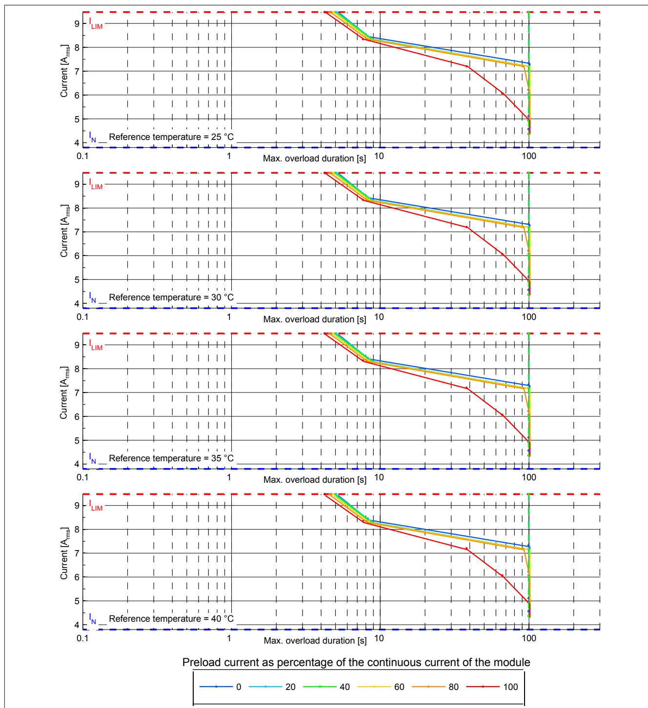
Figure 1: 8BVI0028HWDx.000-1 - Overload characteristics, overload response - WARNING
