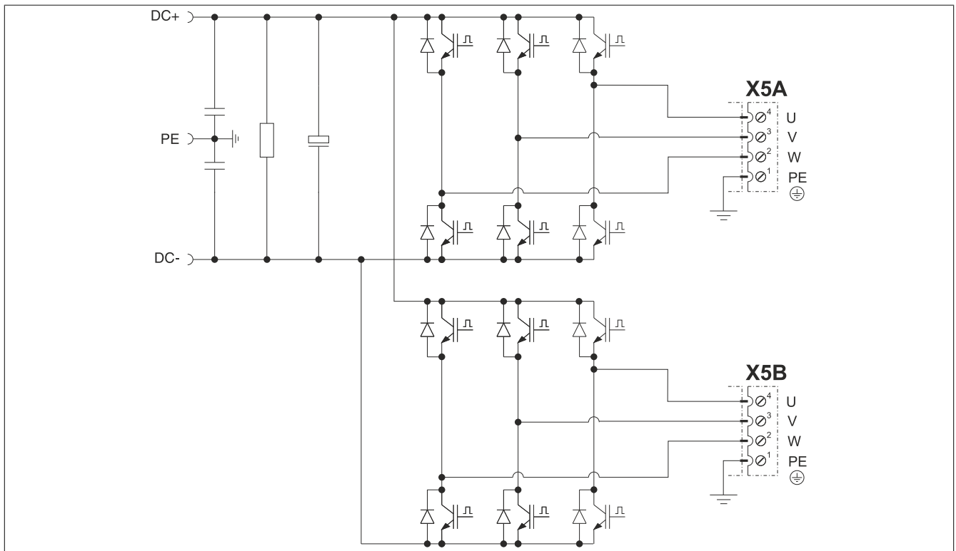
Figure 9: Motor
