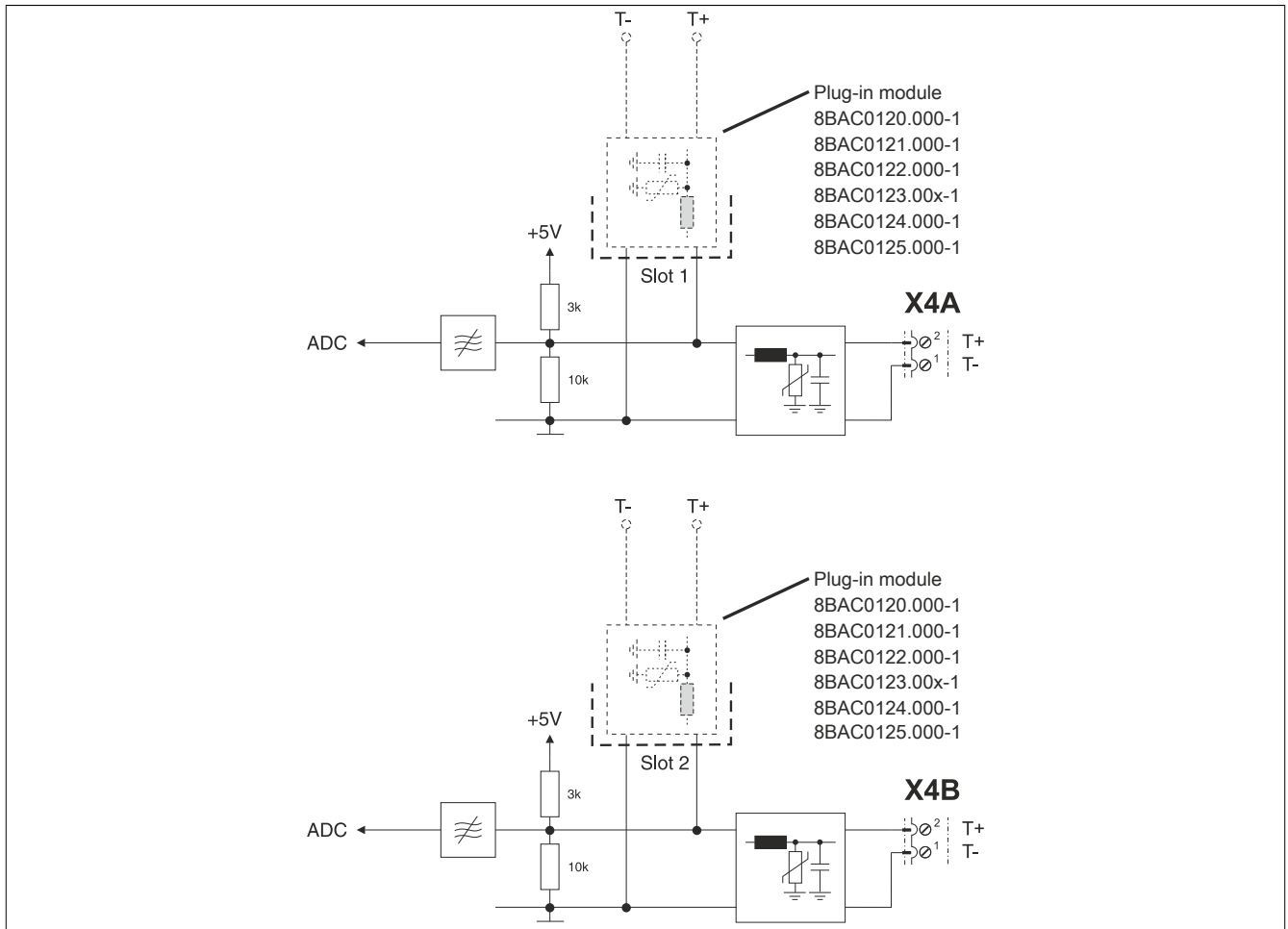
Figure 8: Temperature sensor
