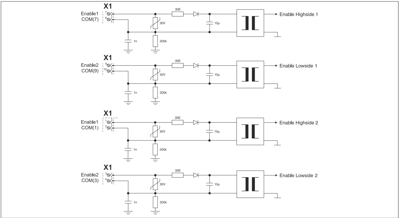
Figure 4: Enable
