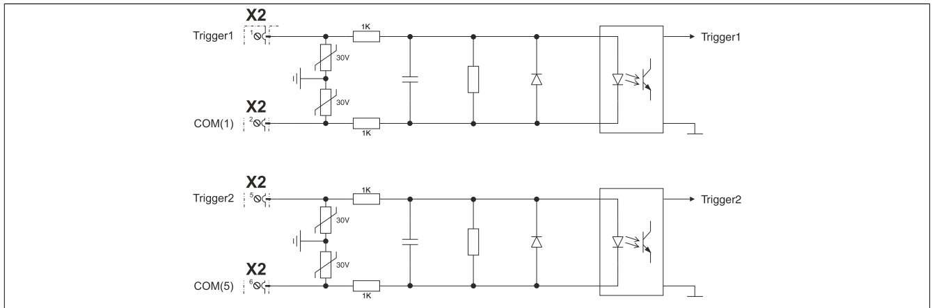
Figure 5: Trigger inputs
