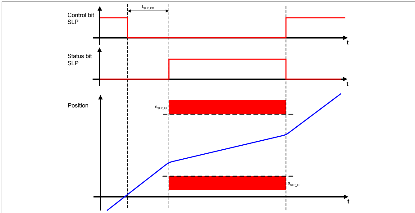
Figure 88: Safety Limited Position (SLP)
