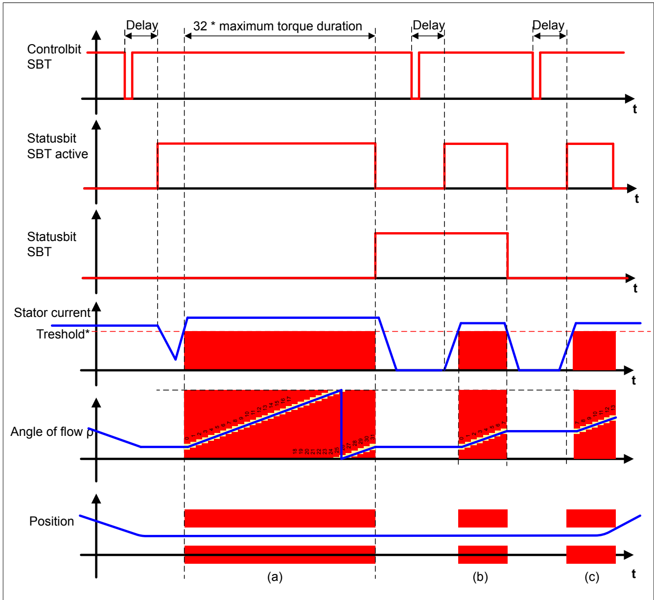
Figure 90: Safe Brake Test (SBT)
