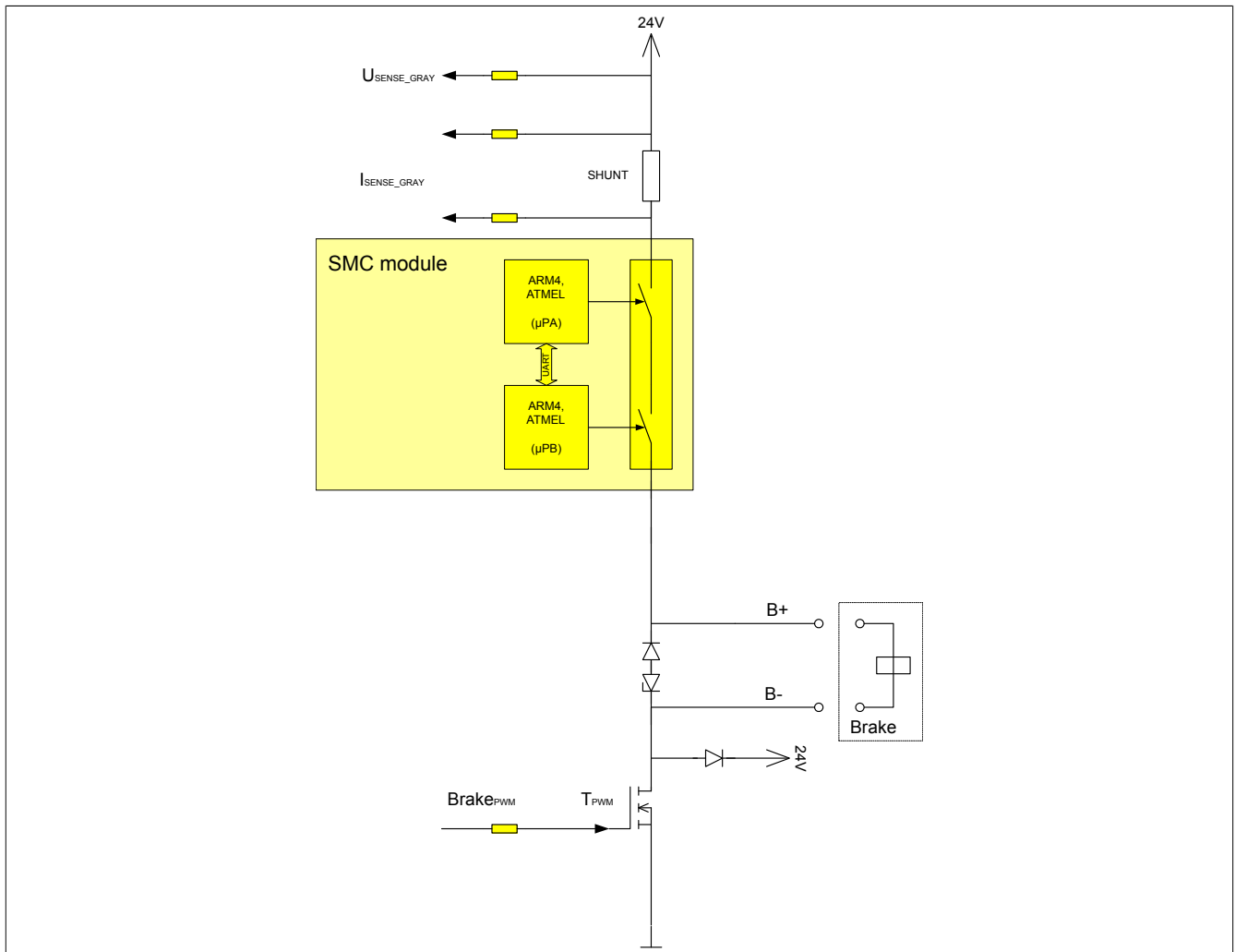
Figure 64: Connection of safe motor holding brake output
