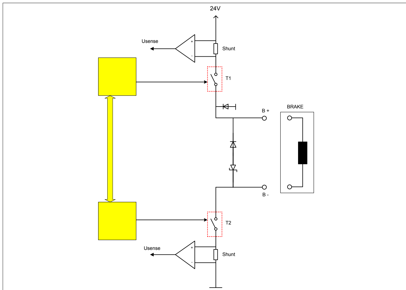
Figure 65: Connection of safe motor holding brake output
