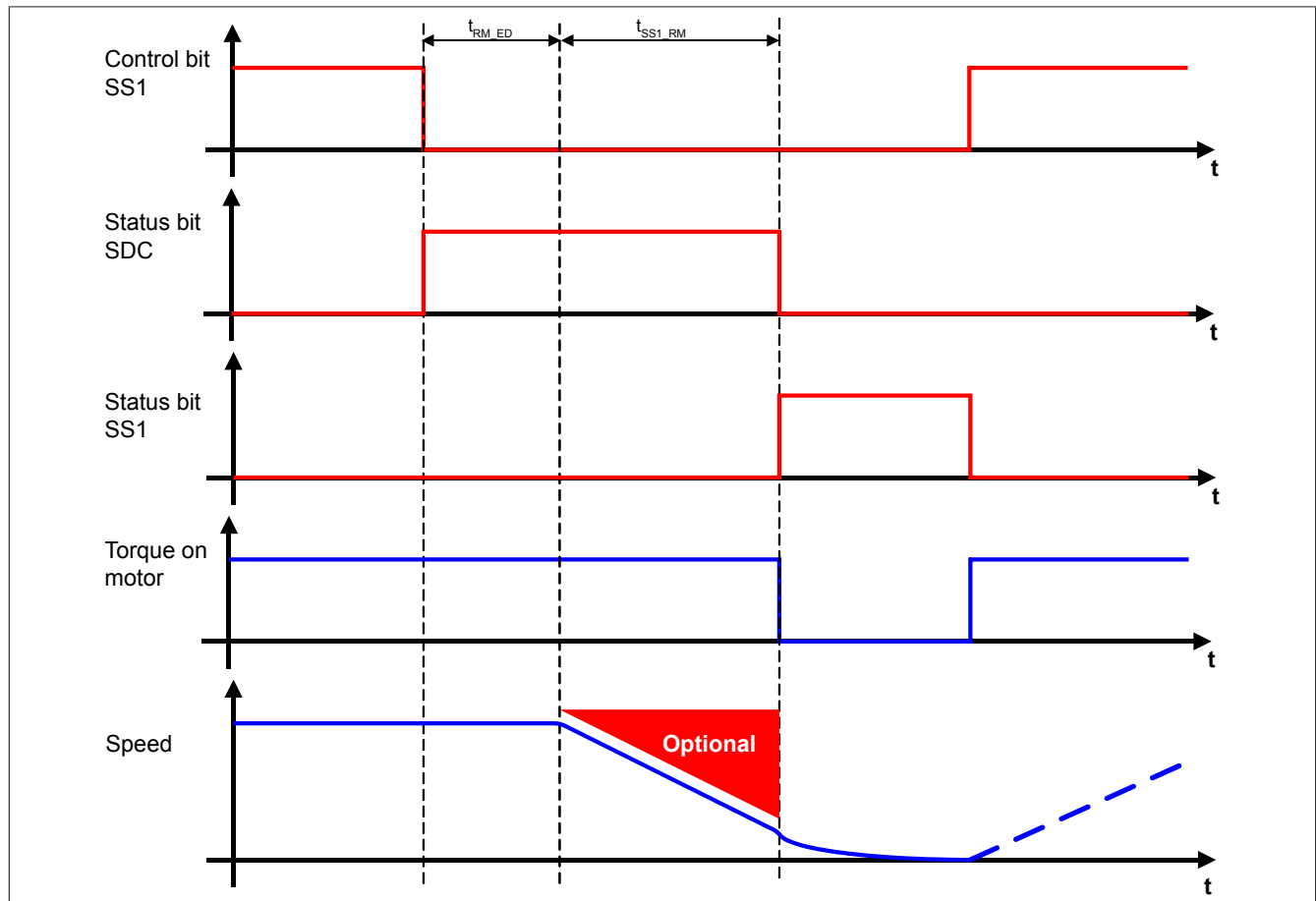
Figure 75: Safe Stop 1 (SS1)
