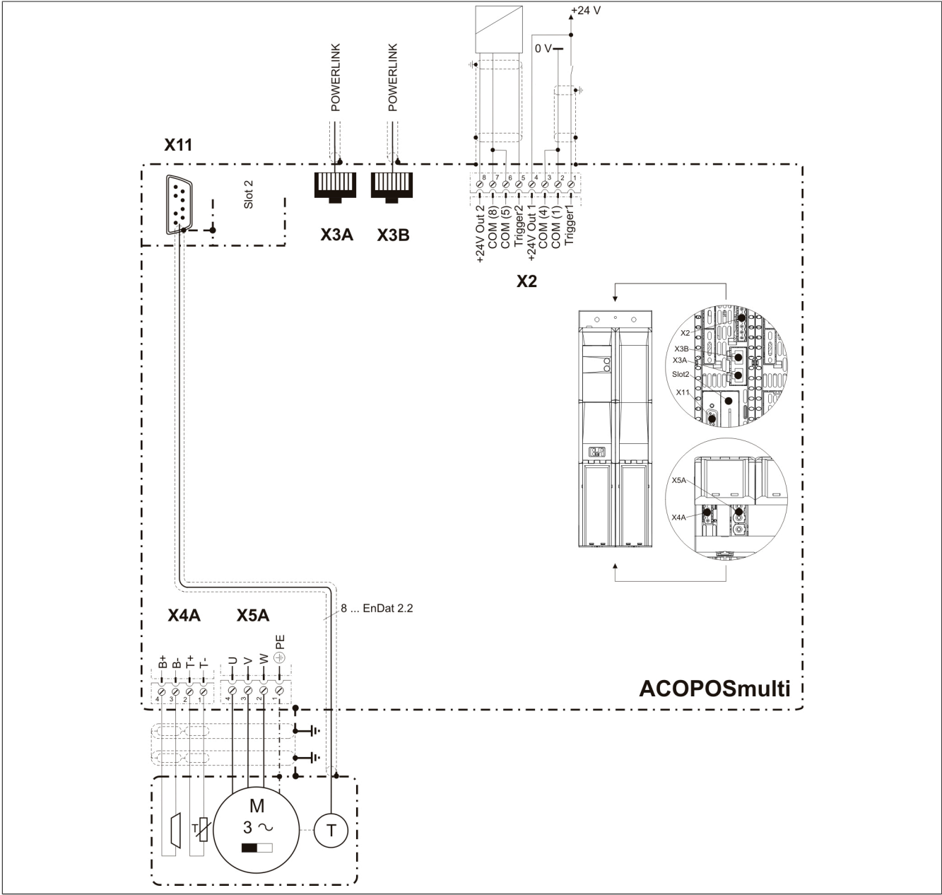
Figure 11: Pinout overview
