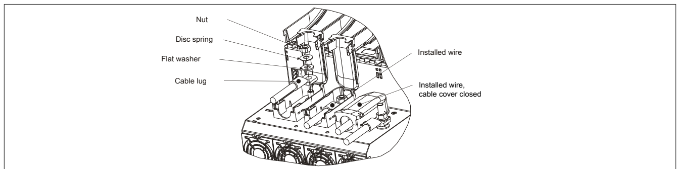
Figure 14: X5A - Cable installation
