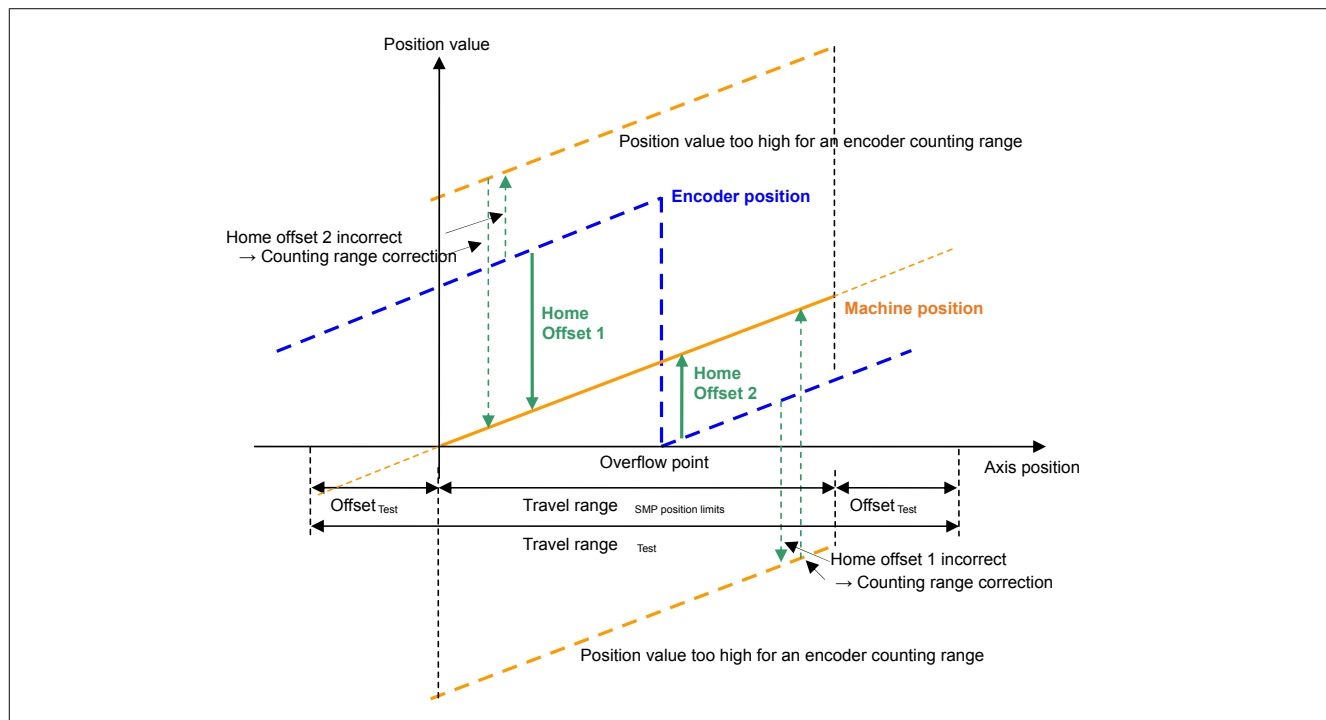
Figure 85: Homing method "Home offset with correction"
