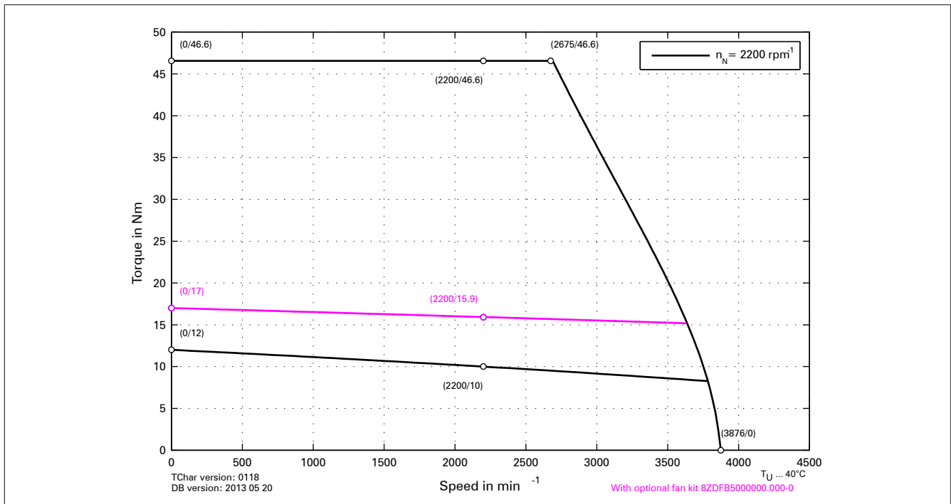
Figure 45: 8DI56e.fggghi00-1 - Speed-torque characteristic curve
