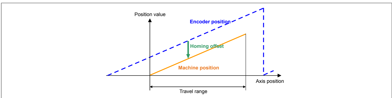
Figure 84: Homing mode - Home offset
