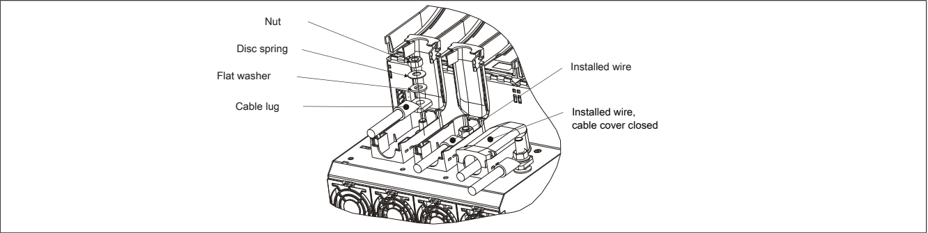
Figure 16: X5A - Cable installation
