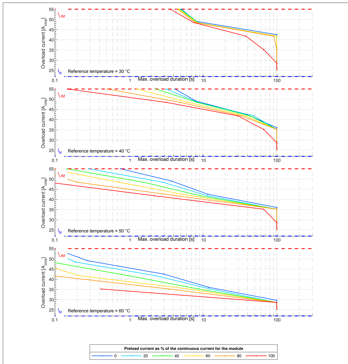
Figure 1: 8BVI0220HCDx.000-1 - Overload characteristics, overload response - WARNING
