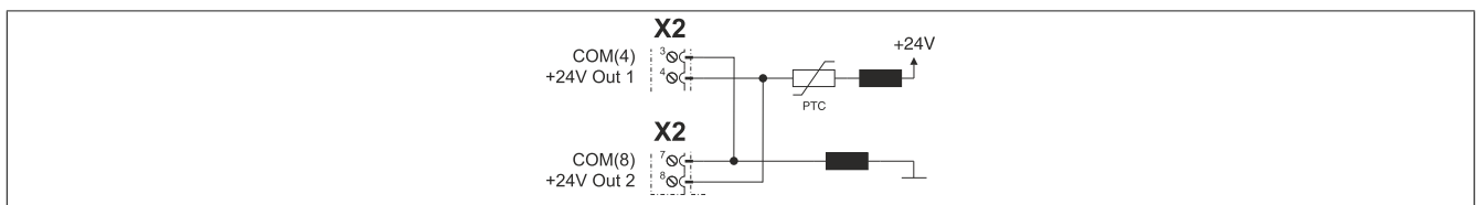
Figure 9: 24 VDC out
