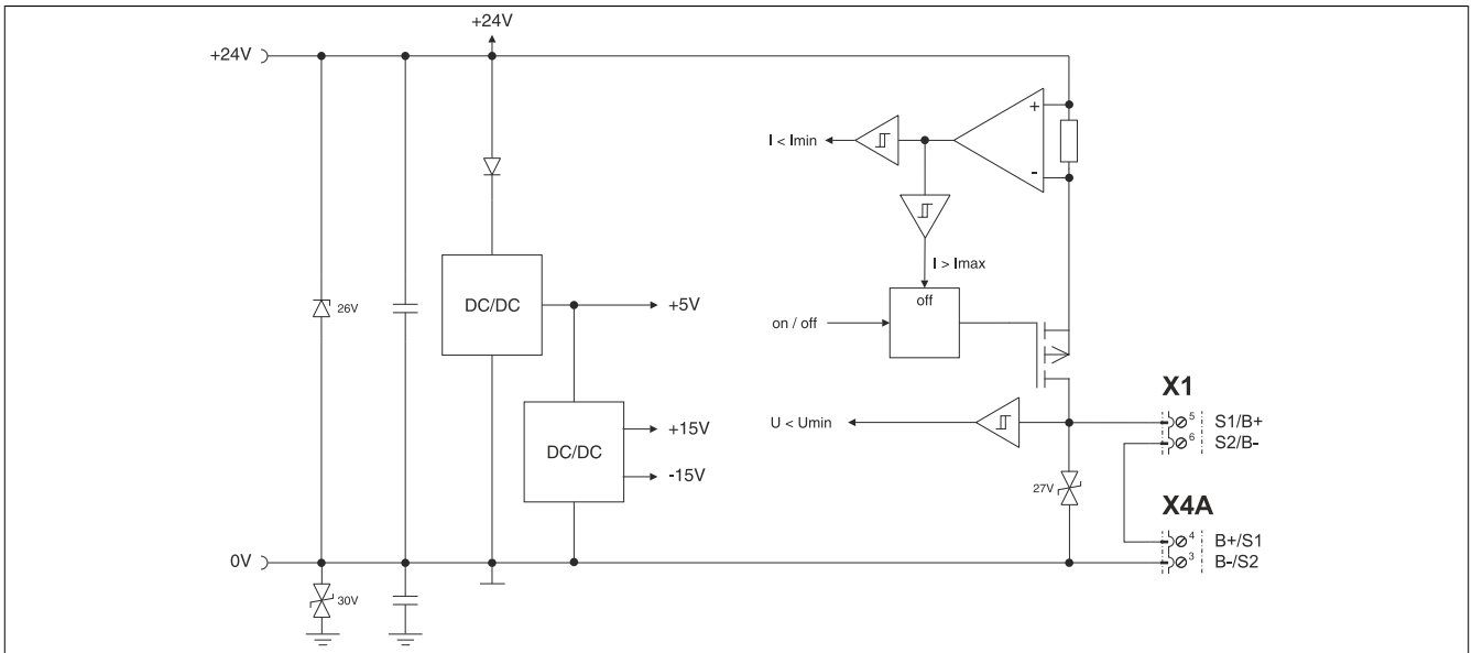
Figure 10: Holding brake
