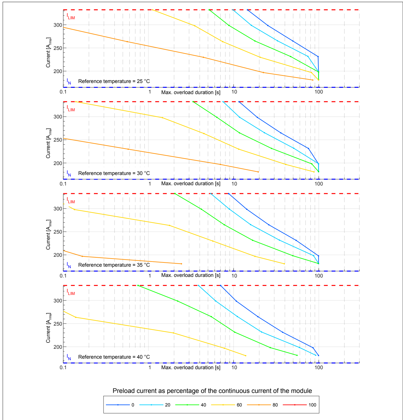
Figure 1: Overload characteristics of 8BVI1650HWSx.000-1, overload response - WARNING
