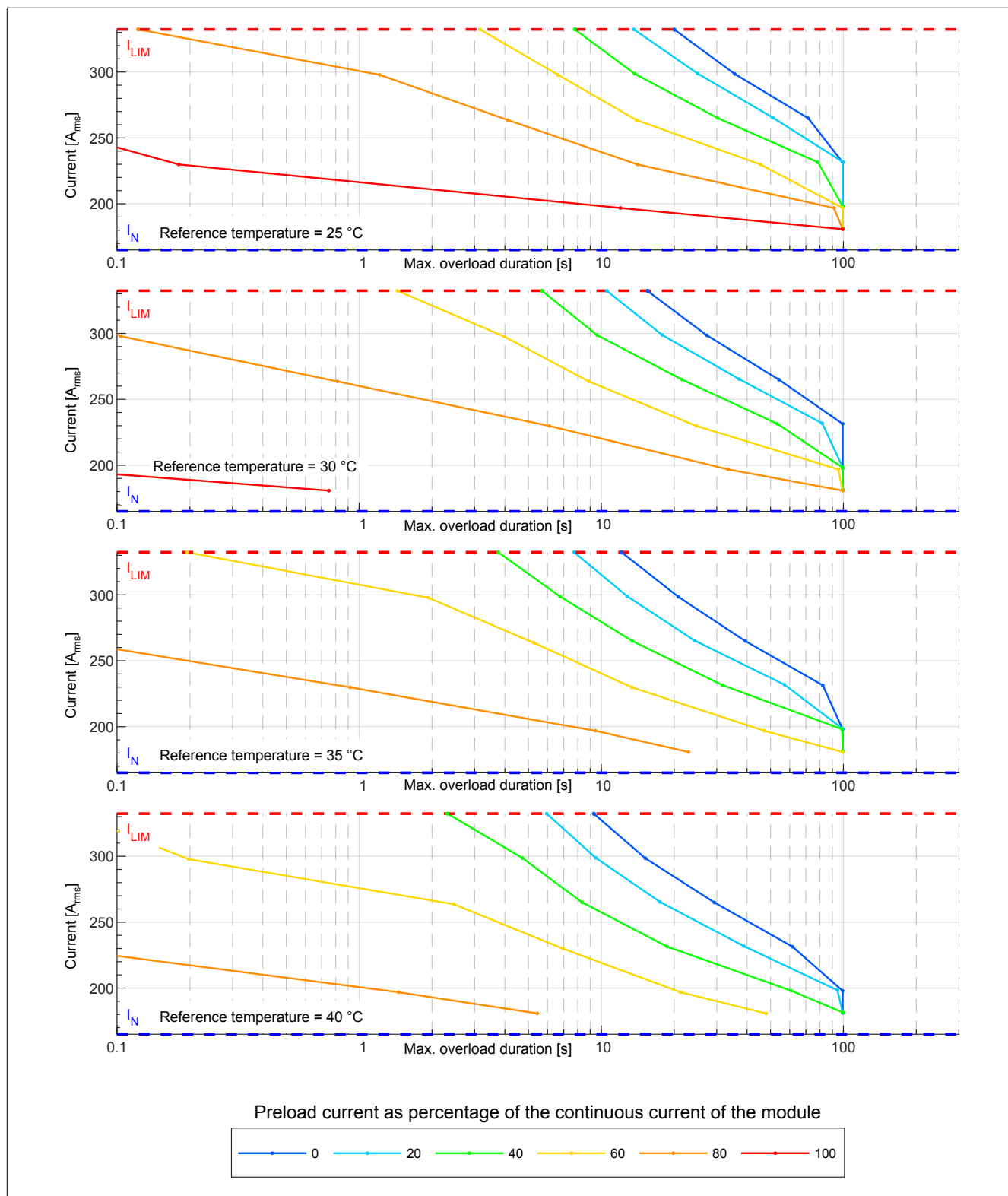
Figure 2: 8BVI1650HWSx.000-1 - Overload characteristics, overload response ERROR+STOP
