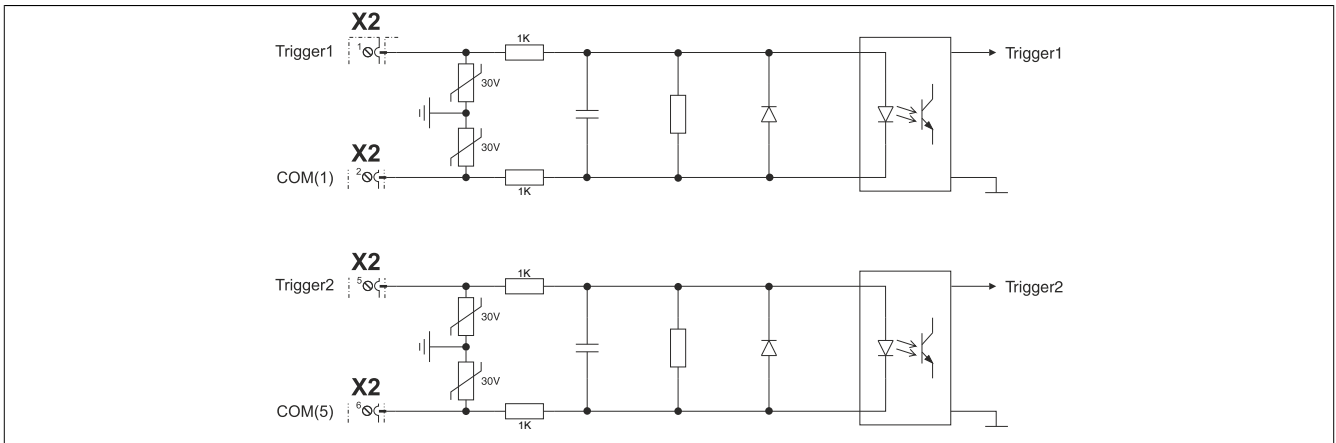
Figure 5: Trigger inputs
