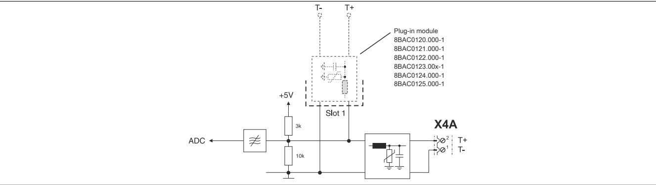
Figure 10: Temperature sensor
