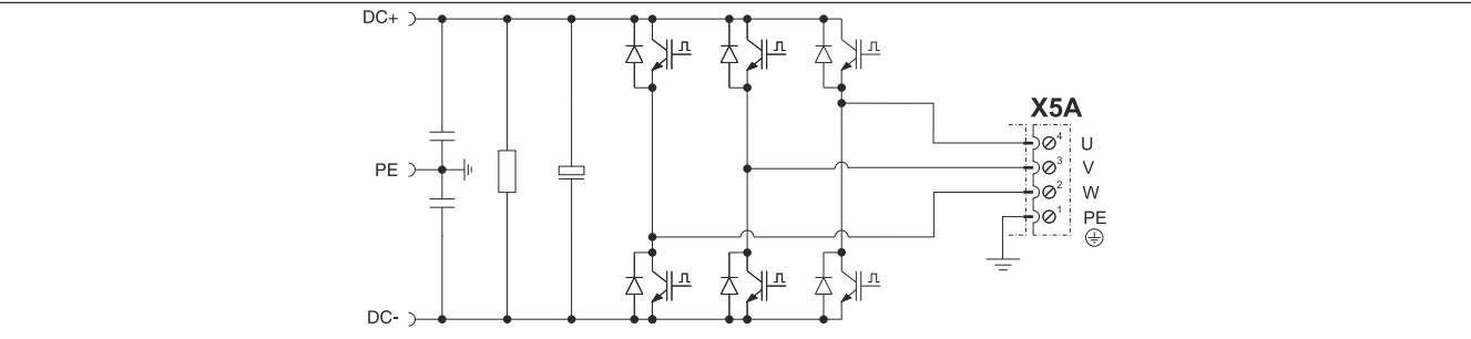
Figure 11: Motor
