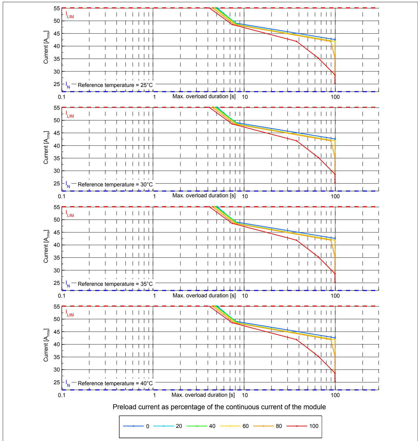
Figure 1: Overload characteristic 8BVI0220HWSx.000-1, Overload response - WARNING
