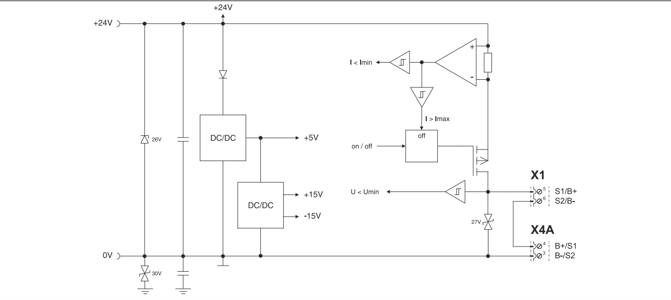
Figure 9: Holding brake
