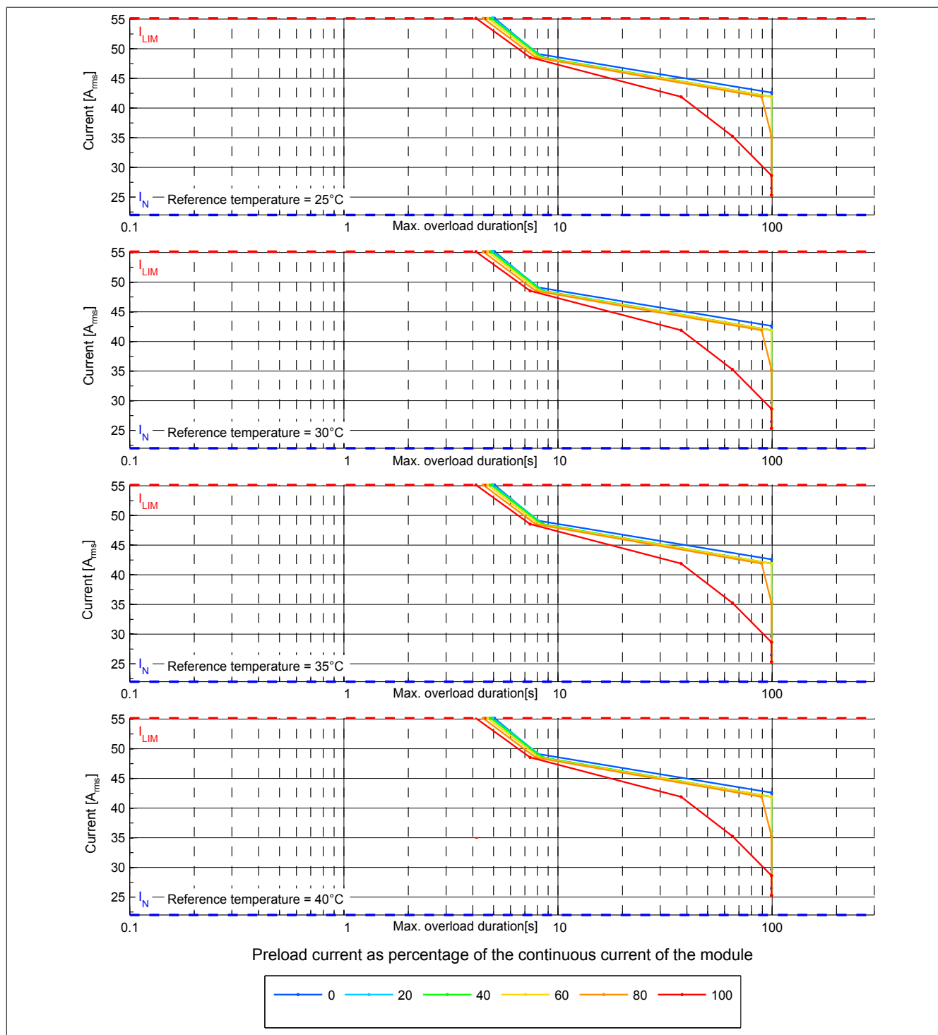
Figure 2: Overload characteristic 8BVI0220HWSx.000-1, Overload response - ERROR+STOP
