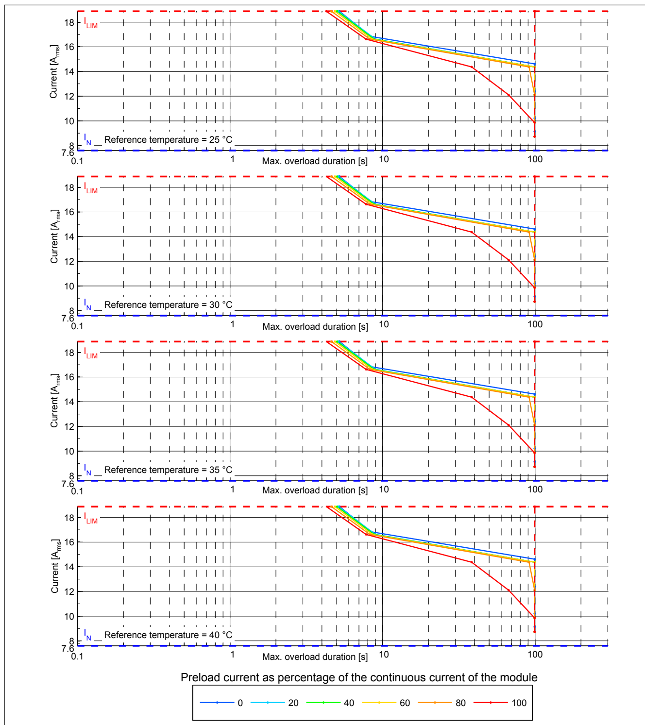
Figure 2: 8BVI0055HWSx.000-1 - Overload characteristics, overload response - ERROR+STOP
