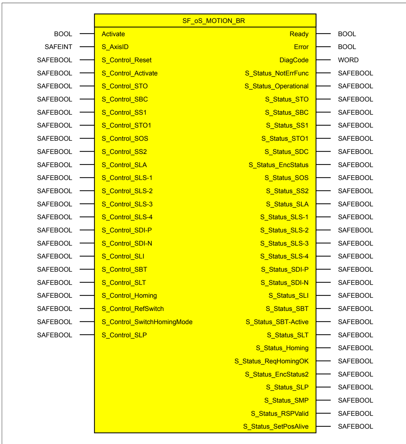
Figure 116: Function block "SF_oS_MOTION_BR"
