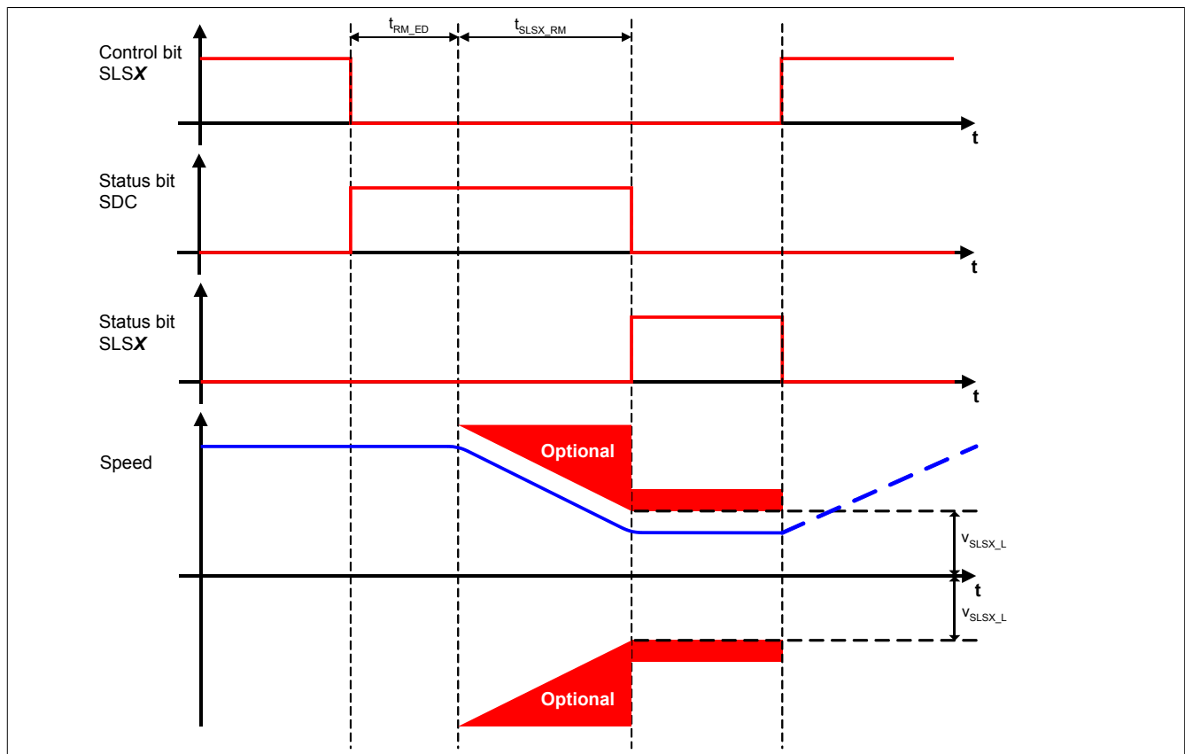
Figure 74: Safely Limited Speed (SLS)
