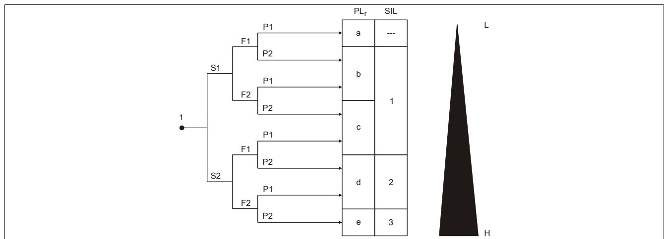
Figure 119: Risk diagram for determining the PL r for each safety function per EN ISO 13849-1, appendix A
