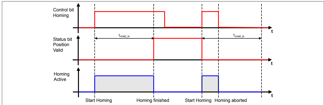
Figure 79: Safe Homing
