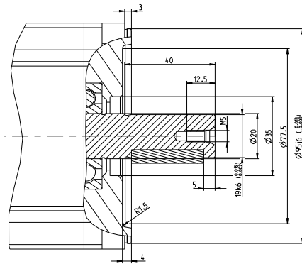
Figure 50: Flange details
