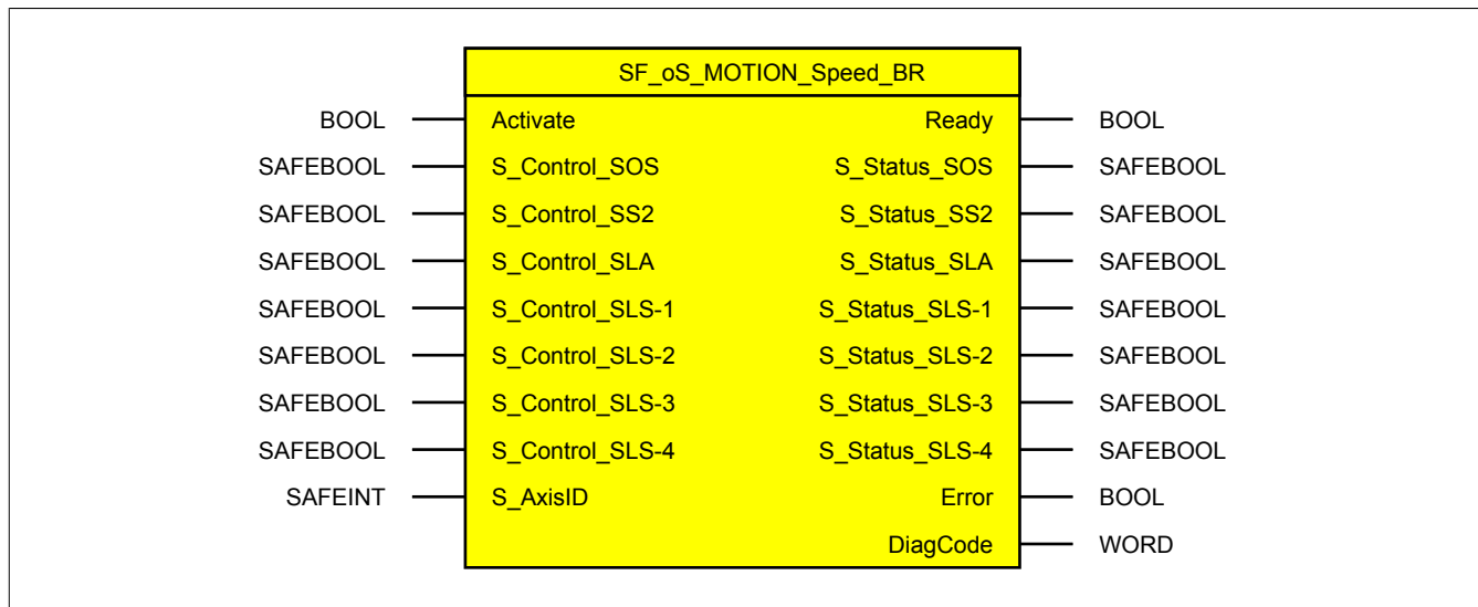
Figure 113: Function block SF_oS_MOTION_Speed_BR
