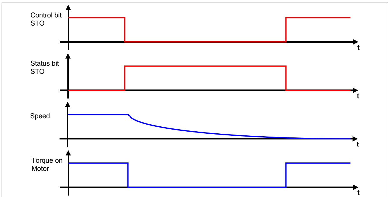
Figure 69: Safe Torque Off (STO)
