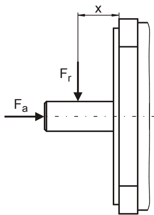
Figure 29: Definition of shaft load
