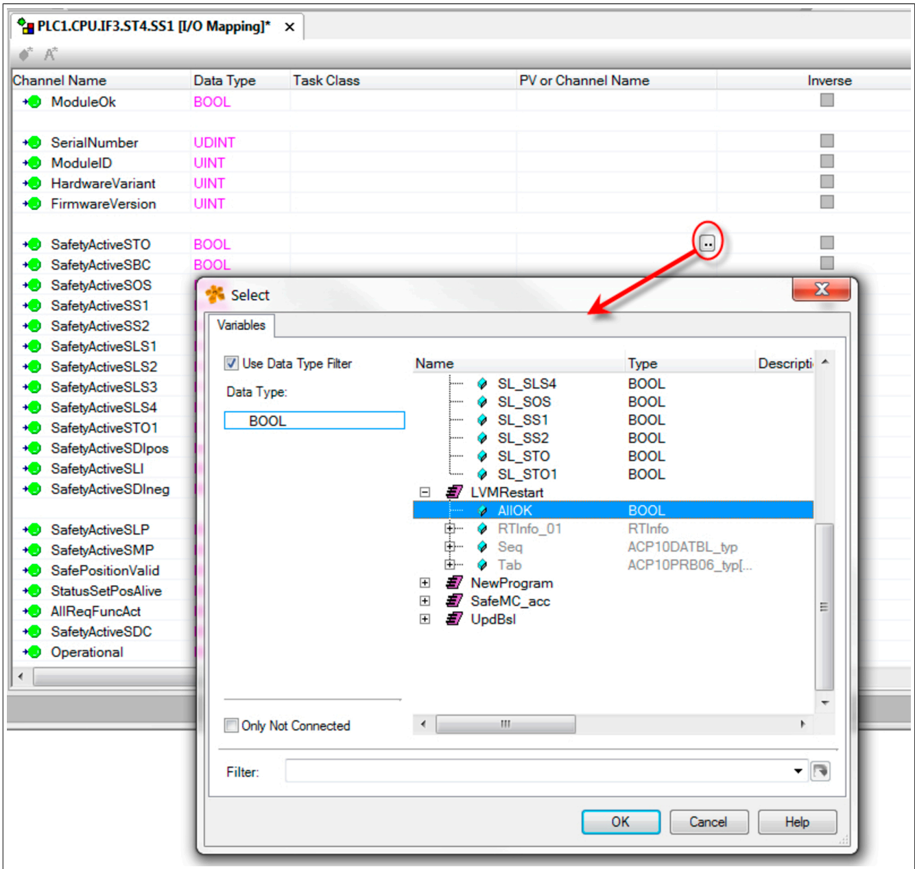
Figure 95: PV mapping
