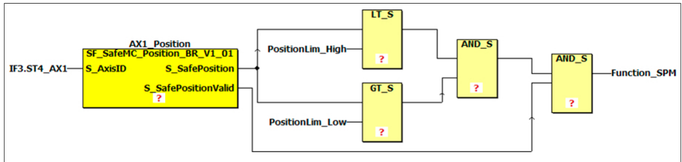
Figure 107: SF_SafeMC_Position_BR: The Safe Position Monitor function
