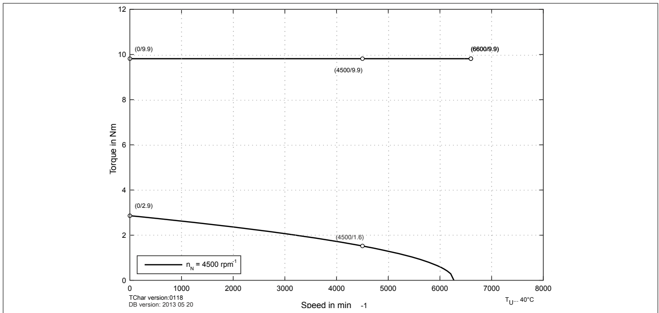
Figure 34: 8DI34e.fggghi00-1 with 750 VDC DC bus voltage - Speed-torque characteristic curve
