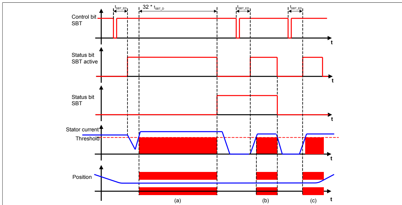
Figure 87: Safe Brake Test (SBT)
