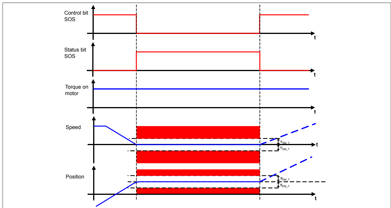
Figure 71: Safe Operating Stop (SOS)
