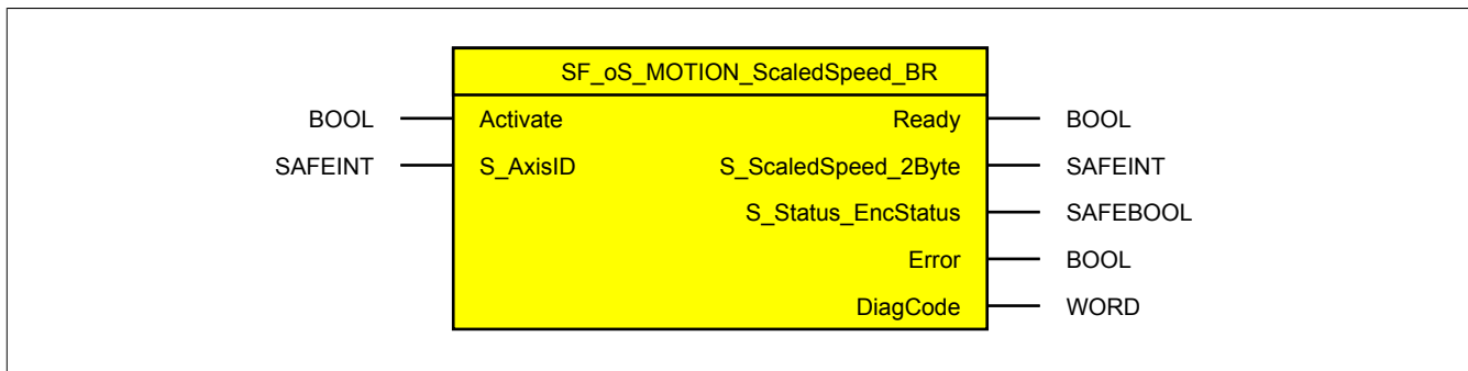
Figure 117: Function block SF_oS_MOTION_ScaledSpeed_BR
