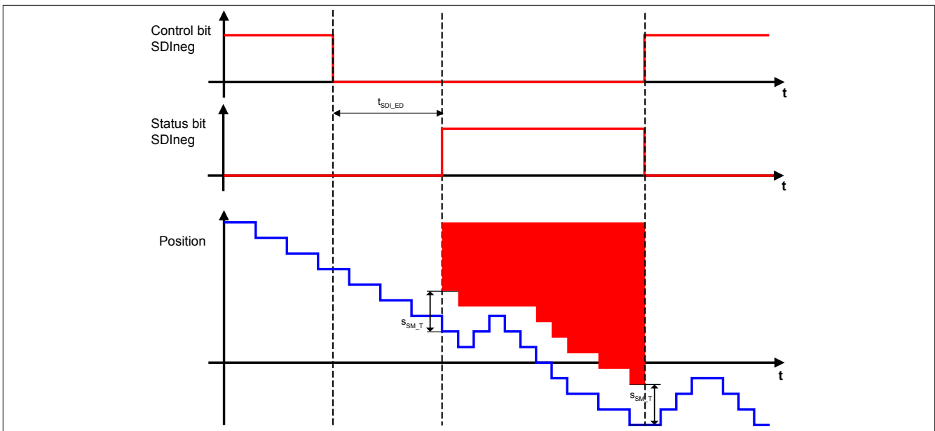
Figure 77: Safe Direction (SDI) - Negative direction of rotation allowed
