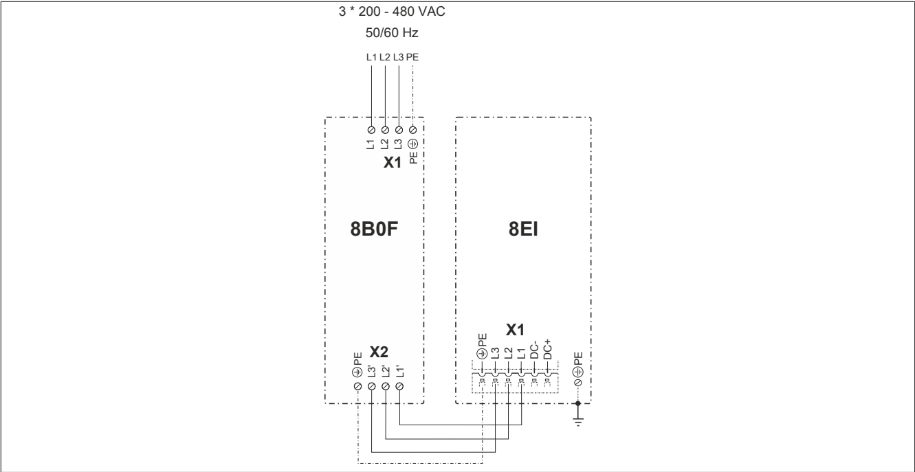
Figure 54: Mains connection 3x 200 - 480 VAC
