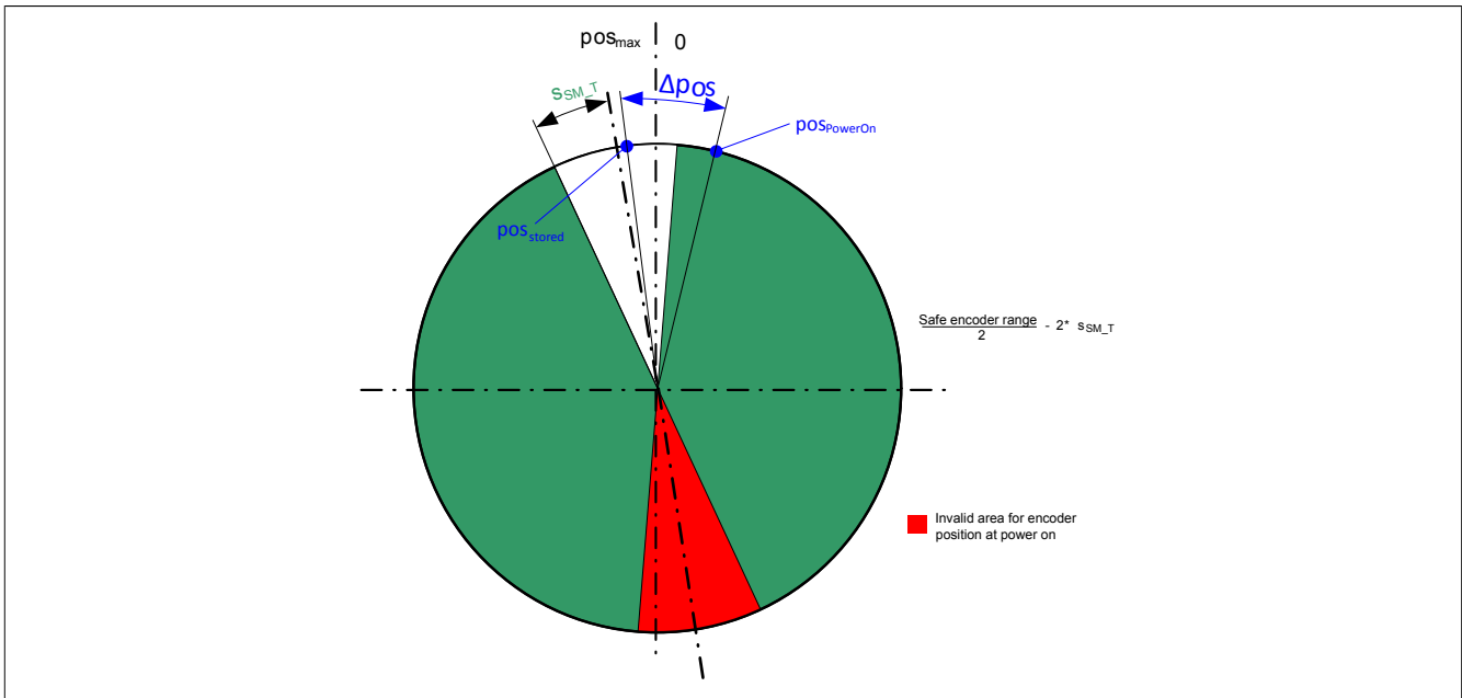
Figure 84: RSP safety function with respect to position for one revolution
