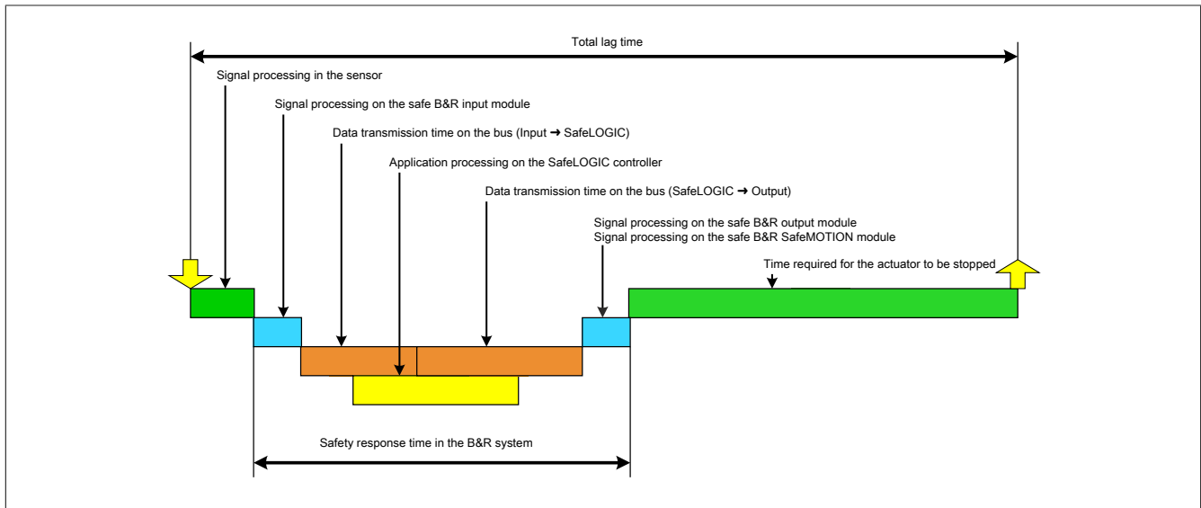
Figure 56: Total lag time
