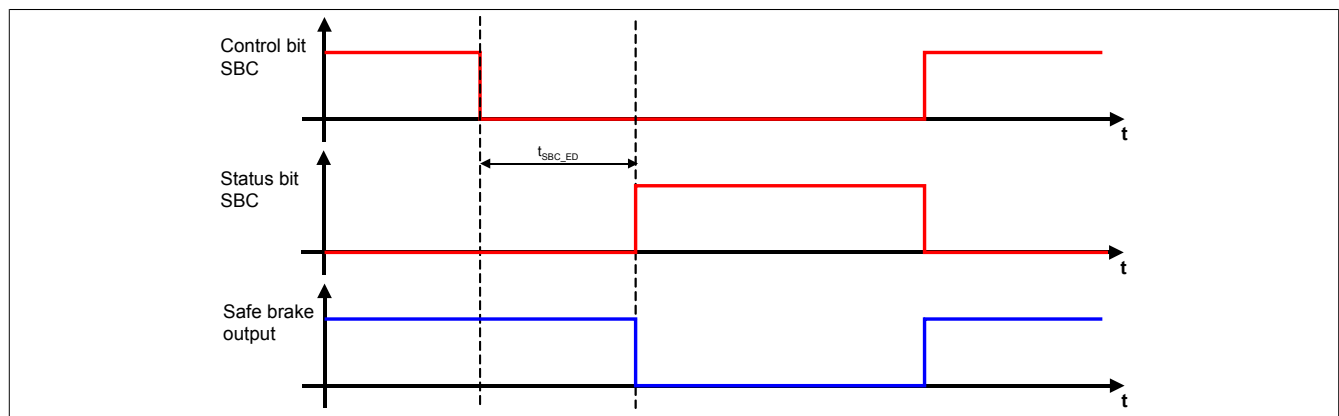
Figure 70: Safe Brake Control (SBC)
