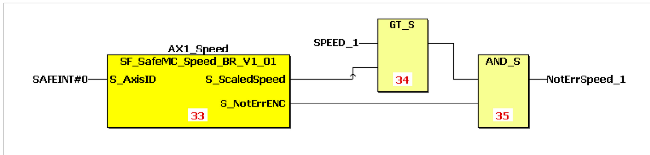
Figure 105: SF_SafeMC_Speed_BR: Evaluation of the scaled safe speed
