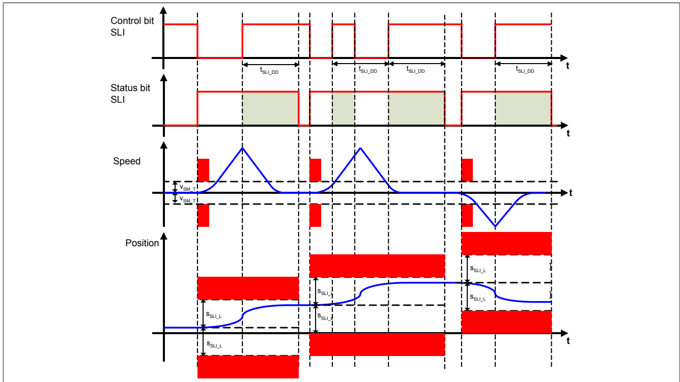
Figure 75: Safely Limited Increment (SLI)
