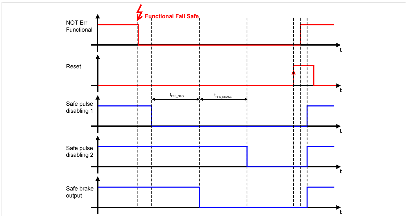
Figure 68: FUNCTIONAL FAIL SAFE - STO1 and STO configuration with time delay
