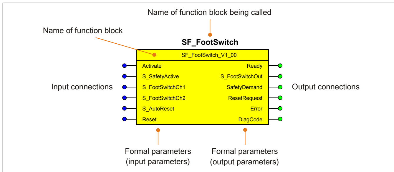
Figure 111: Function block label
