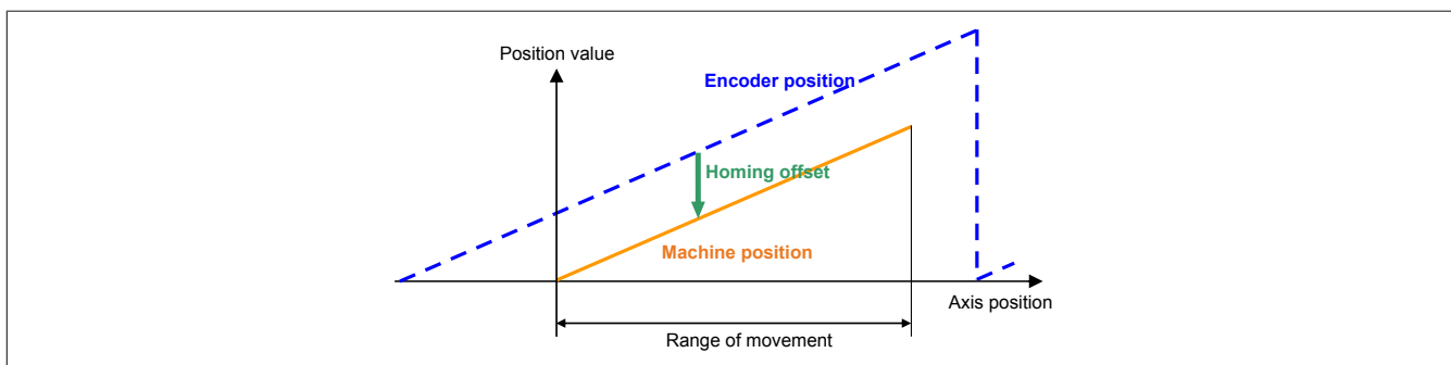
Figure 81: Homing mode - Home offset
