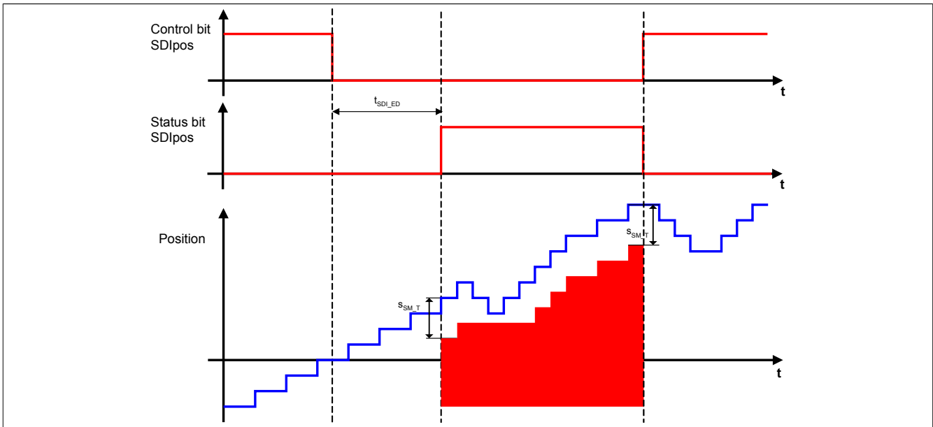
Figure 76: Safe Direction (SDI) - Positive direction of rotation allowed
