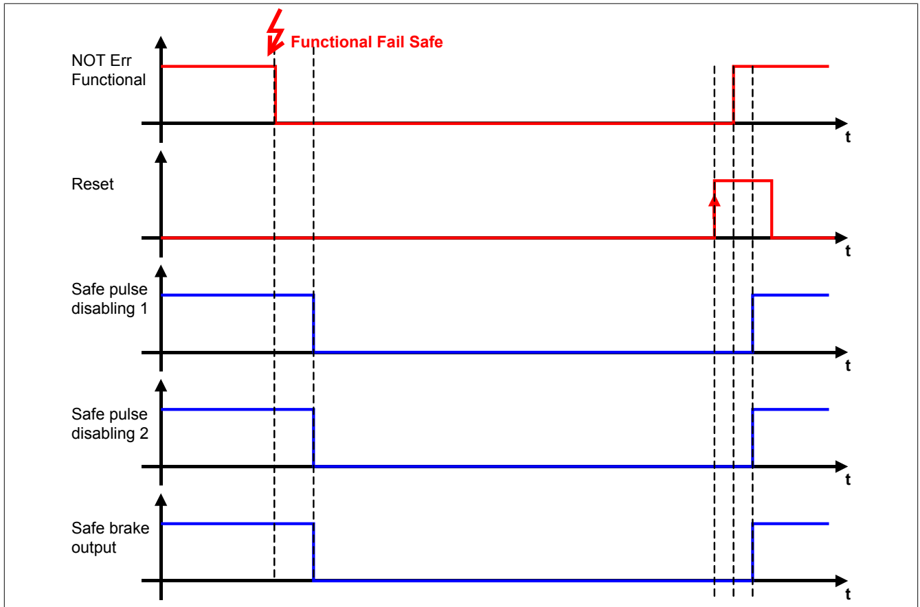
Figure 67: FUNCTIONAL FAIL SAFE - STO configuration
