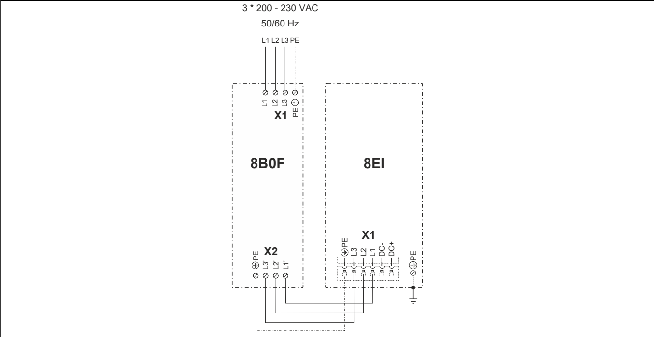
Figure 53: Mains connection 3x 200 - 230 VAC
