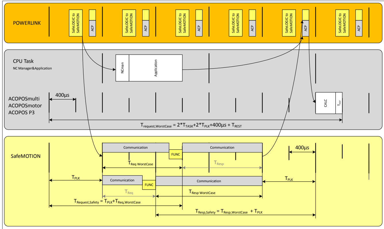
Figure 88: Inverter unit timing - SafeMOTION module
