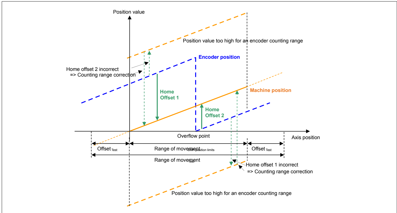
Figure 82: Homing mode - Home offset with correction
