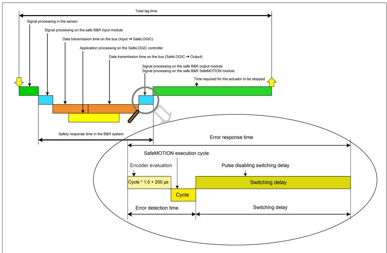
Figure 57: Safe error response time
