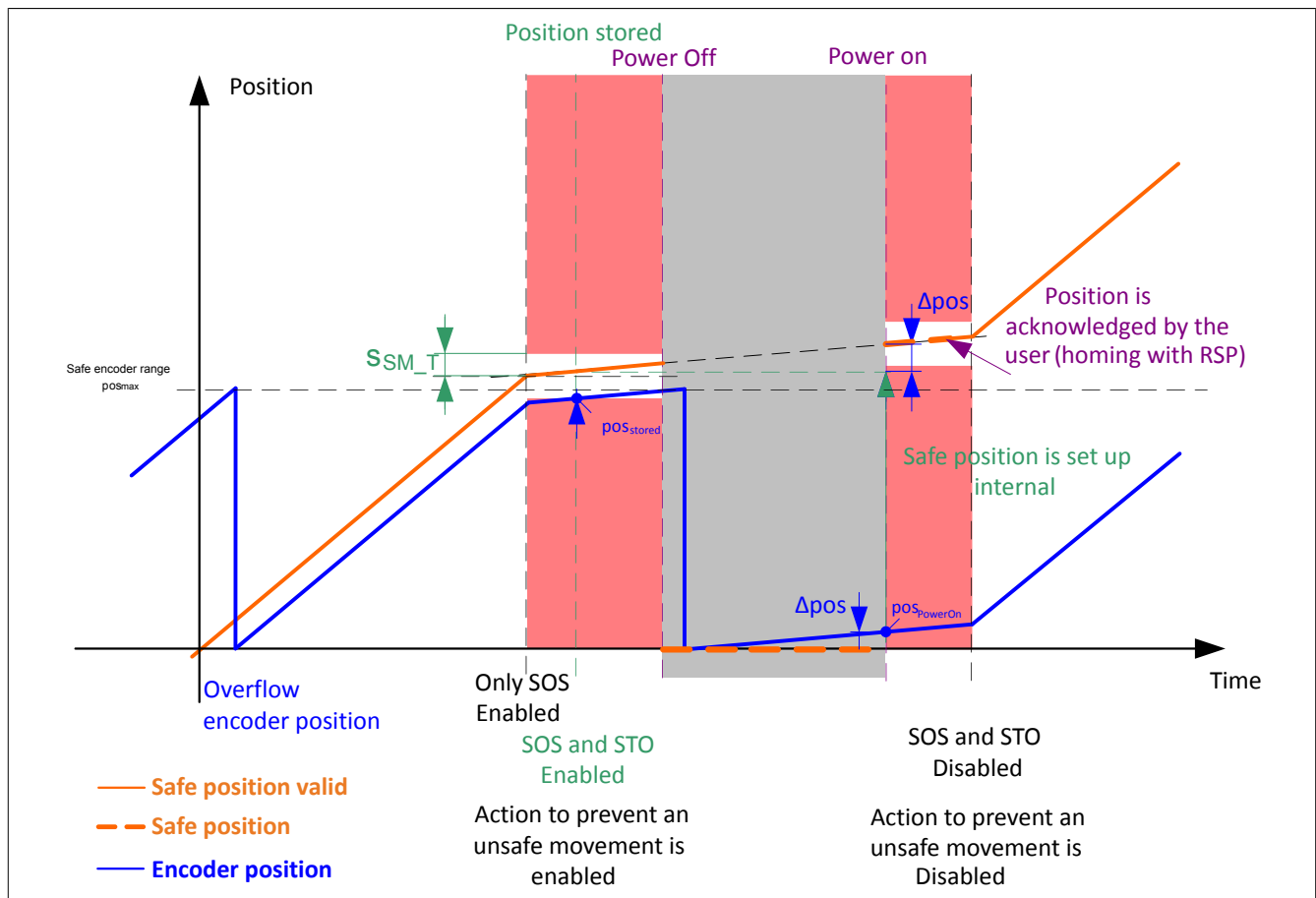
Figure 83: RSP safety function - Timing diagram with encoder overflow during power off
