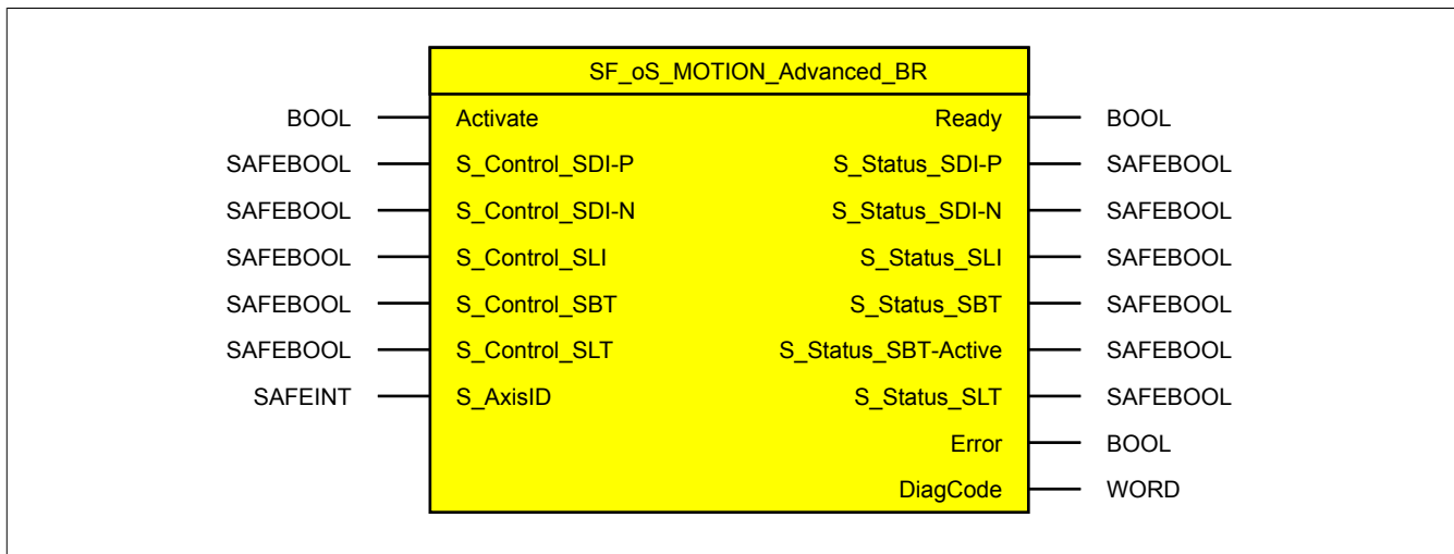
Figure 114: Function block SF_oS_MOTION_Advanced_BR
