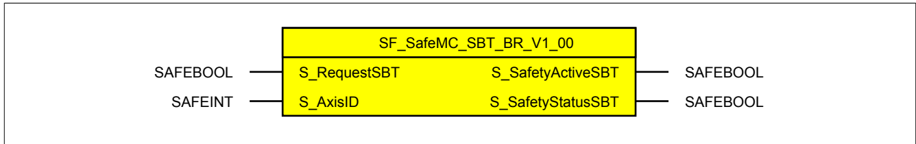
Figure 110: SF_SafeMC_SBT_BR function block
