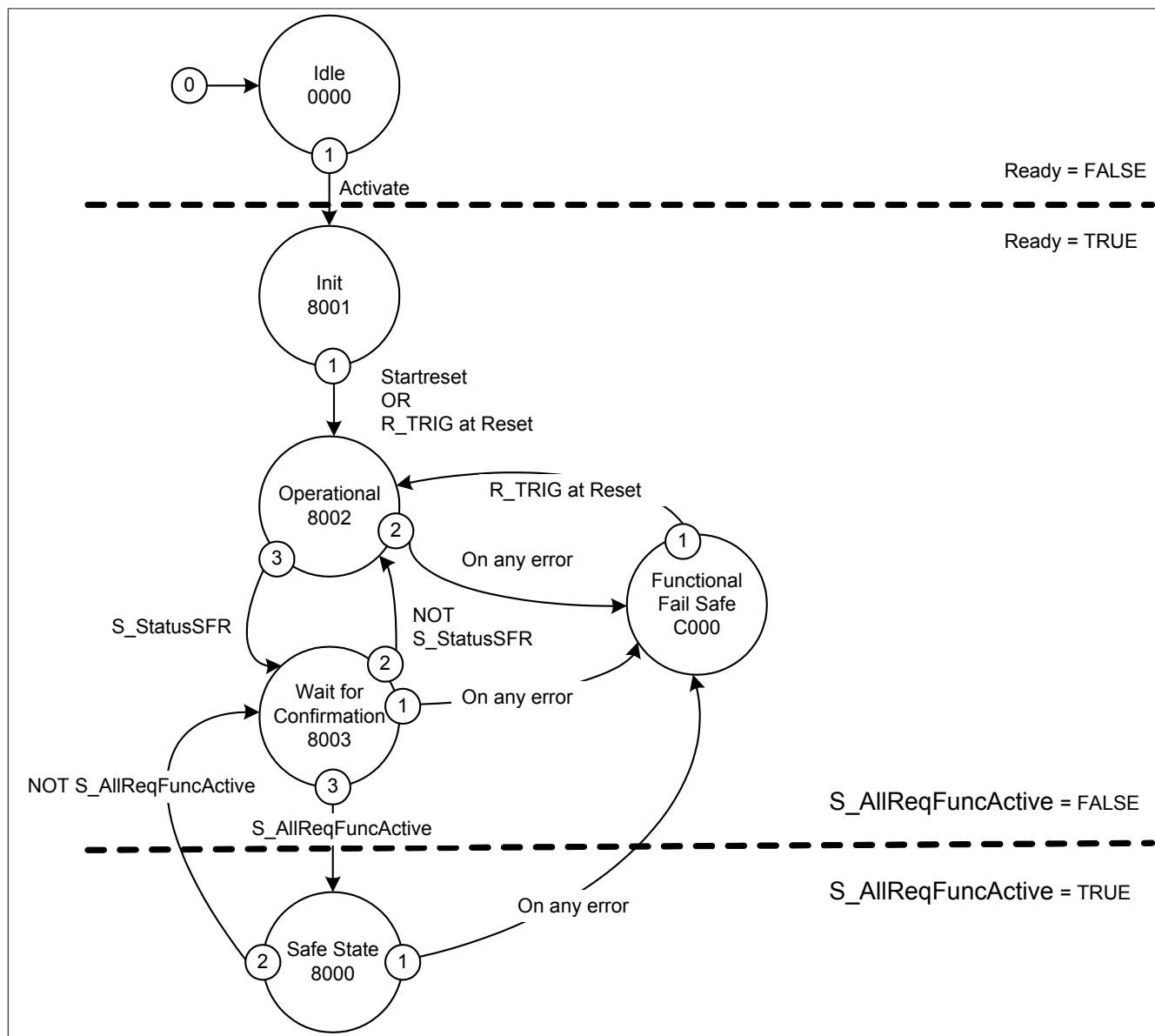
Figure 100: SF_SafeMC_BR(_V2, _V3): State machine
