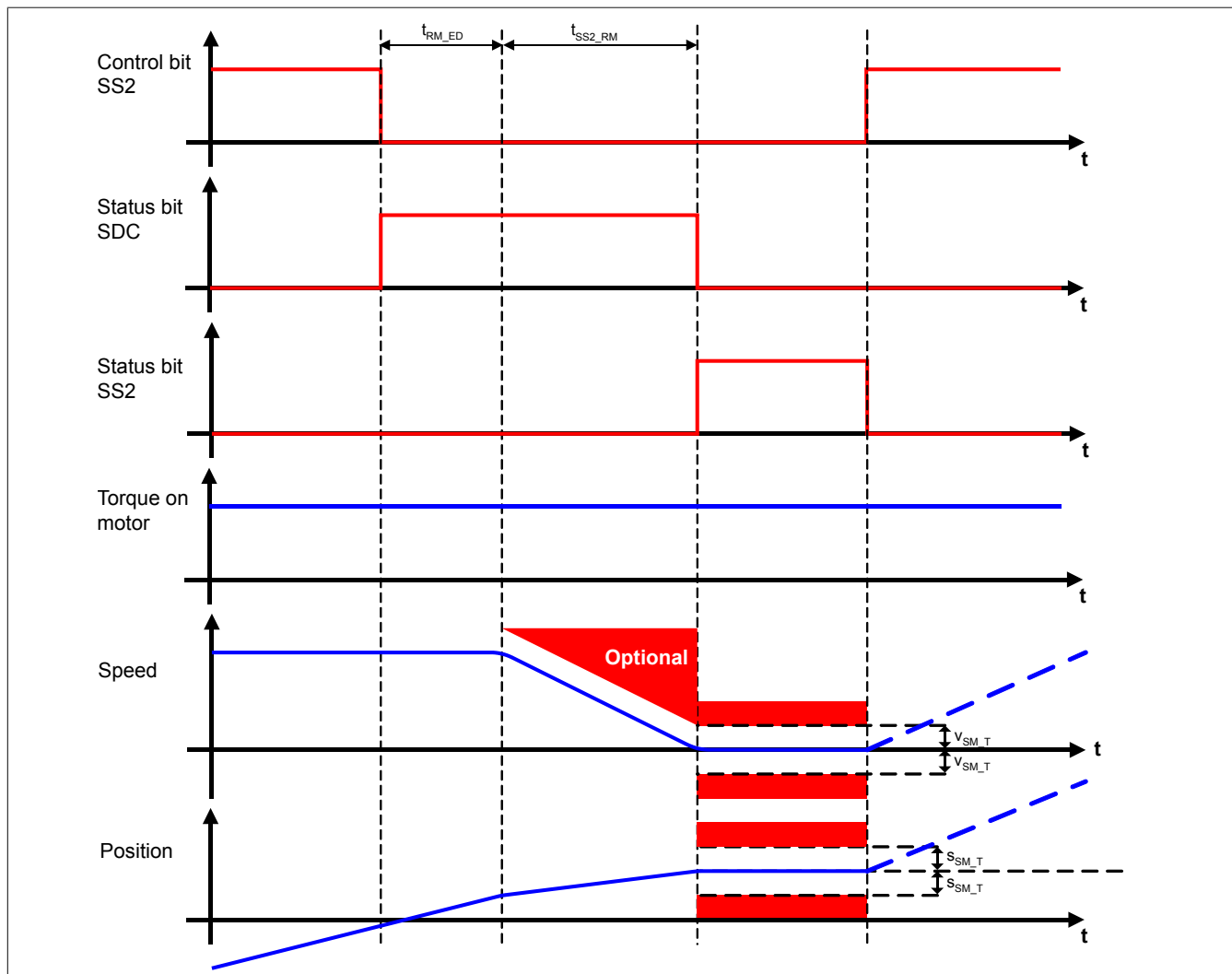
Figure 73: Safe Stop 2 (SS2)
