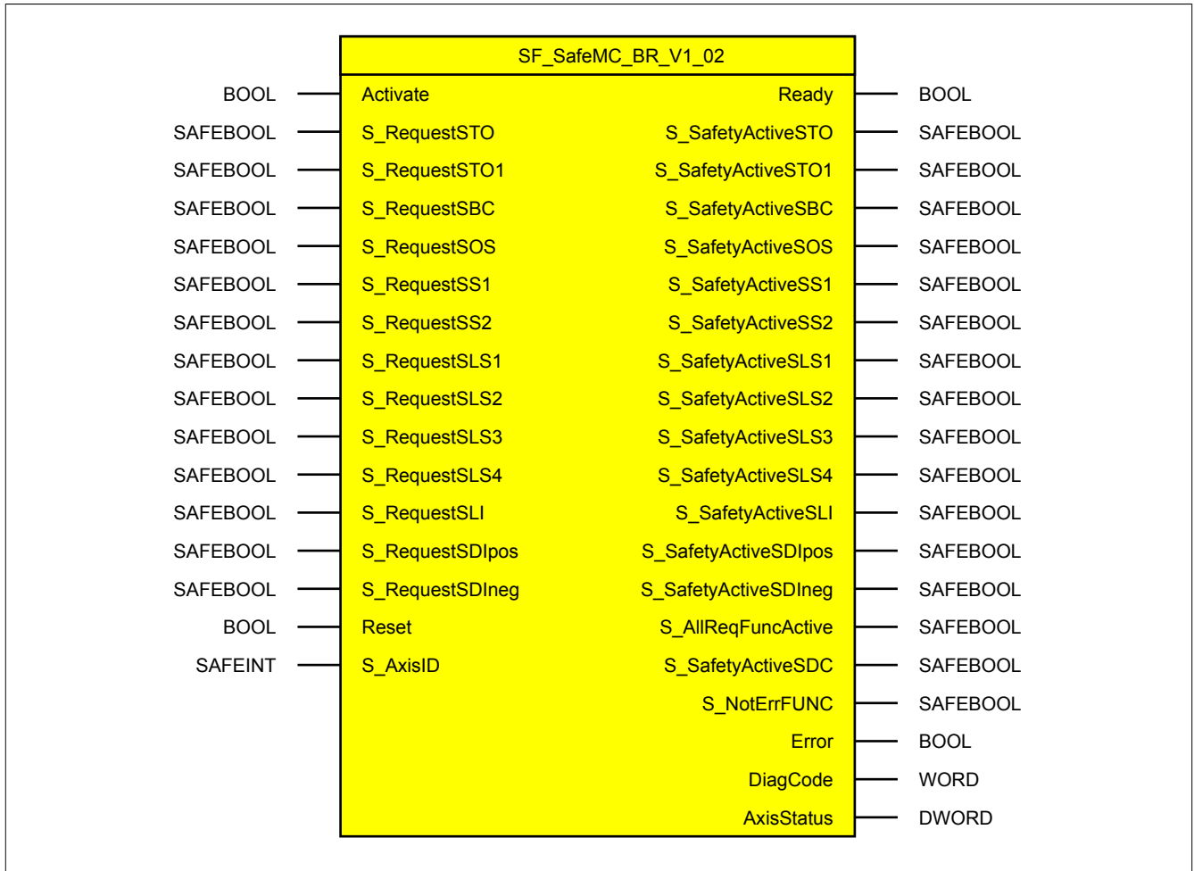
Figure 99: SF_SafeMC_BR function block
