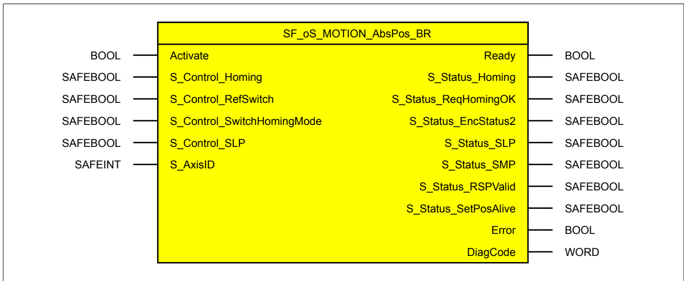
Figure 115: Function block SF_oS_MOTION_AbsPos_BR
