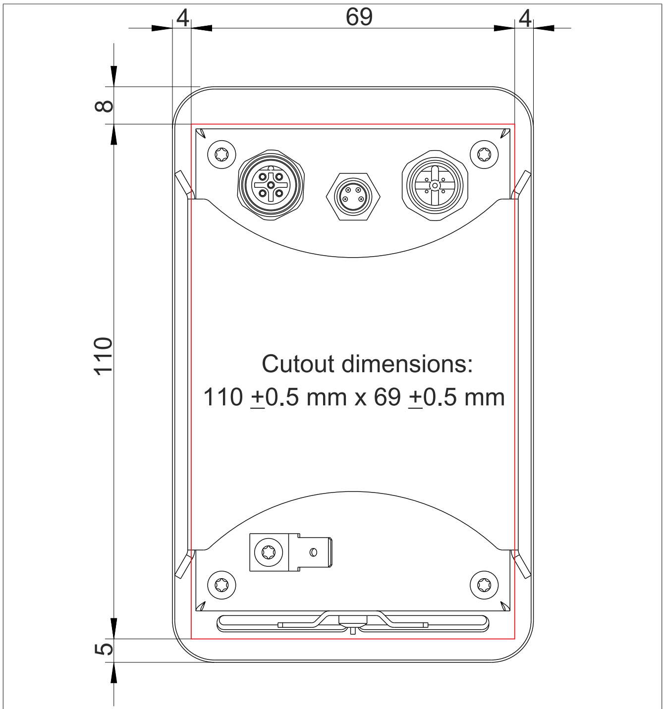
Figure 5: 4XP0000.00-K64 - Cutout installation
