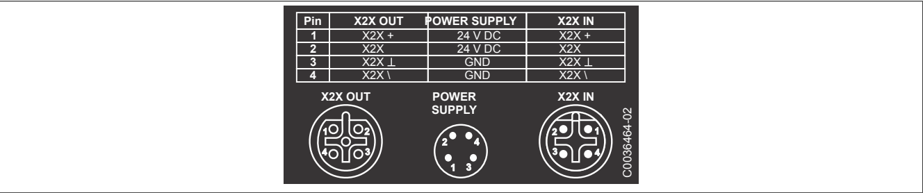
Figure 9: 4XP0000.00-K64 - Device label
