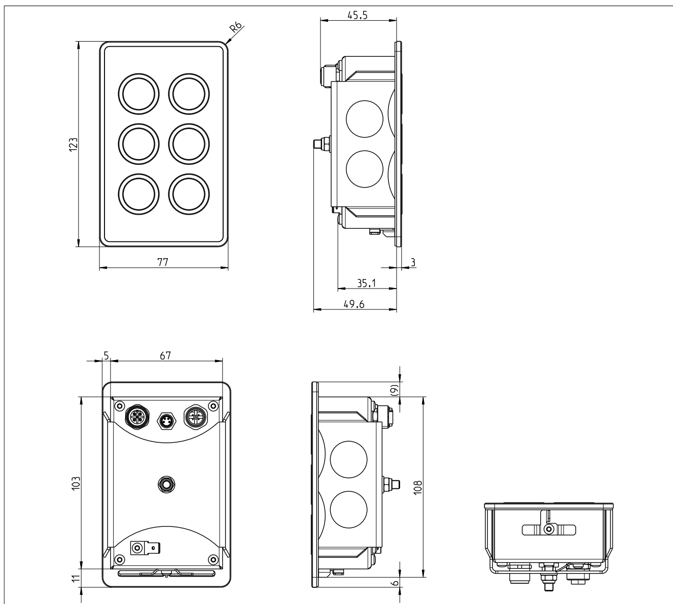
Figure 4: 4XP0000.00-K64 - Dimensions
