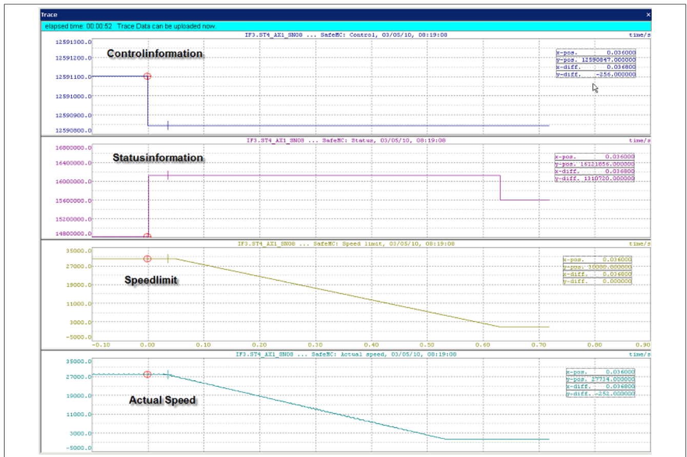
Figure 64: ACOPOSmulti Trace: Example with SafeMOTION data
