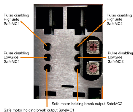
Figure 5: Dual-axis modules
