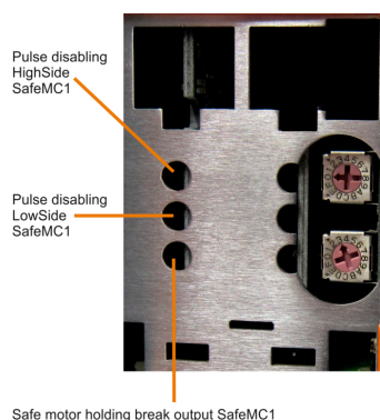
Figure 4: Single-axis modules
