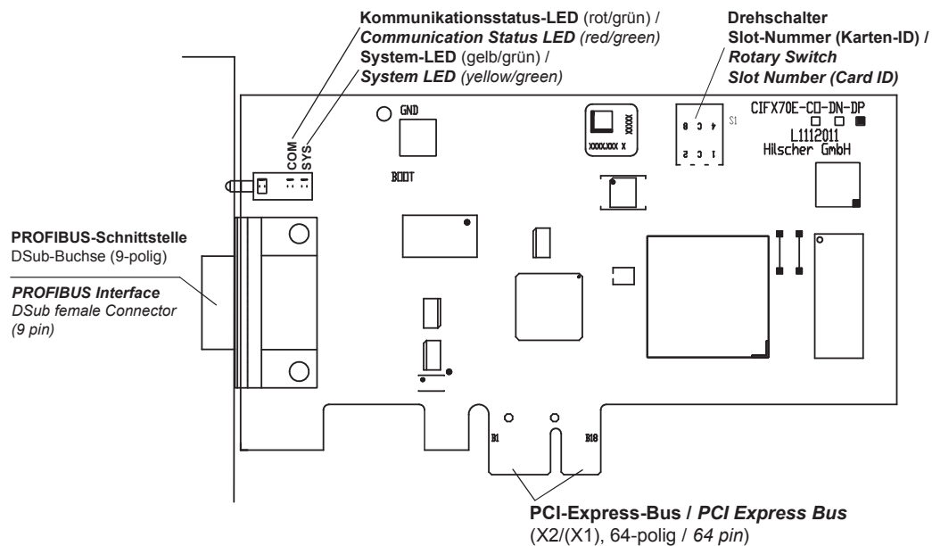
Figure 38: CIFS 70E-DP\MR (Hardware revision 1)
