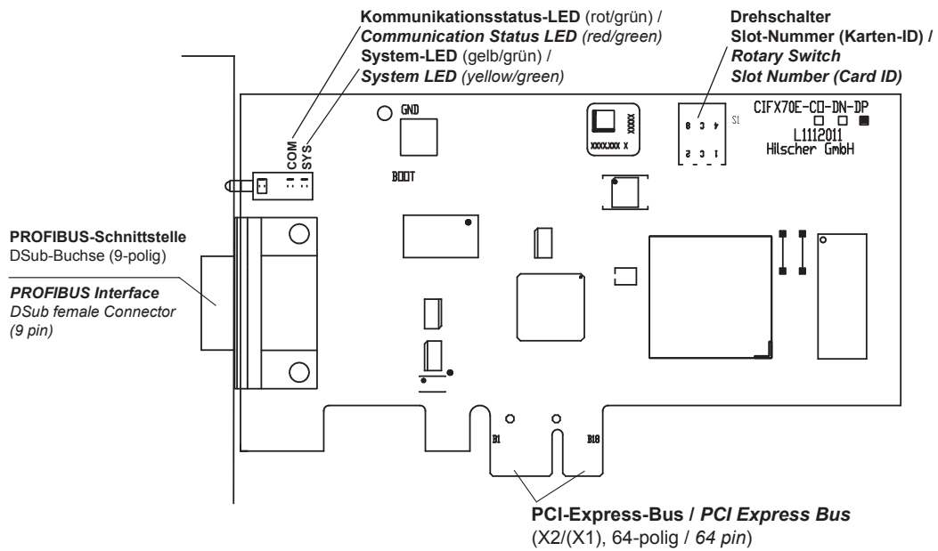
Figure 37: CIFS 70E-DP (Hardware revision 1)
