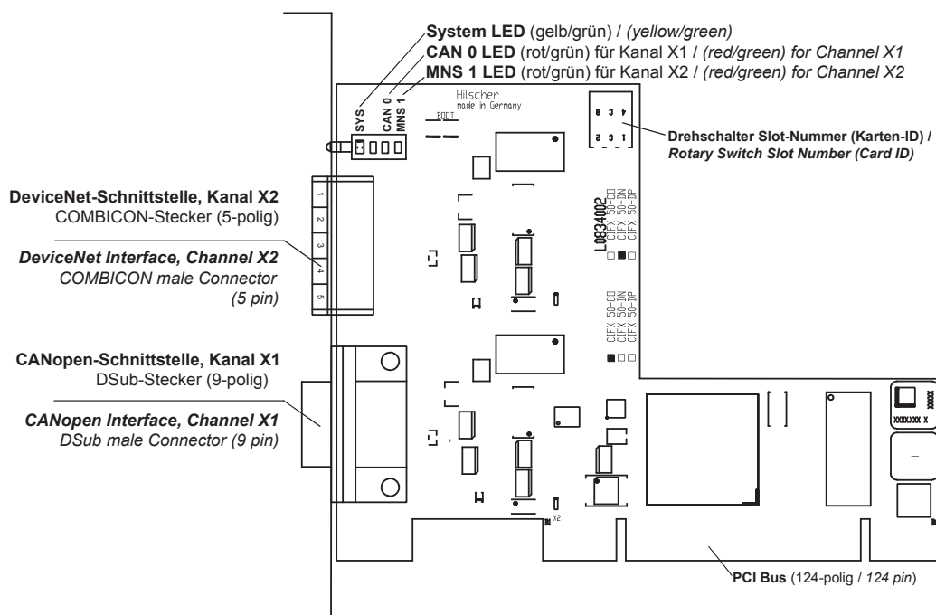
Figure 19: CIFX 50-2 CO\DN (Hardware Revision 1)
