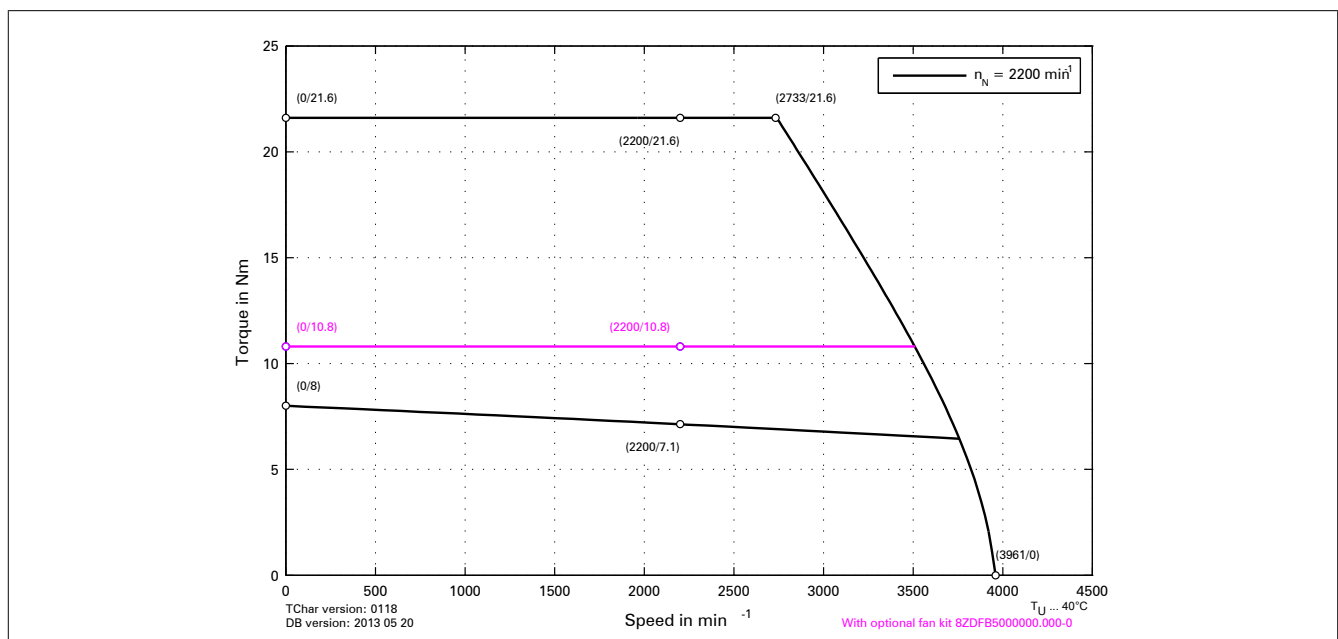
Figure 2: 8DI54e.ffggghijk-I at 750 VDC DC bus voltage - Speed-torque characteristic curve
