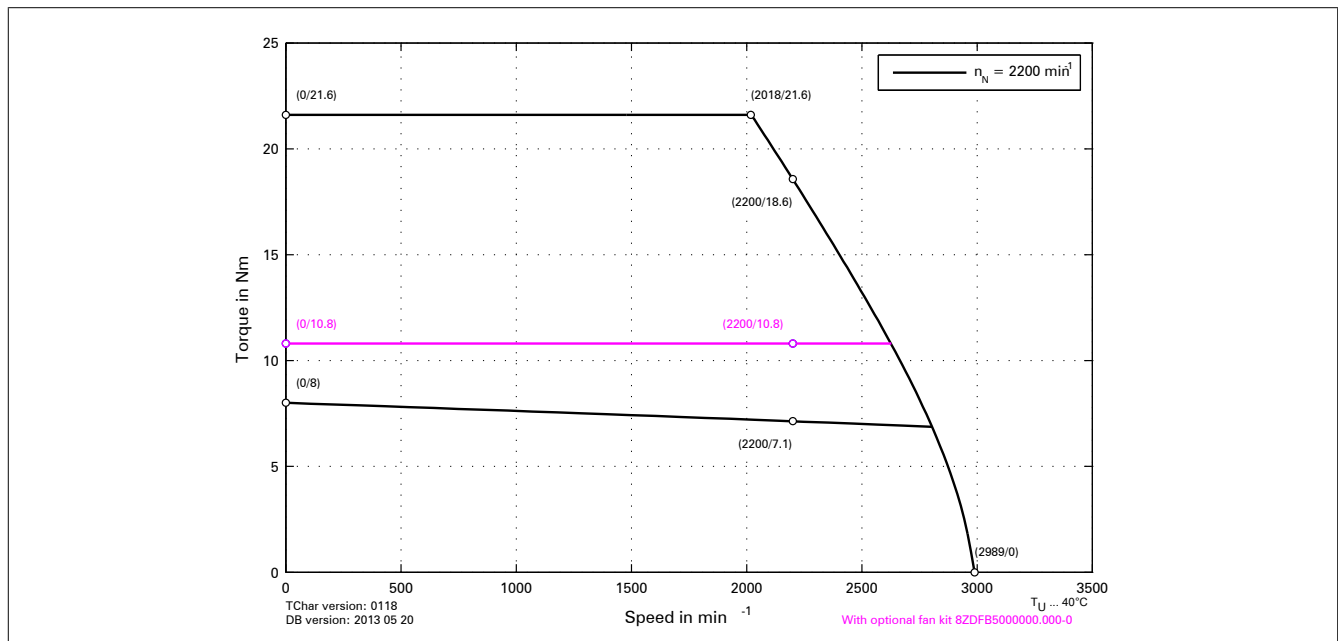
Figure 1: 8DI54e.ffggghijk-I at 560 VDC DC bus voltage - Speed-torque characteristic curve
