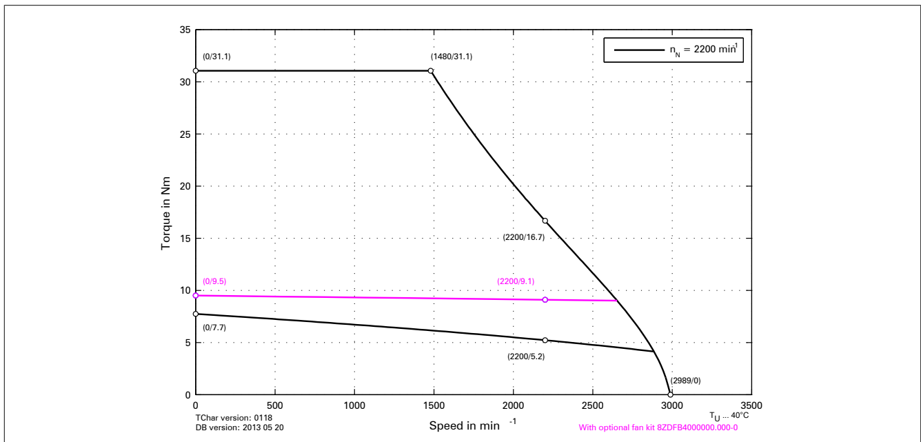
Figure 1: 8DI460.ffggghijk-I at 560 VDC DC bus voltage - Speed-torque characteristic curve
