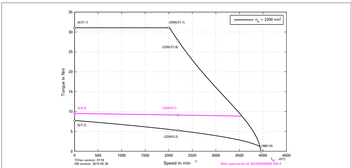
Figure 2: 8DI460.ffggghijk-I at 750 VDC DC bus voltage - Speed-torque characteristic curve
