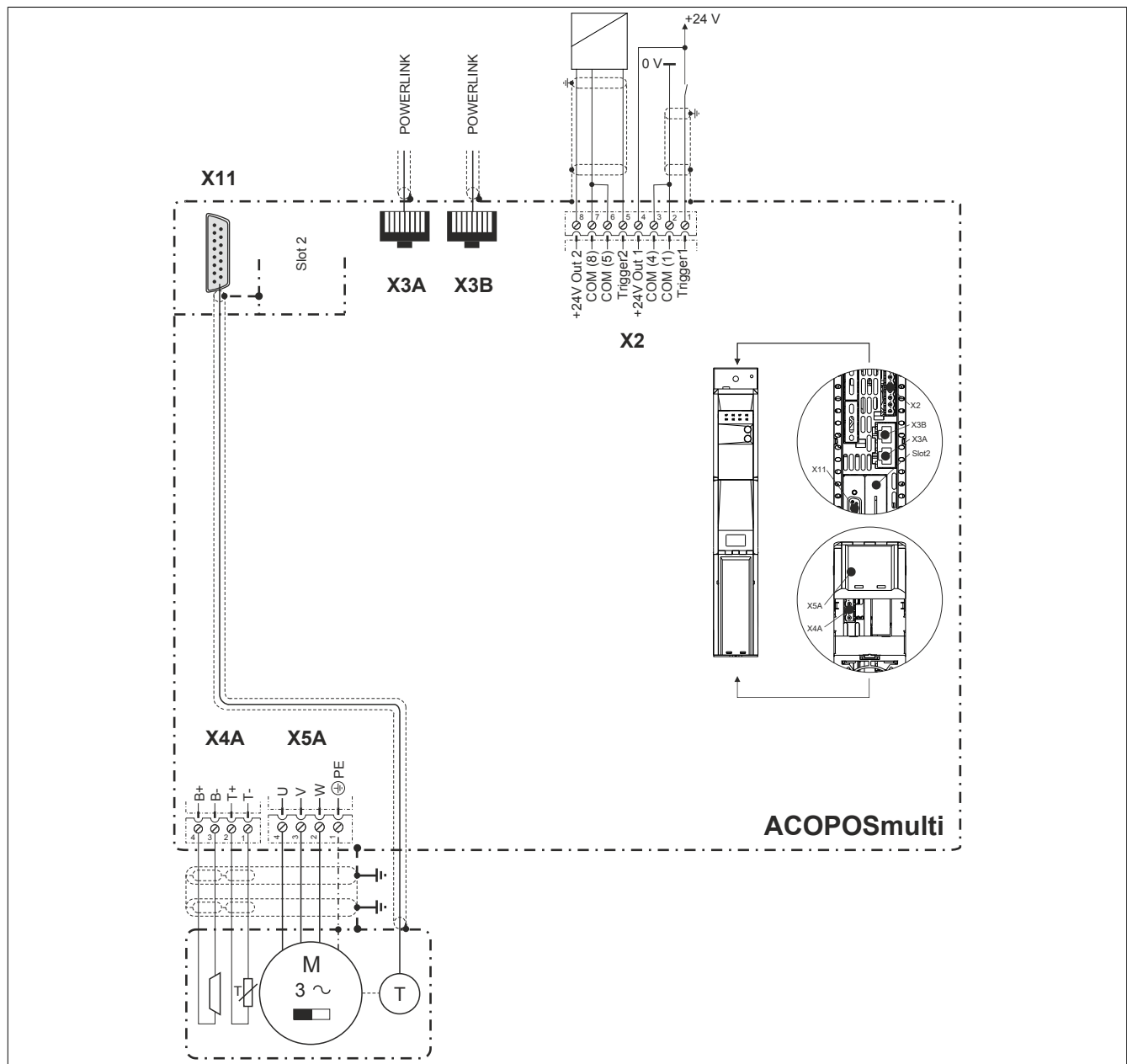
Figure 3: Pinout overview
