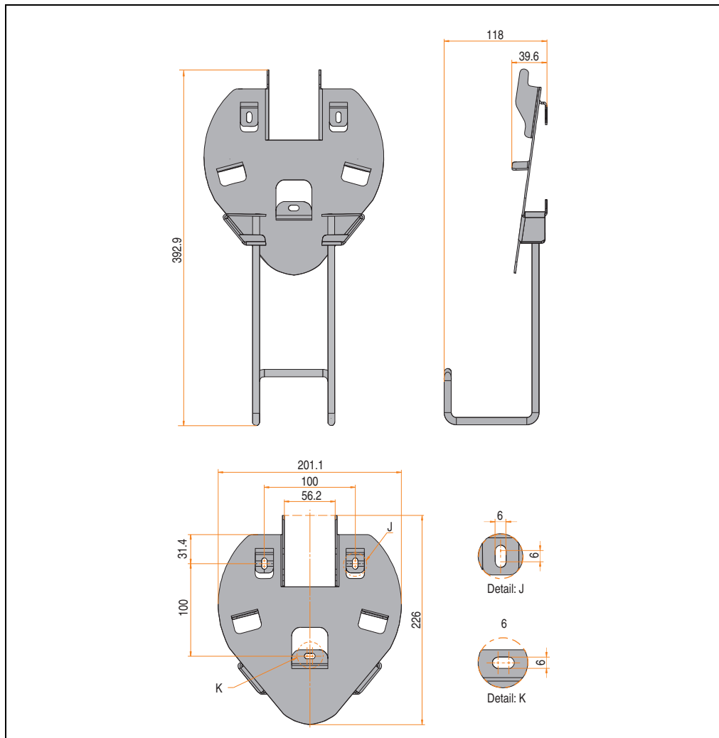
Figure 32: Dimensions - Wall mount 4MPBRA.0000-01
