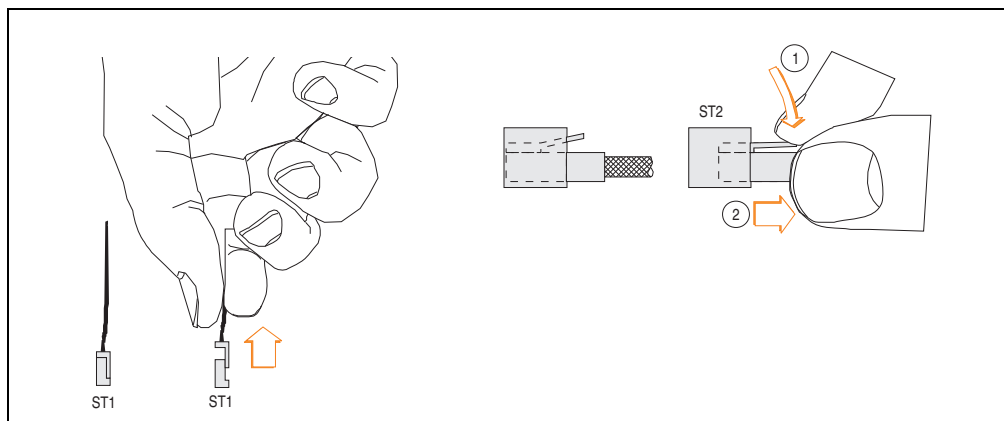
Figure 34: Removing ST1 and ST2
