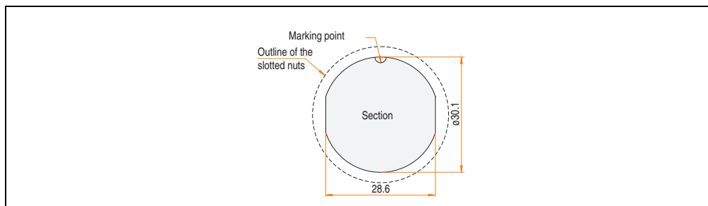
Figure 30: Drilling template - Receptacle
