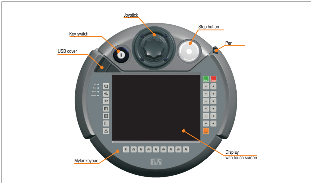
Figure 20: Operating unit 5MP050.0653-02
