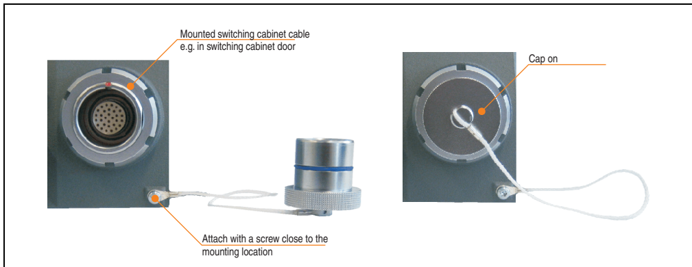
Figure 55: Attaching the switching cabinet cable protective cap
