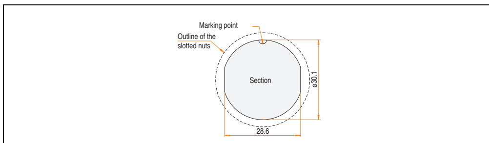
Figure 27: Drilling template - Receptacle
