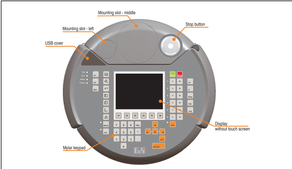
Figure 17: Operating unit 5MP040.0381-01
