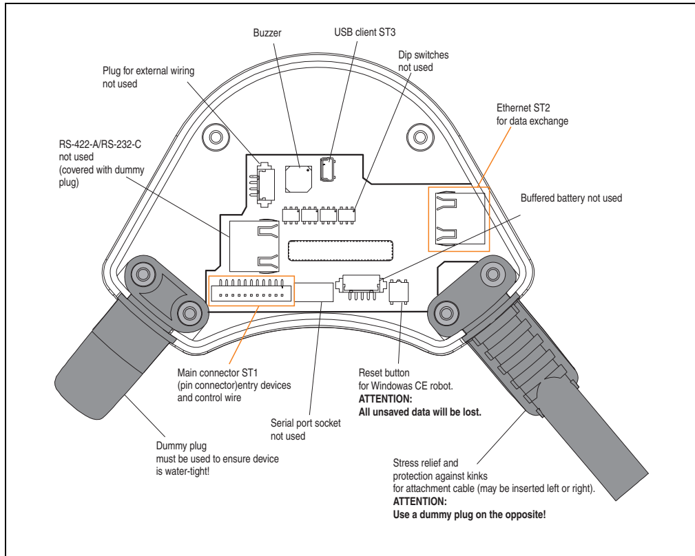
Figure 33: Attachment shaft
