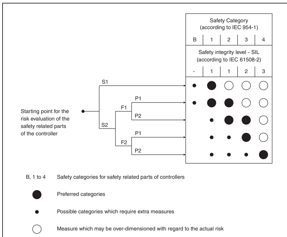
Figure 49: Risk graph according to EN 954-1, Appendix B
