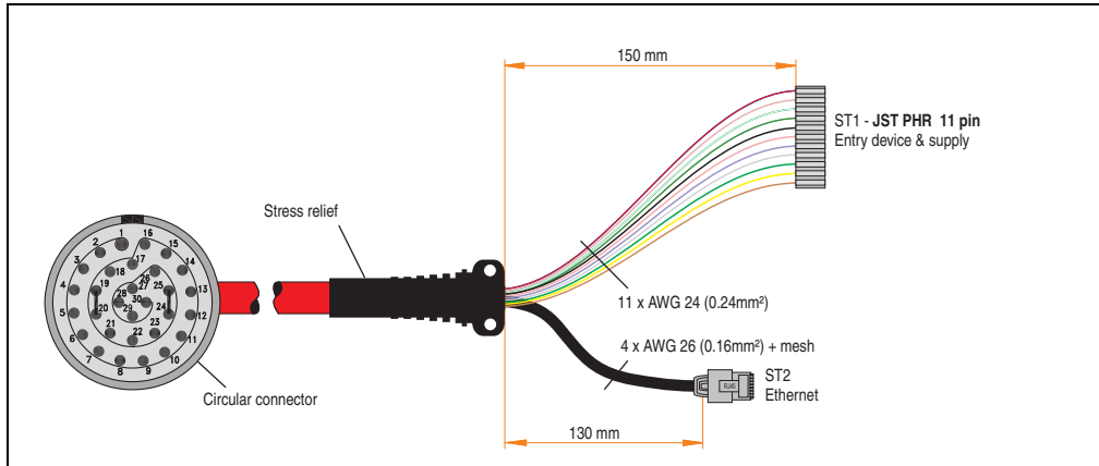
Figure 24: Attachment cable specifications 5CAMPH.0xxx-30
