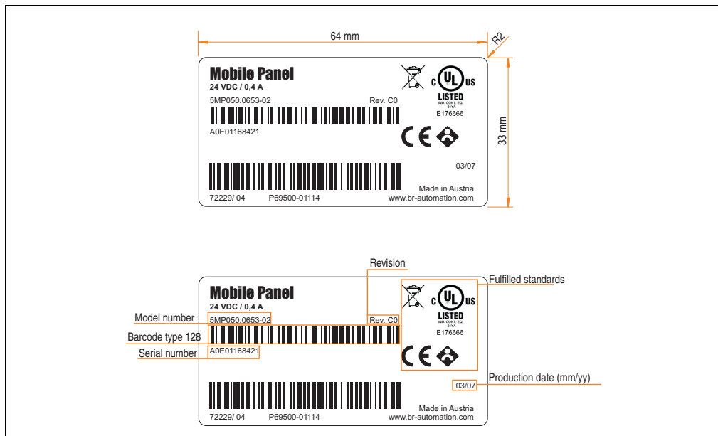
Figure 7: Design/dimensions - Serial number sticker
