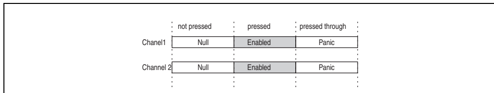
Figure 13: Possible enable switch positions
