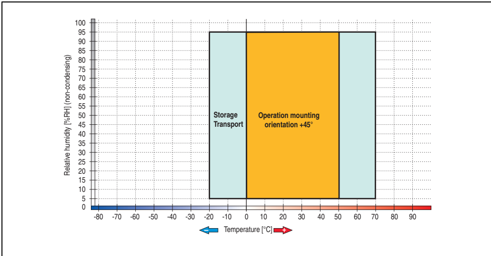
Figure 6: Temperature humidity diagram
