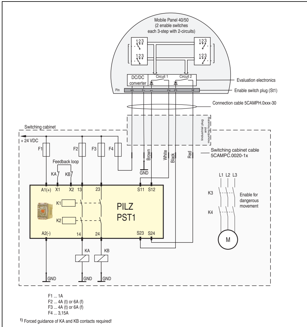
Figure 38: Connection example - Enable switch
