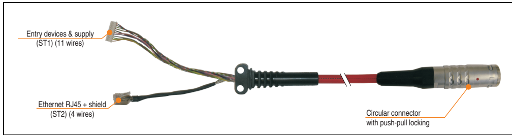
Figure 23: Attachment cable 5CAMPH.0xxx-30
