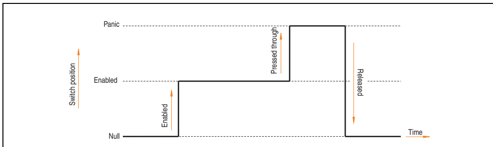
Figure 16: Enable switch - panic
