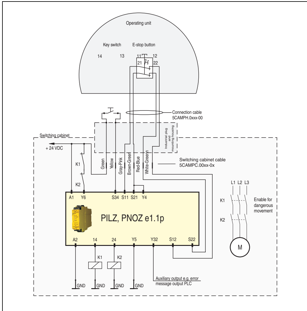
Figure 37: Connection example for stop button
