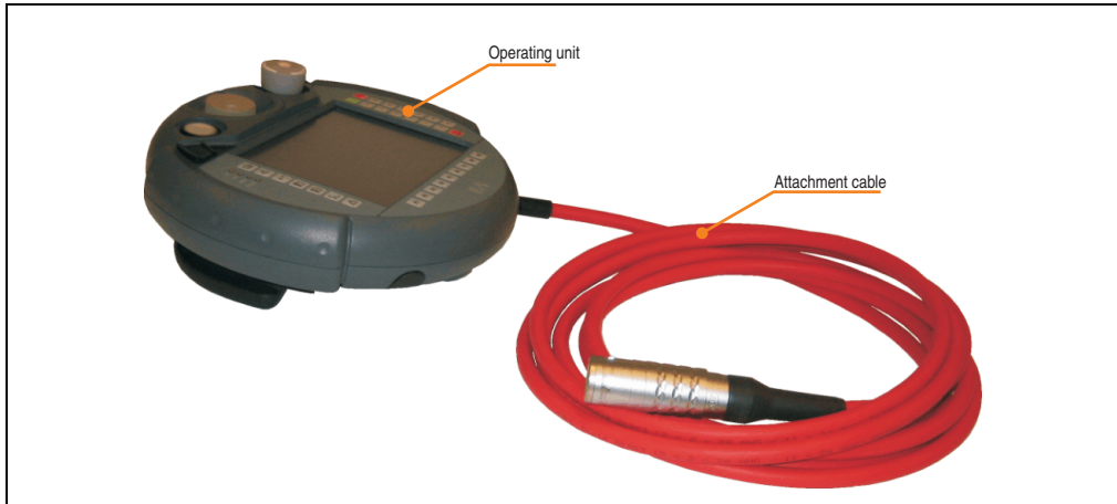
Figure 2: Construction
