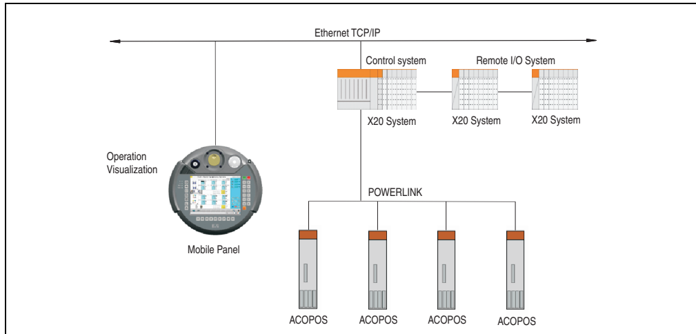
Figure 41: Connection to a B&R controller (e.g. X20)
