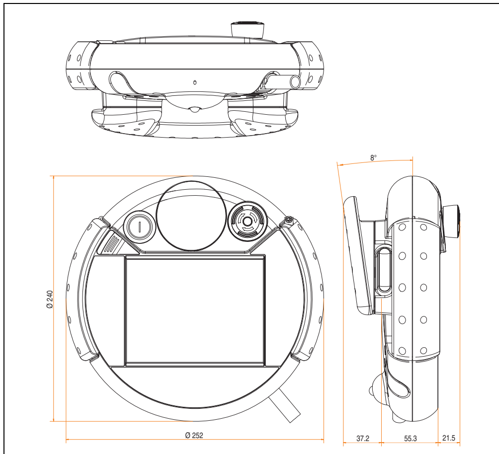
Figure 5: Entire device - Dimensions
