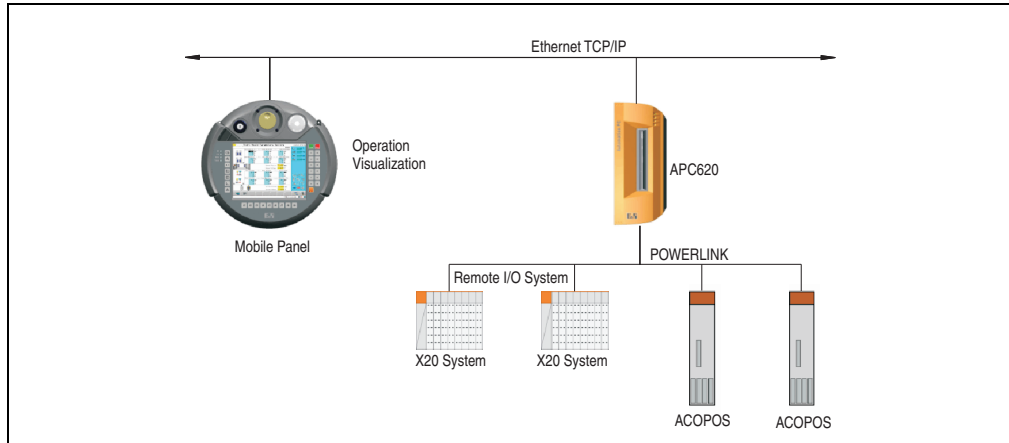
Figure 42: Mobile thin client
