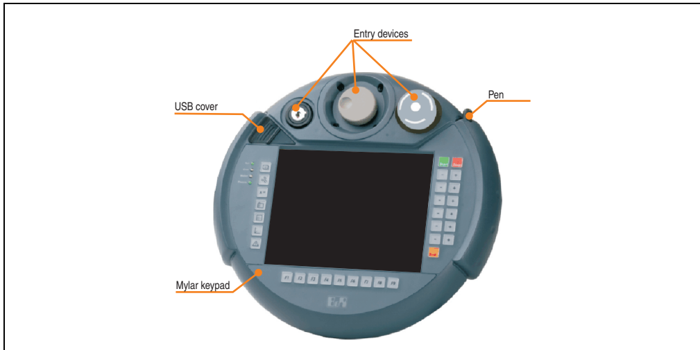
Figure 9: Mobile Panel operating unit
