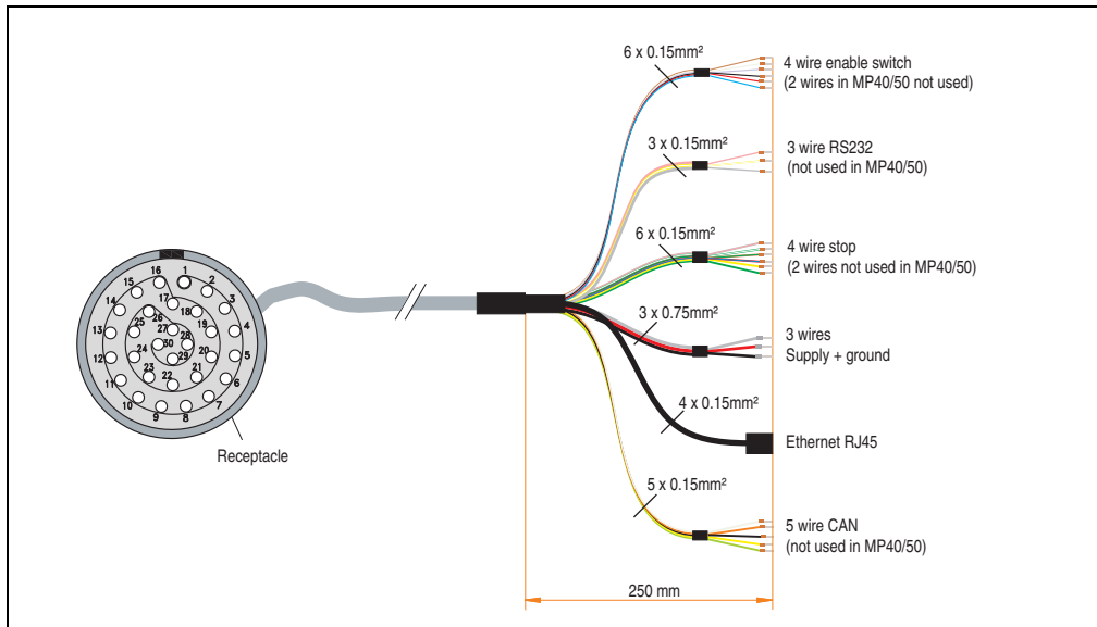
Figure 26: Cable layout - switching cabinet cable 5CAMPC.0020-10
