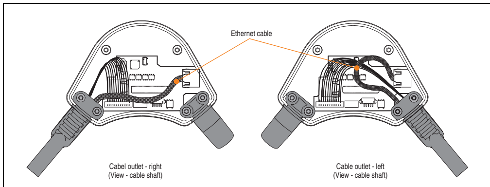
Figure 35: Cable outlet
