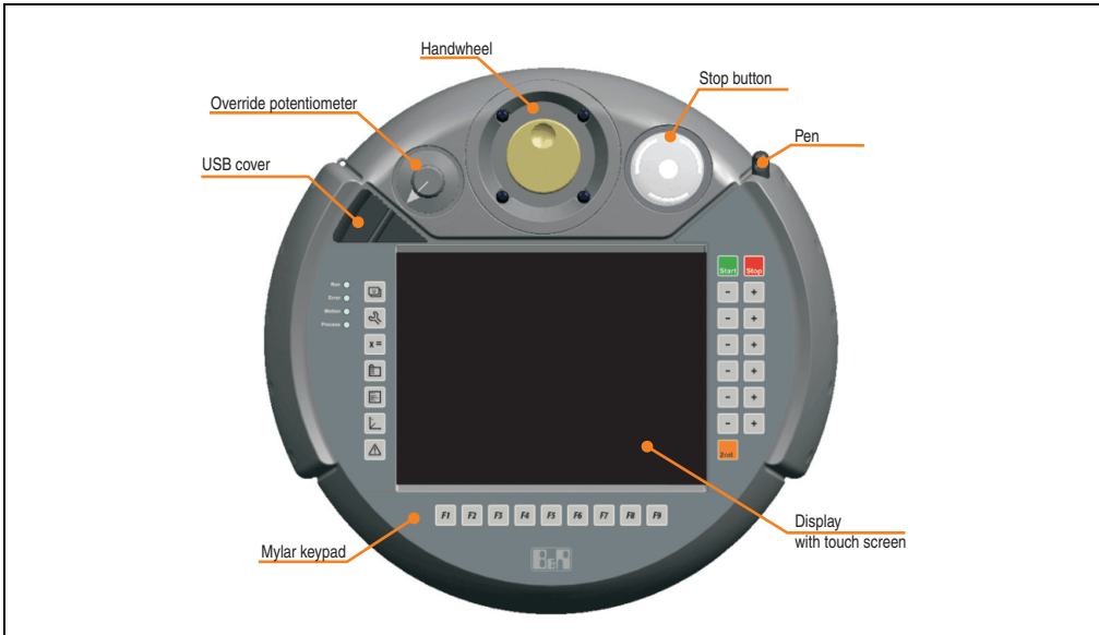
Figure 21: Operating unit 5MP050.0653-03
