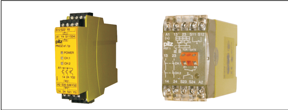
Figure 36: Pilz PNOZ e1.1p (left) and Pilz PNOZ PST1 (right)
