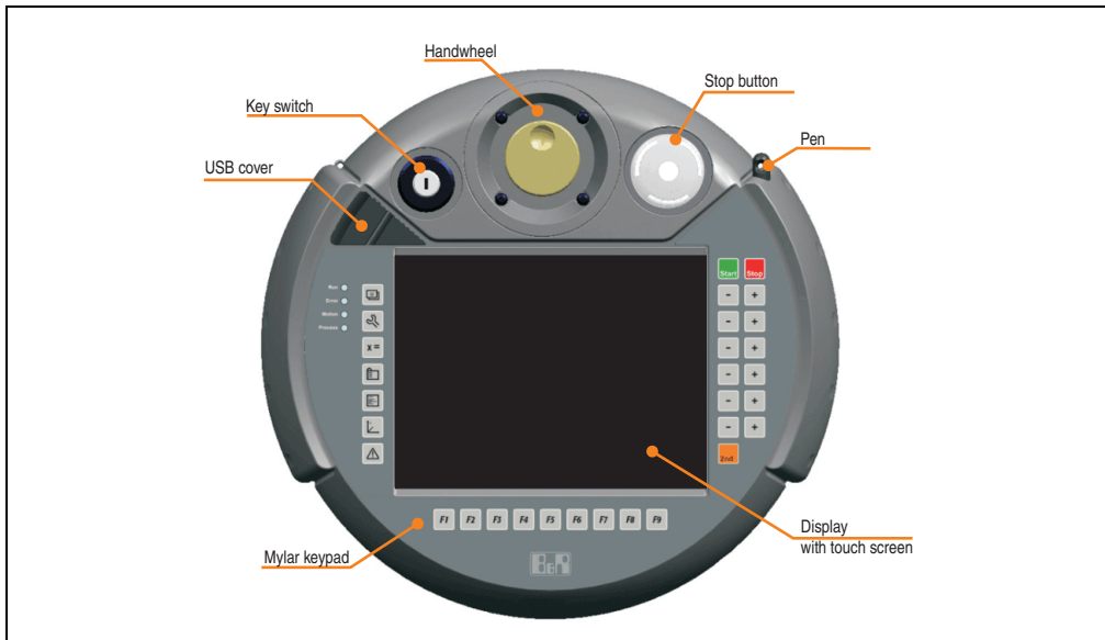
Figure 22: Operating unit 5MP050.0653-04
