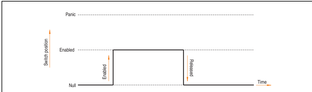
Figure 15: Enable switch - enable
