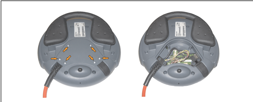
Figure 58: Remove the cover of the connection compartment
