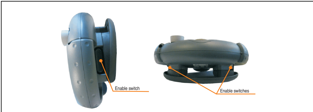
Figure 12: Enabling device
