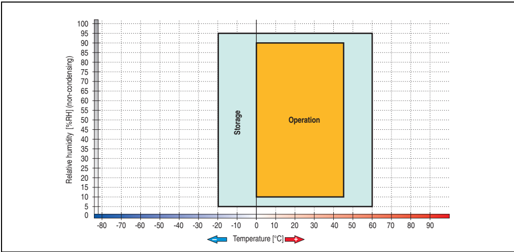
Figure 50: Temperature humidity diagram - USB flash drive - 5MMUSB.xxxx-00
