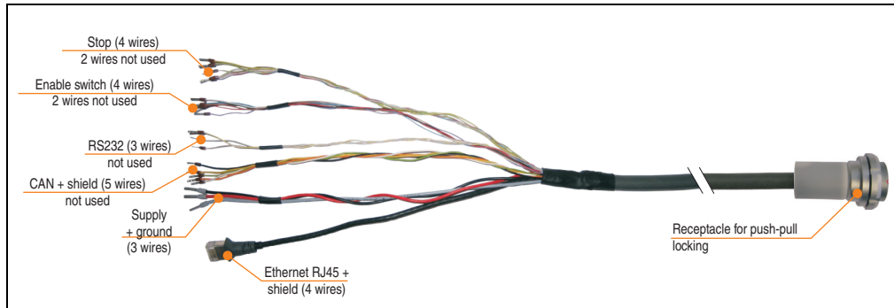
Figure 28: Mobile Panel switching cabinet cable 5CAMPC.0020-11
