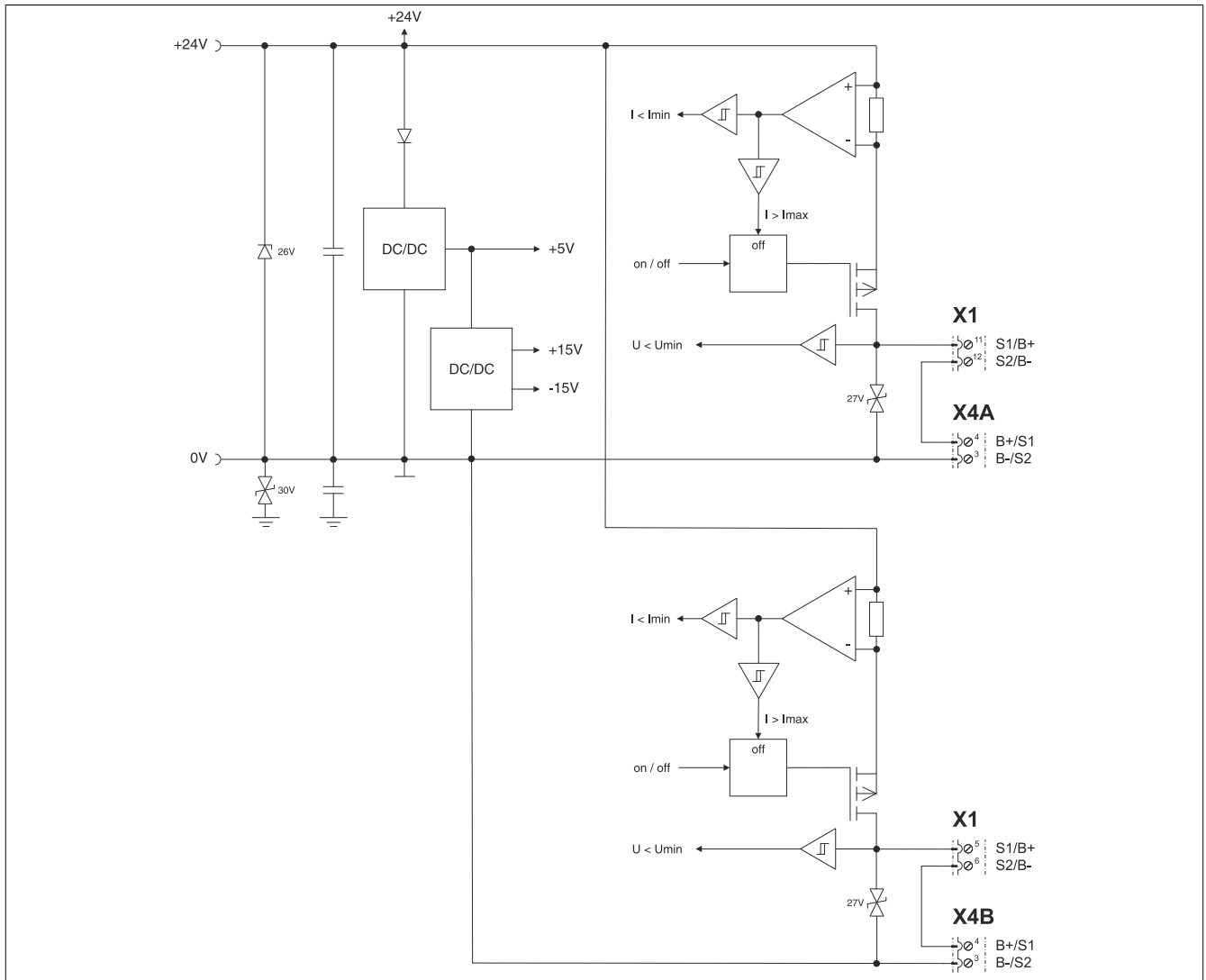
Figure 8: Holding brake
