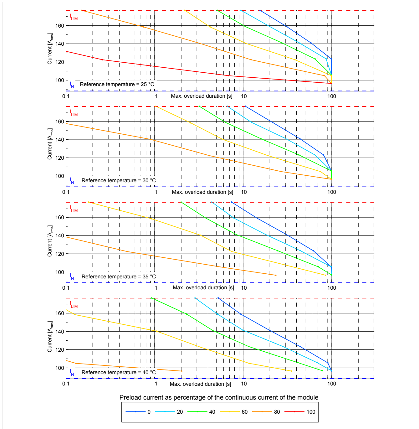
Figure 1: Overload characteristics of 8BVI0880HWSx.004-1, overload response - WARNING
