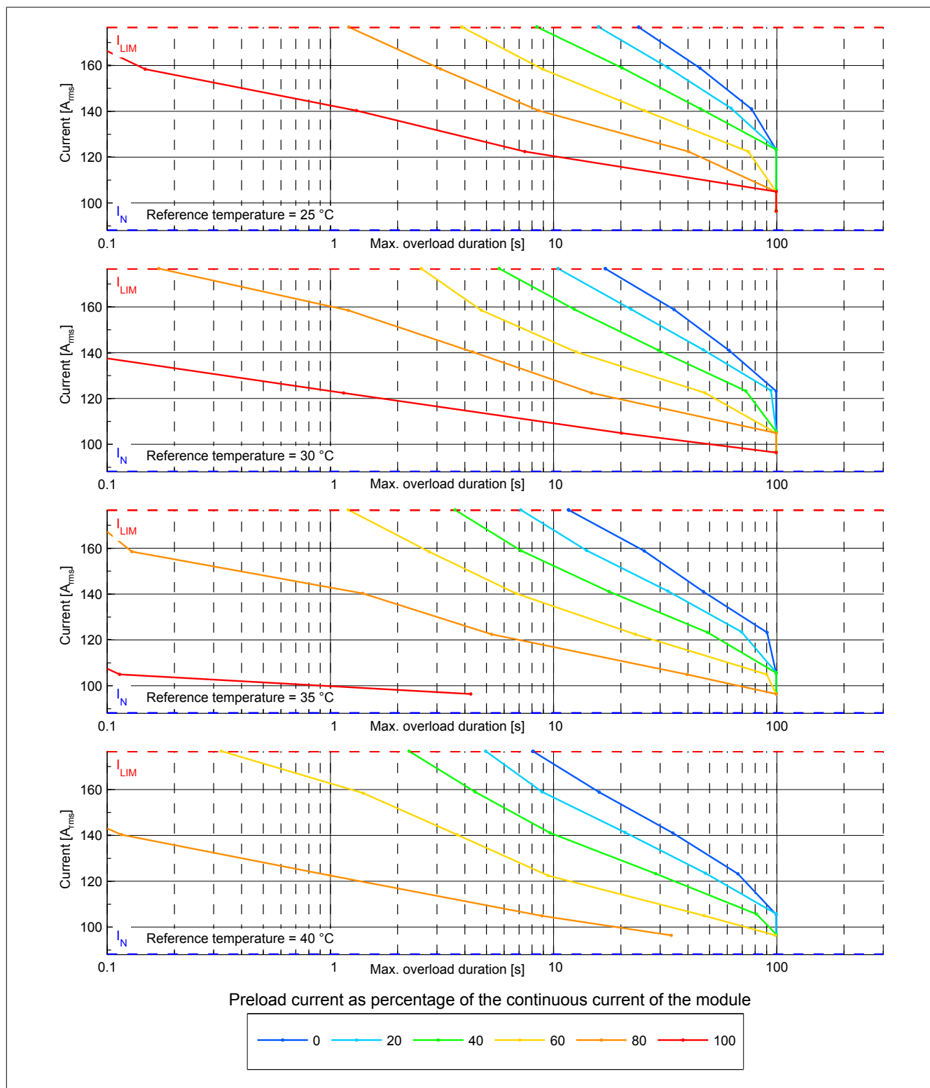
Figure 2: 8BVI0880HWSx.004-1 - Overload characteristics, overload response ERROR+STOP
