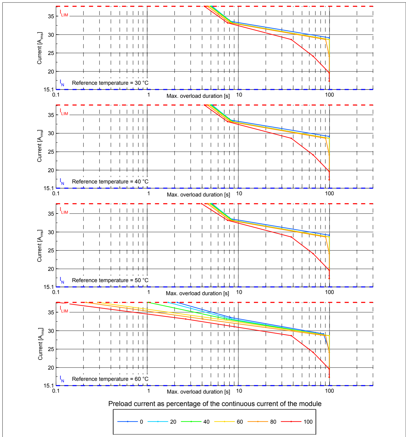
Figure 2: 8BVI0110HCSS.000-x - Overload characteristics, overload response - ERROR+STOP
