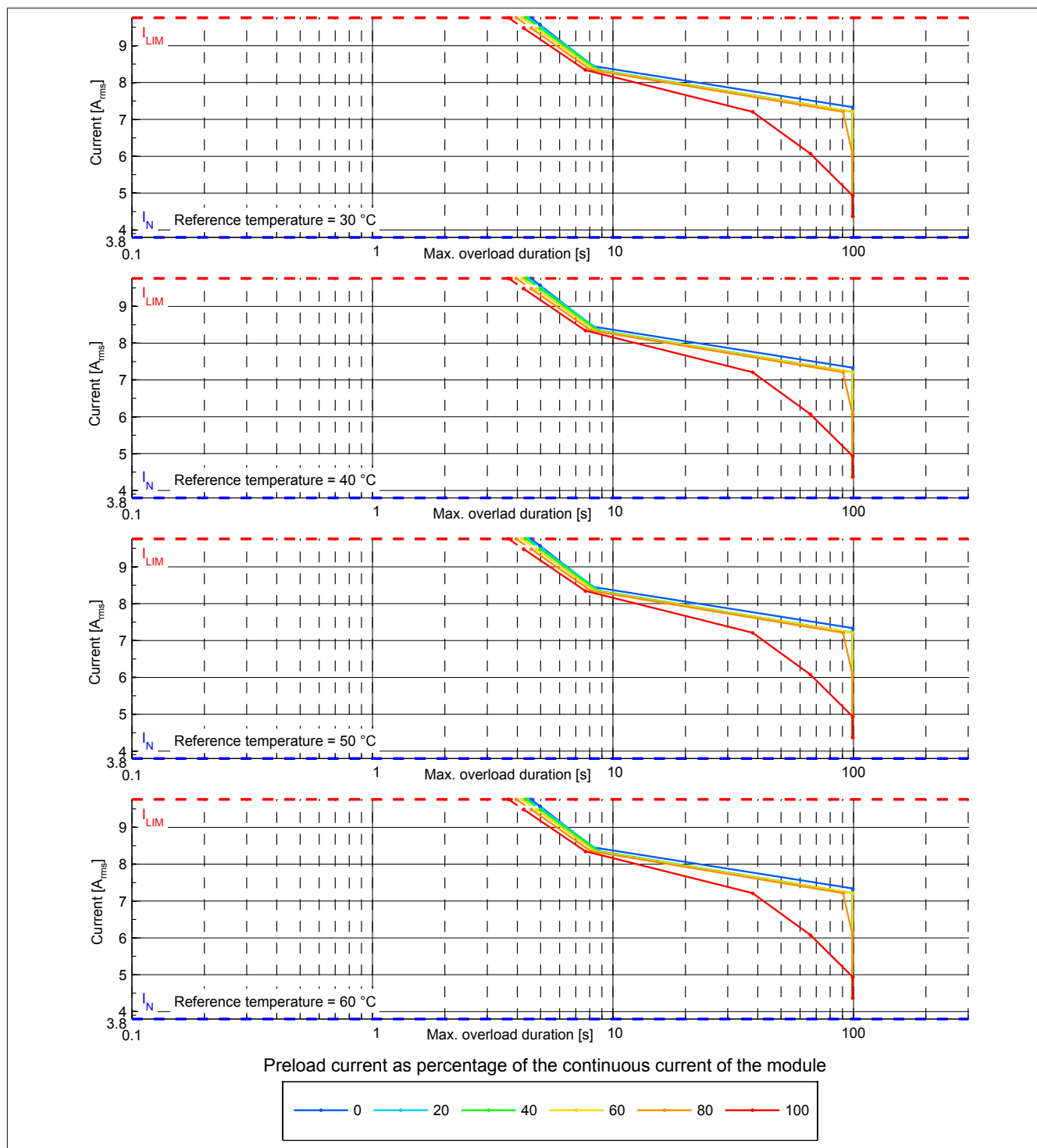
Figure 2: 8BVI0028HCSx.000-x_8BVI0028HCDx.000-x - Overload characteristics, overload response - ERROR+STOP
