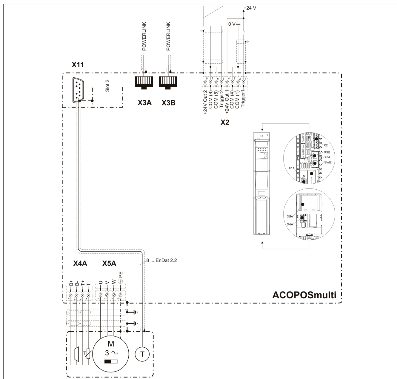
Figure 8: Pinout overview
