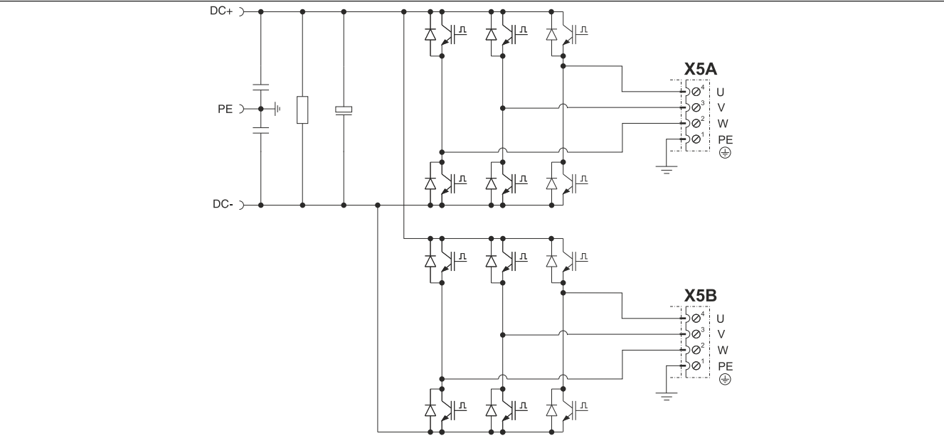
Figure 10: Motor
