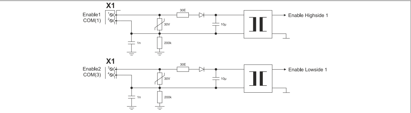
Figure 6: Enable
