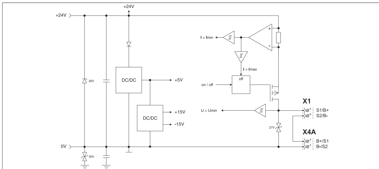
Figure 9: Holding brake
