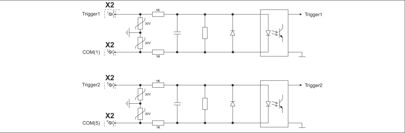
Figure 7: Trigger inputs
