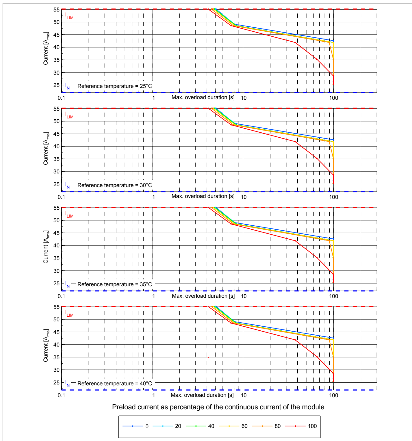
Figure 1: 8BVI0220HWSx.000-x - Overload characteristics, overload response - WARNING
