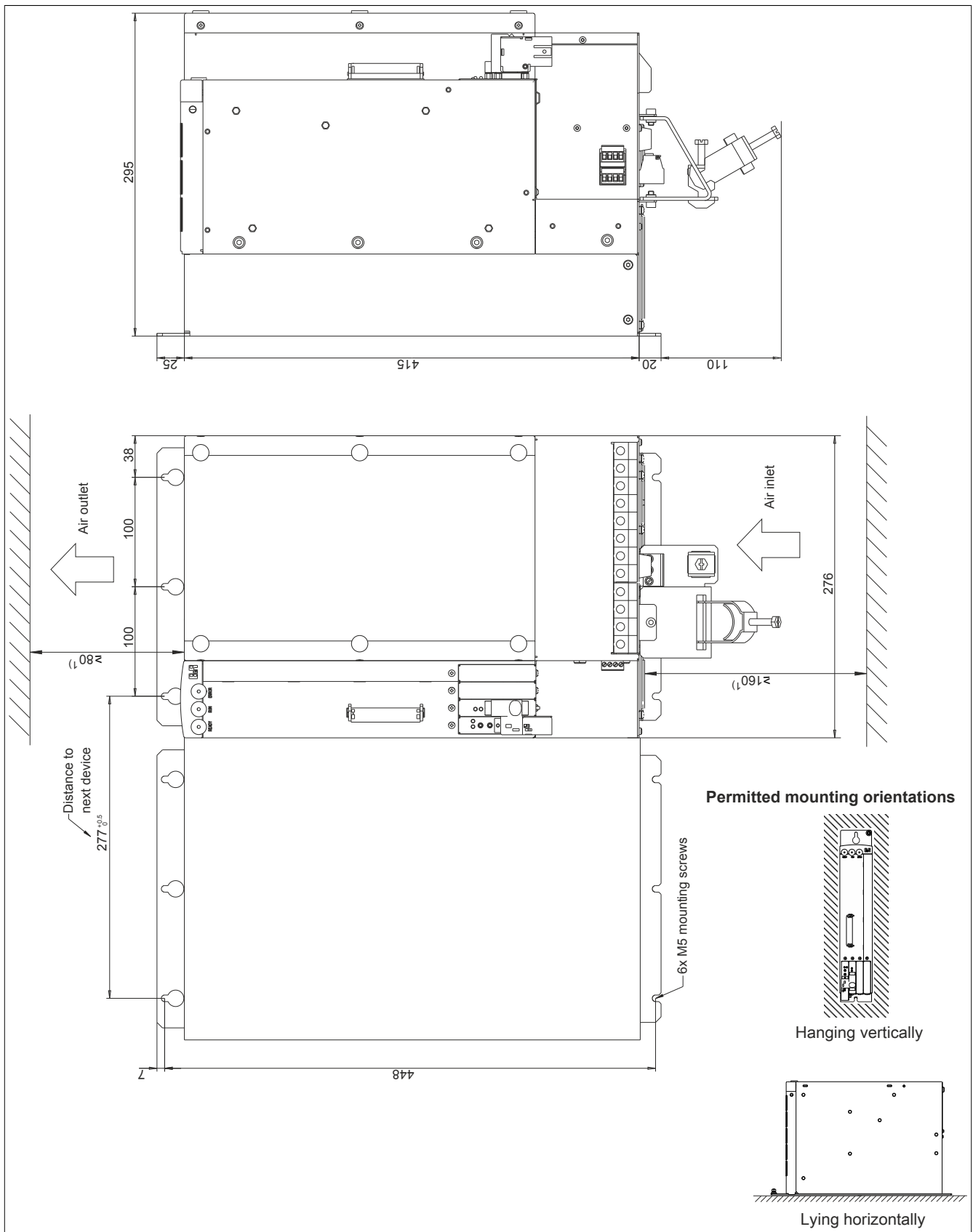
Figure 2: Dimension diagram and installation dimensions
