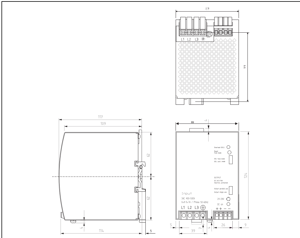
Figure 1: PS310 - dimensions
