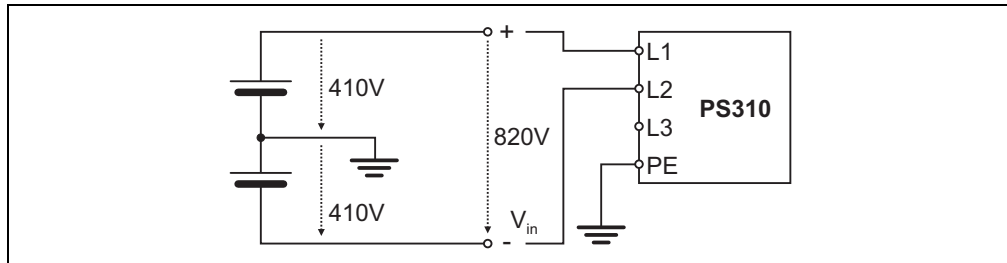
Figure 4: DC mains, grounded neutral point
