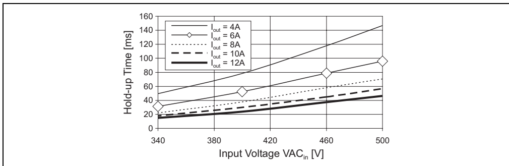
Figure 10: PS310 - hold-up time, 3 phase (min., at V_{out} = 24 V)
