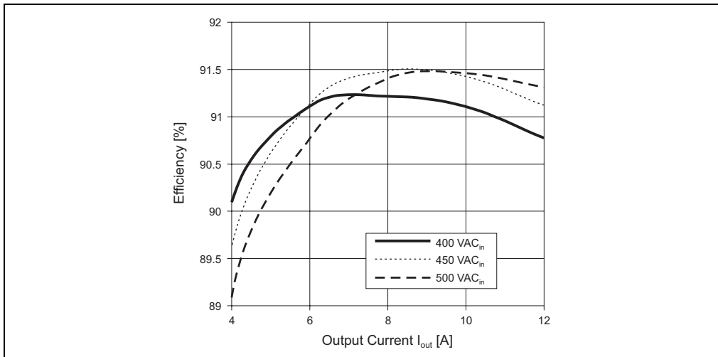
Figure 9: PS310 - efficiency -2 phase (min., at V_{out} = 24 V)
