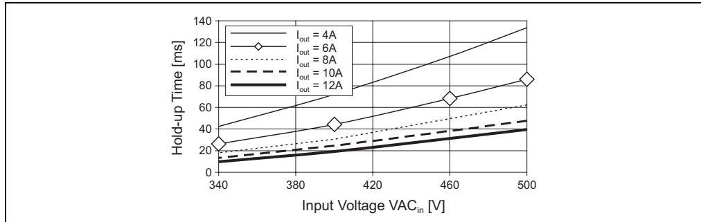
Figure 11: PS310 - hold-up time, 2 phase (min., at V_{out} = 24\text{ V} )
