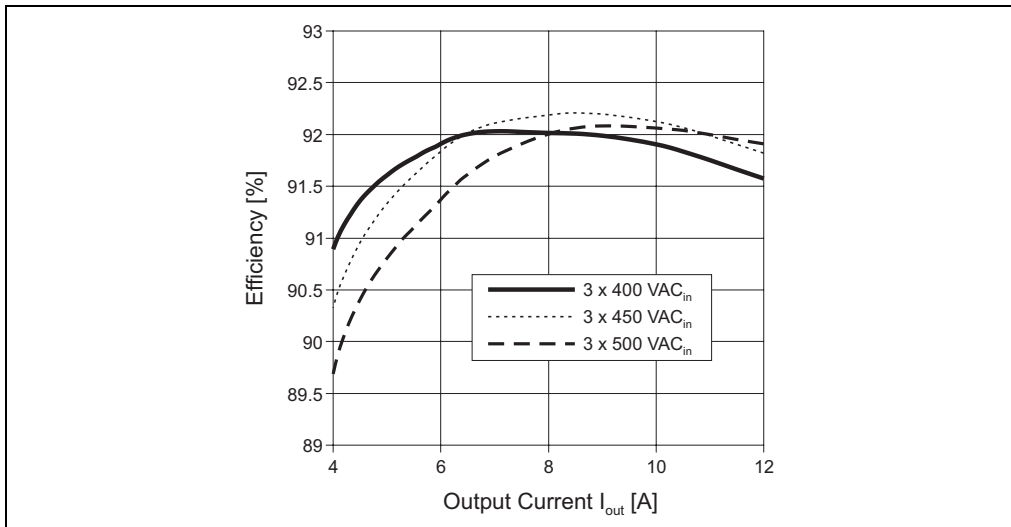
Figure 8: PS310 - efficiency - 3 phase (min., at V_{out} = 24 \text{ V} )
