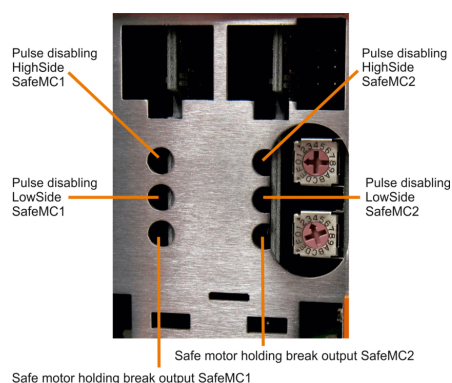
Figure 5: 2-axis modules
