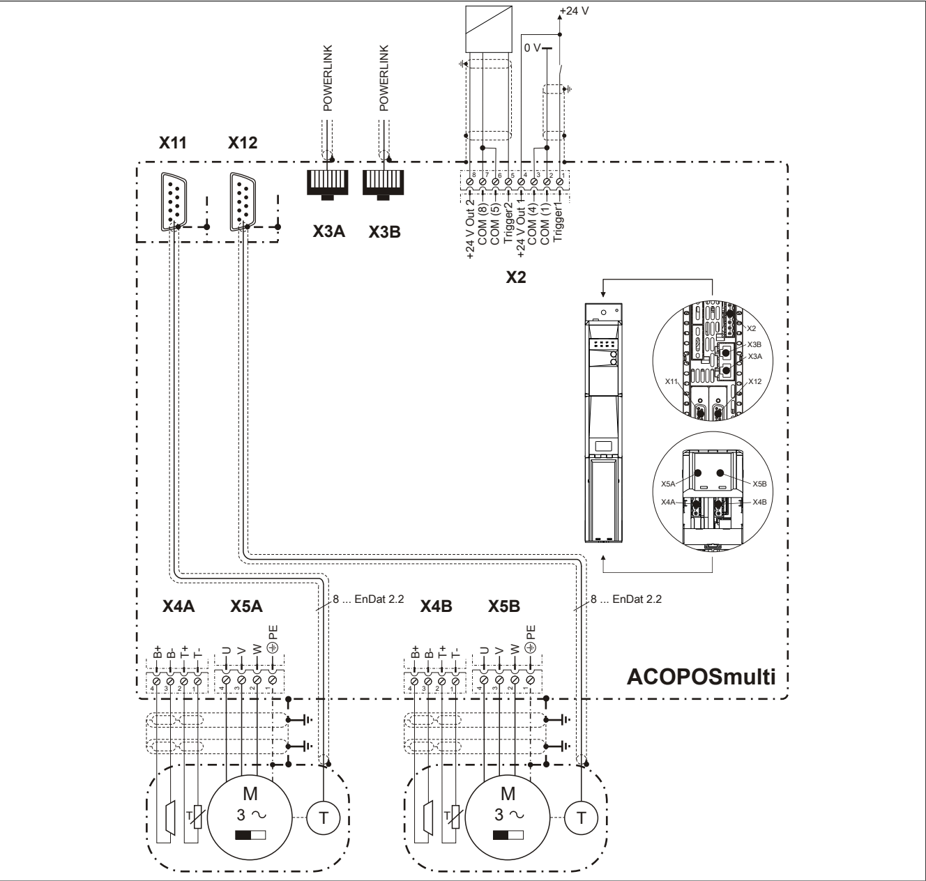
Figure 8: Pinout overview
