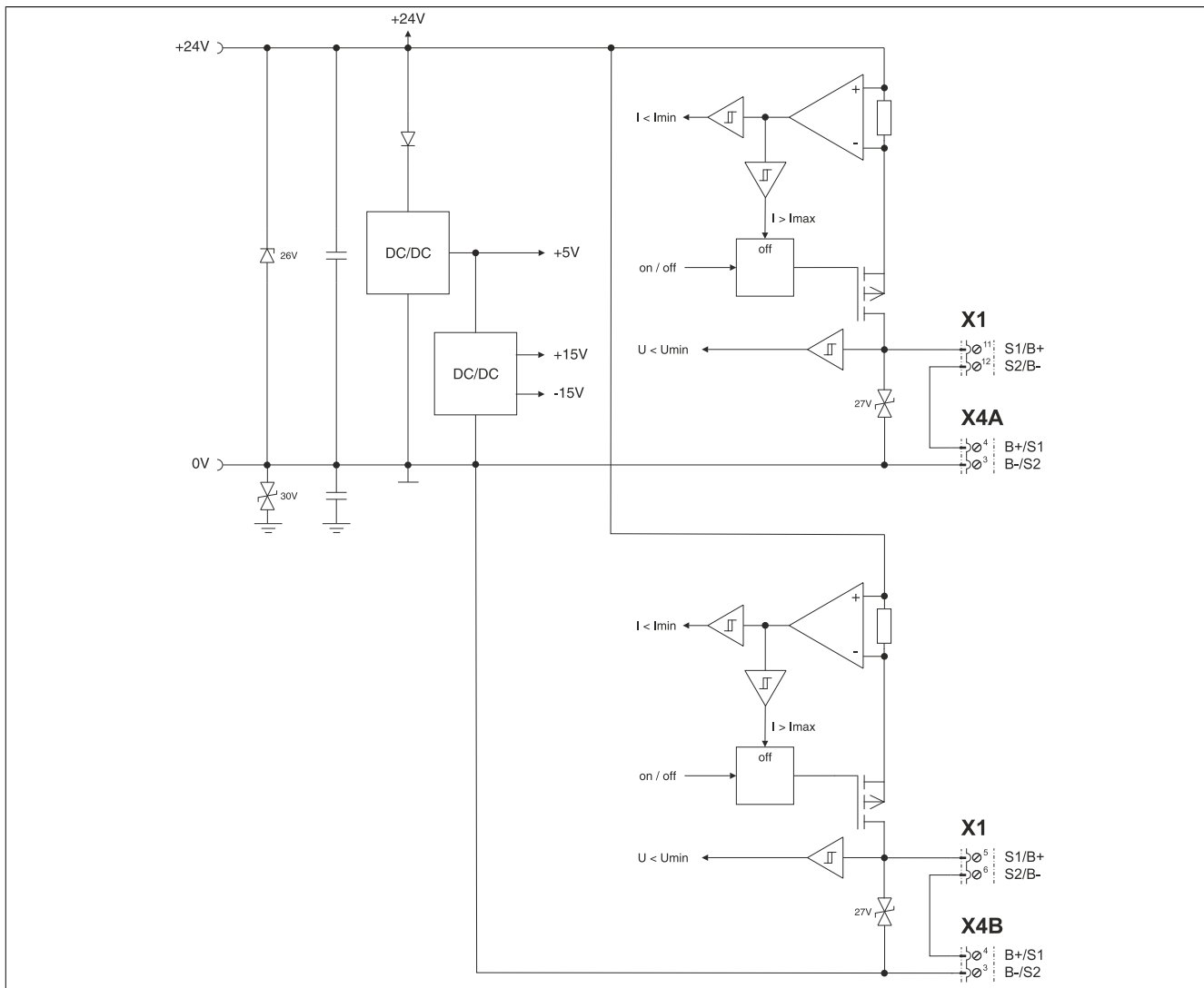
Figure 8: Holding brake
