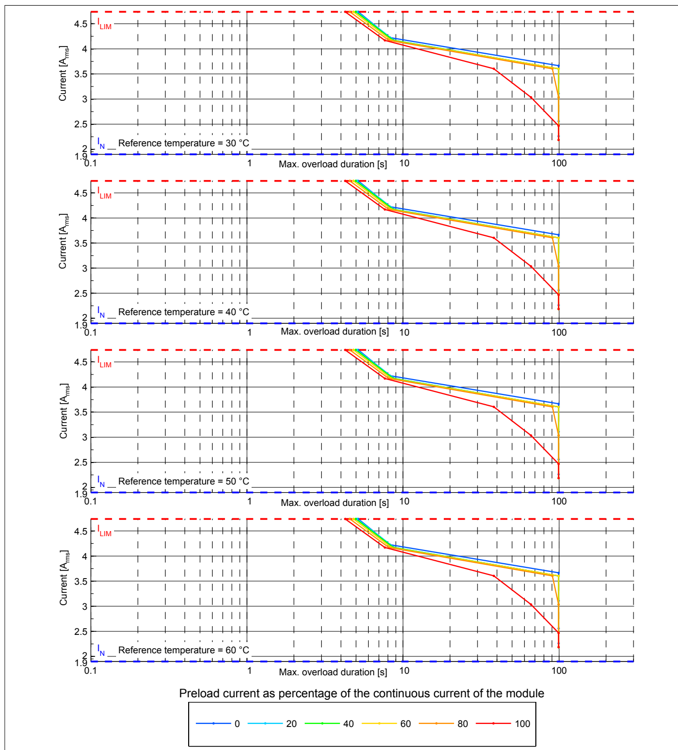
Figure 1: 8BVI0014HCDx.000-x - Overload characteristics, overload response - WARNING
