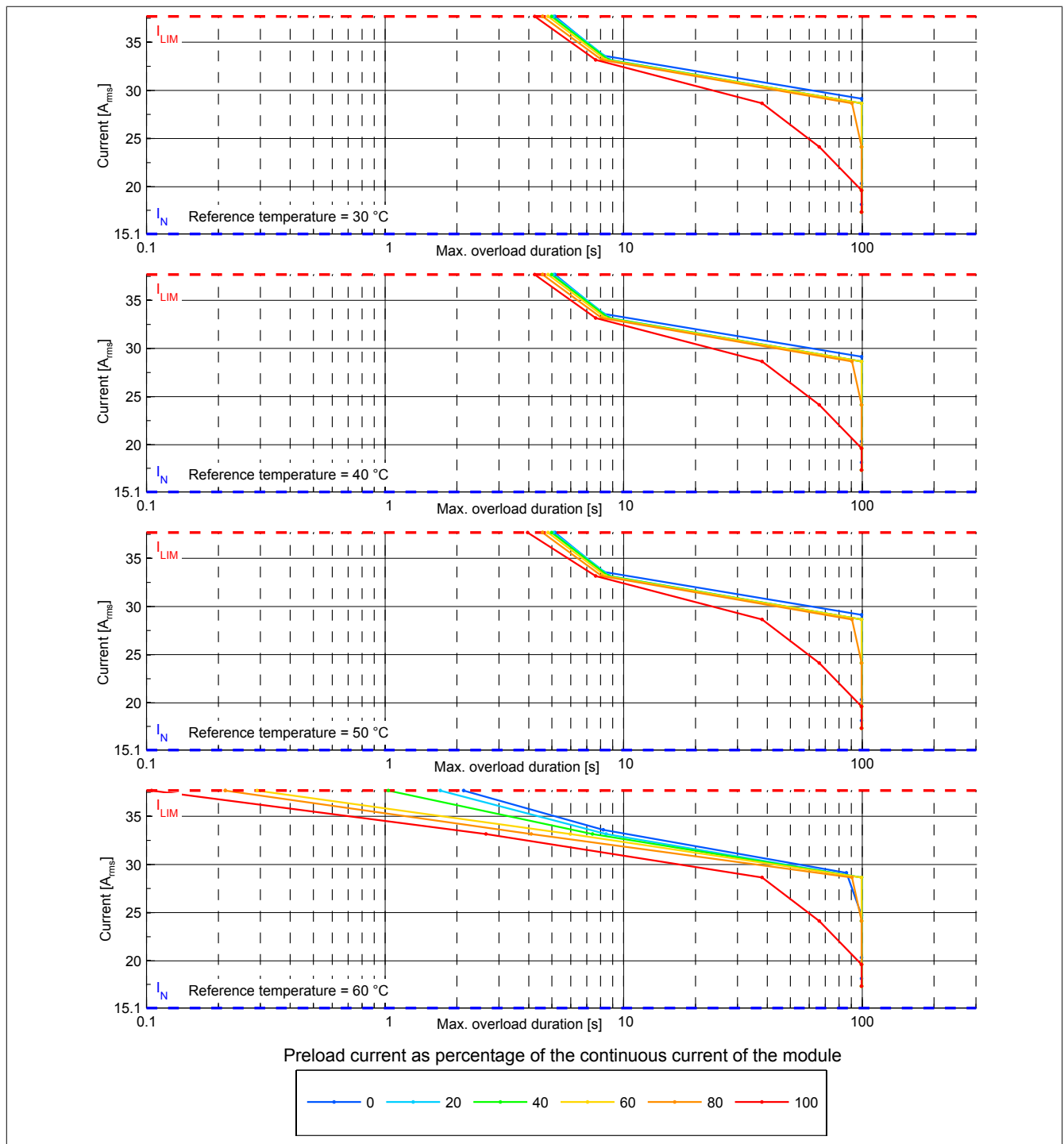
Figure 2: 8BVI0110HCDS.000-x - Overload characteristics, overload response - ERROR + STOP
