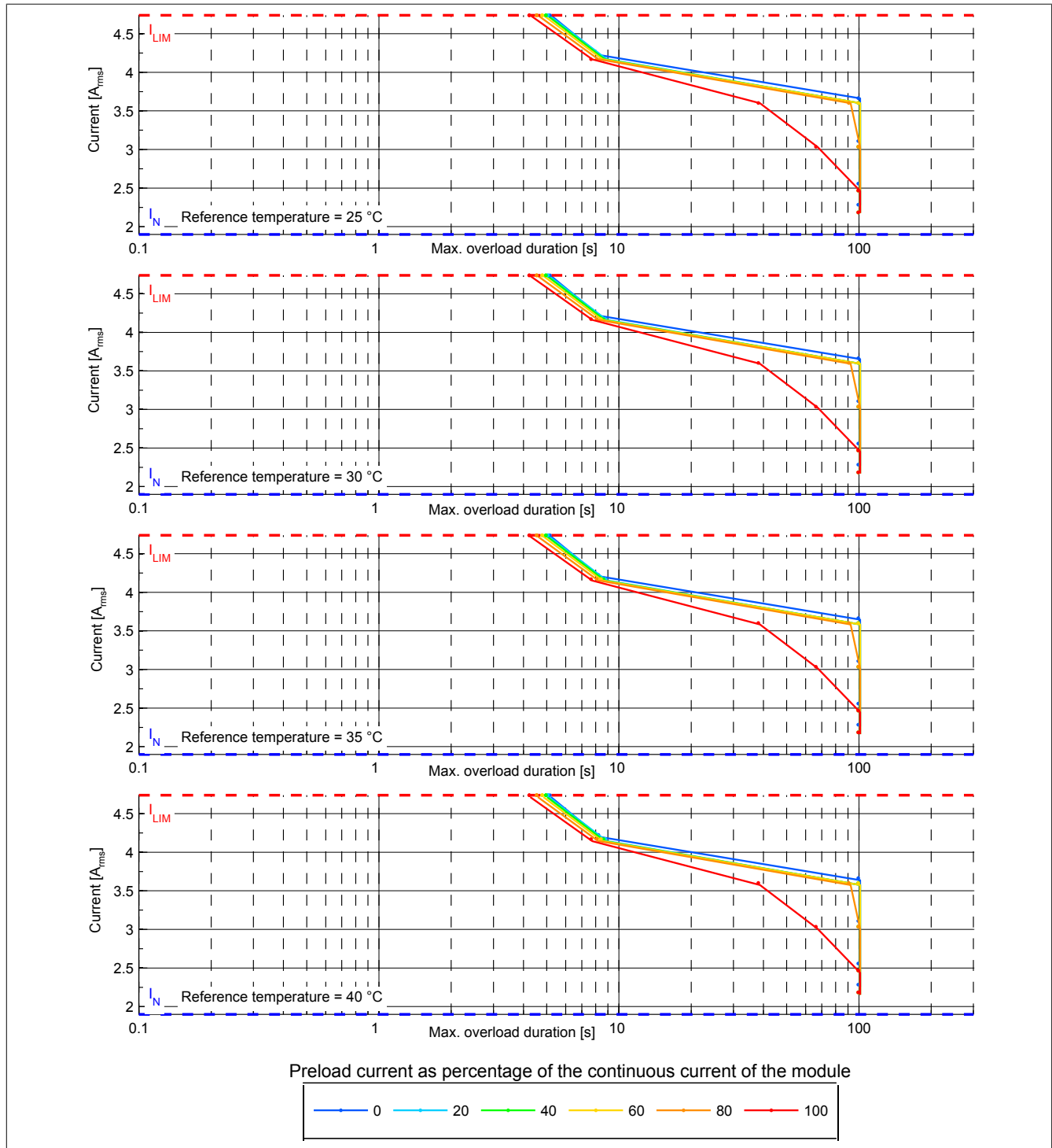
Figure 1: 8BVI0014HWDx.000-x - Overload characteristics, overload response - WARNING
