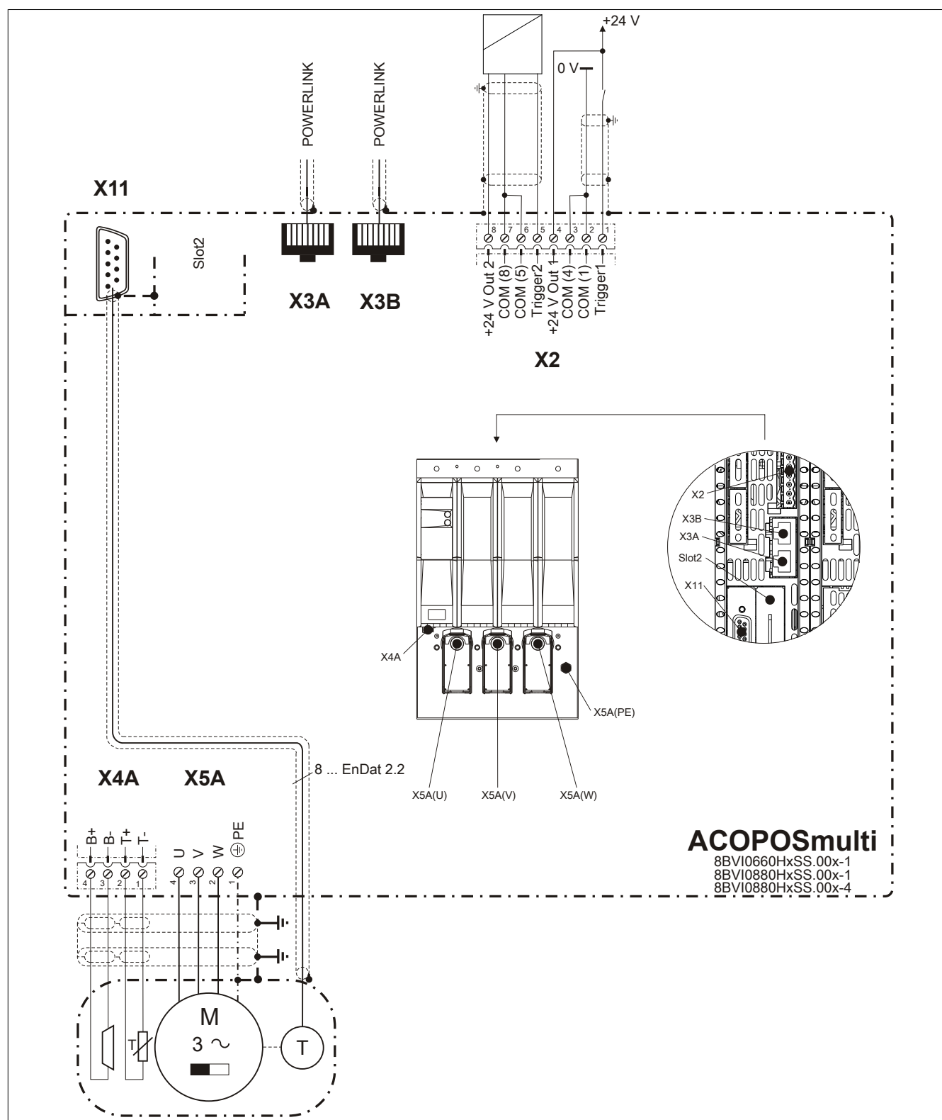
Figure 6: Pinout overview
