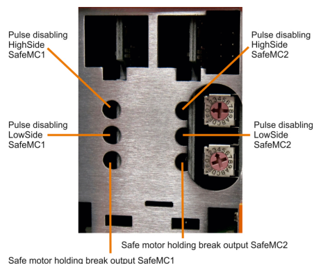
Figure 3: 2-axis modules
