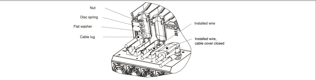
Figure 7: X5A - Cable installation
