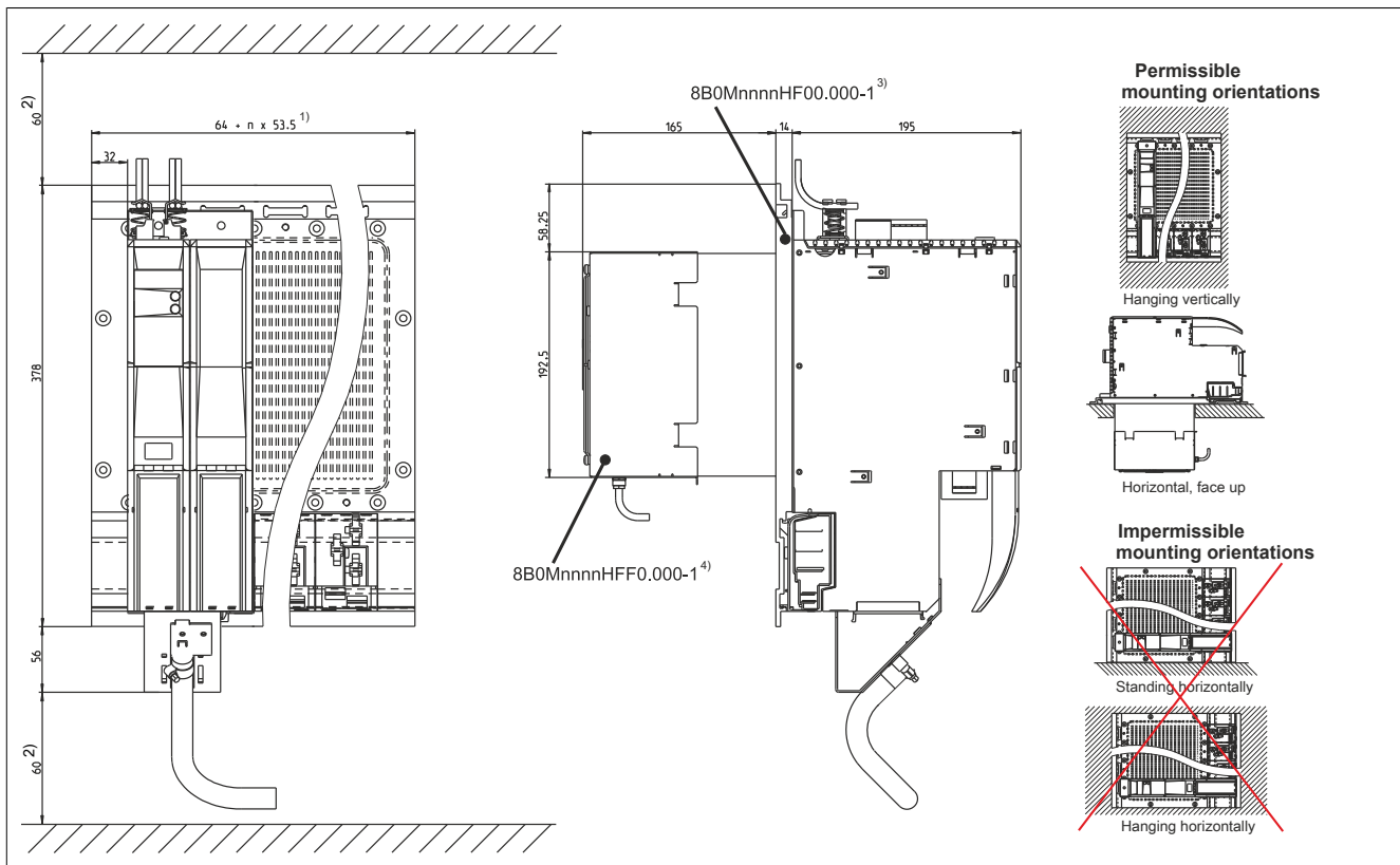
Figure 10: Feed-through mounting - Dimension diagram and installation dimensions
