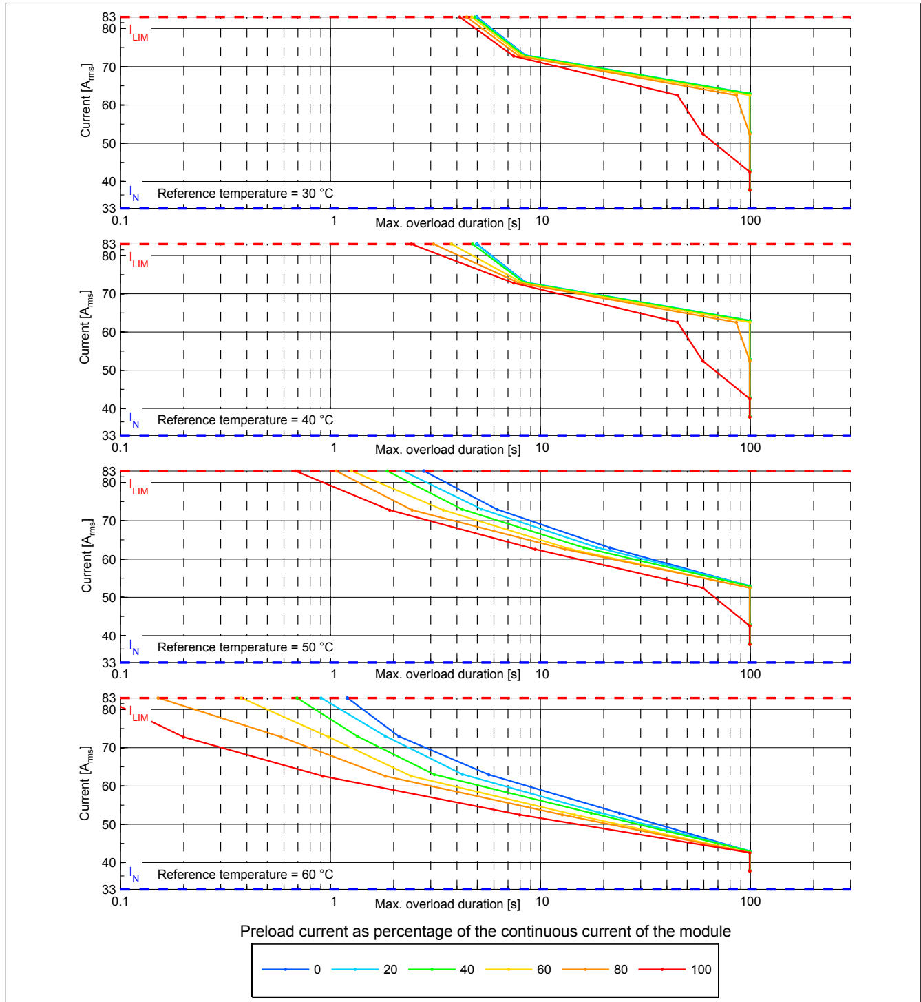
Figure 4: 8BVI0330HCSS.000-x - Overload characteristics, overload response - WARNING
