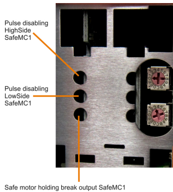
Figure 2: 1-axis modules
