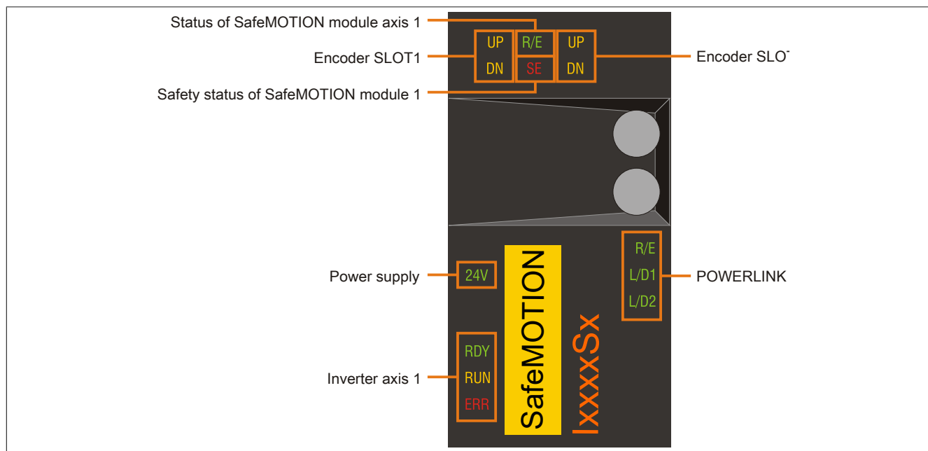
Figure 6: 8BVI SafeMOTION inverter modules (1-axis modules) - Status indicator groups
