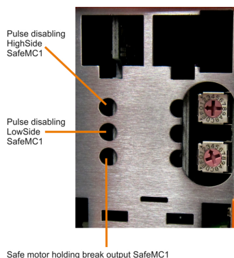
Figure 7: 1-axis modules
