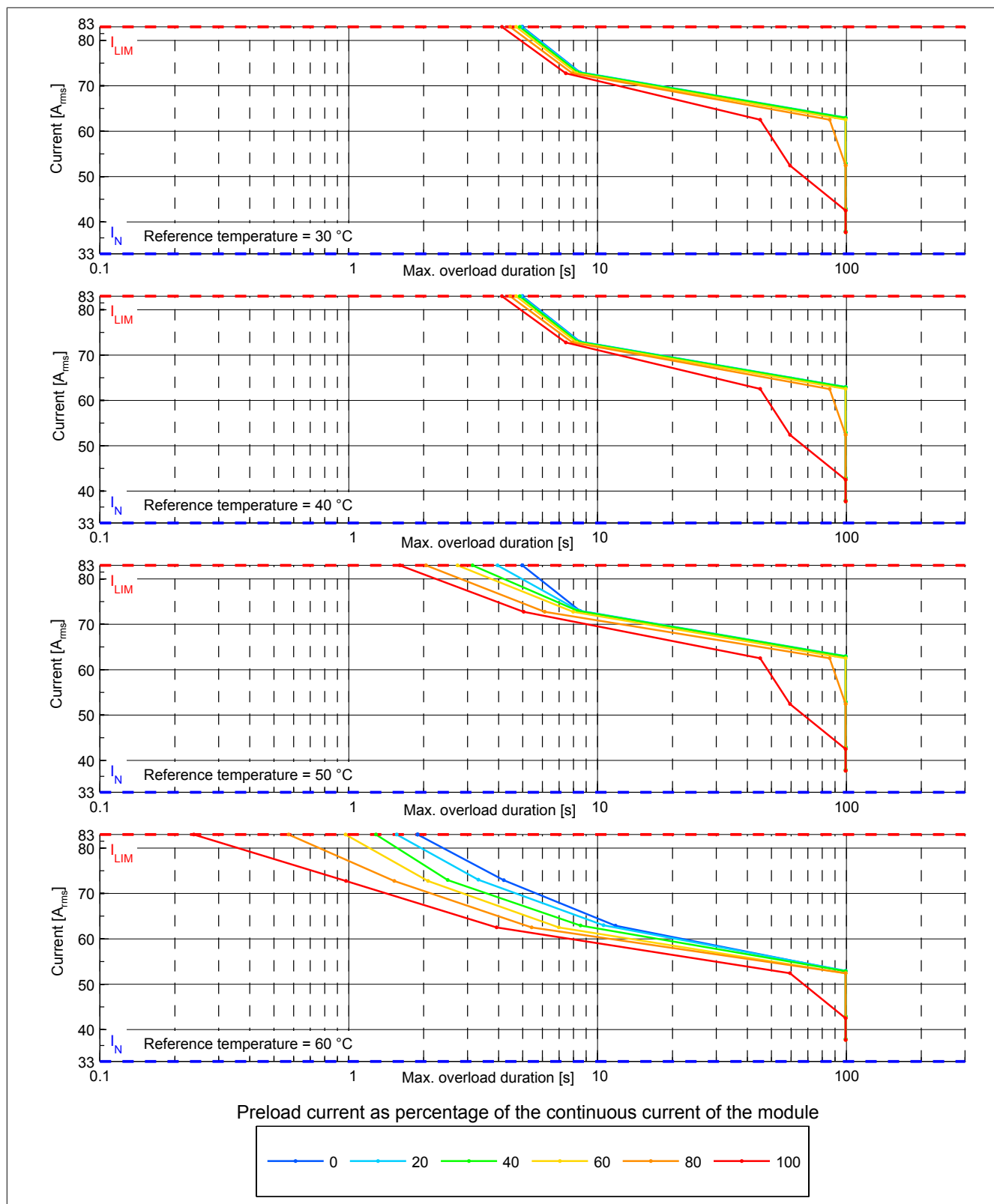
Figure 5: 8BVI0330HCSx.000-x - Overload characteristics, overload response - ERROR+STOP
