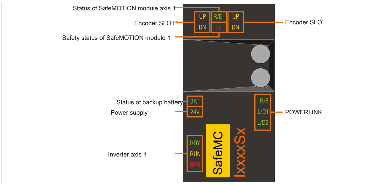
Figure 1: 8BVI SafeMOTION inverter modules (1-axis modules) - Status indicator groups 1)
