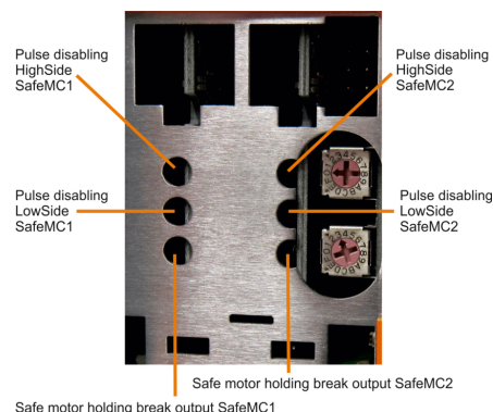
Figure 8: 2-axis modules
