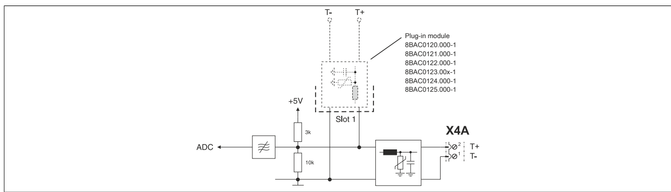
Figure 11: Temperature sensor
