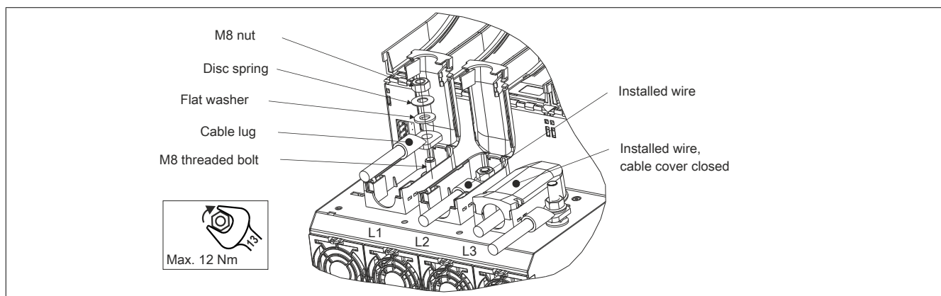
Figure 4: Mains connections L1, L2, L3 - Cable installation
