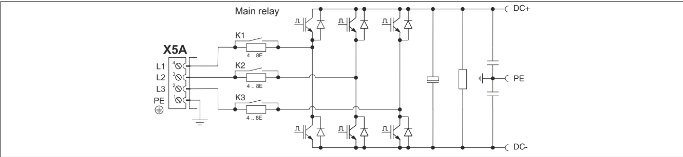
Figure 10: Power unit
