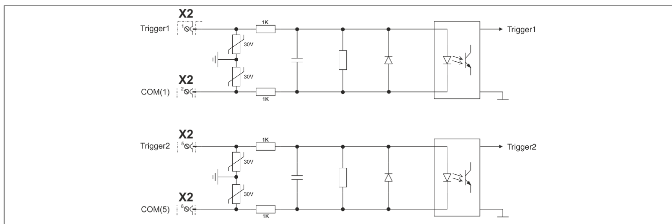
Figure 6: Trigger inputs
