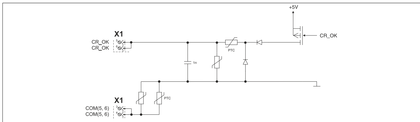
Figure 5: 8B0C enable
