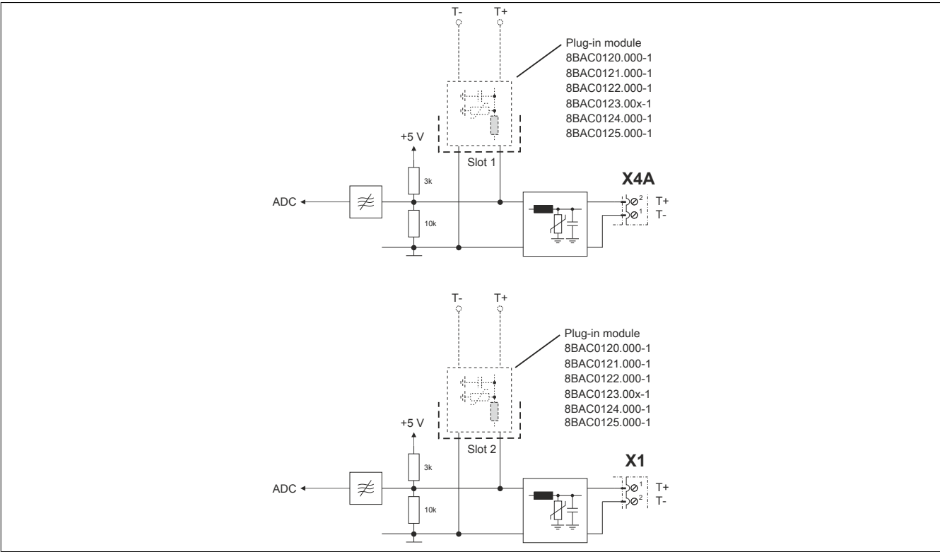
Figure 9: Temperature sensor
