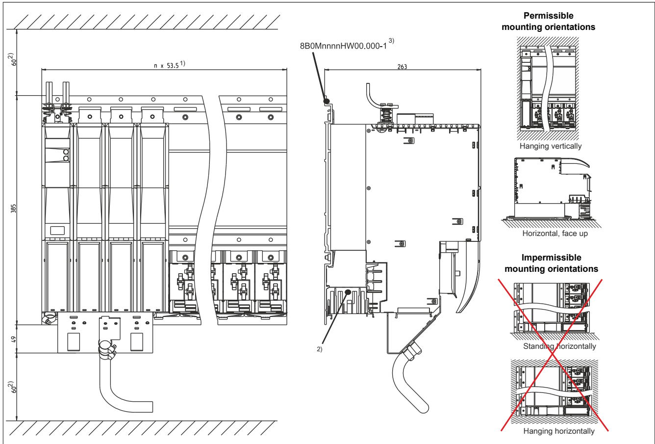
Figure 2: Dimension diagram and installation dimensions
