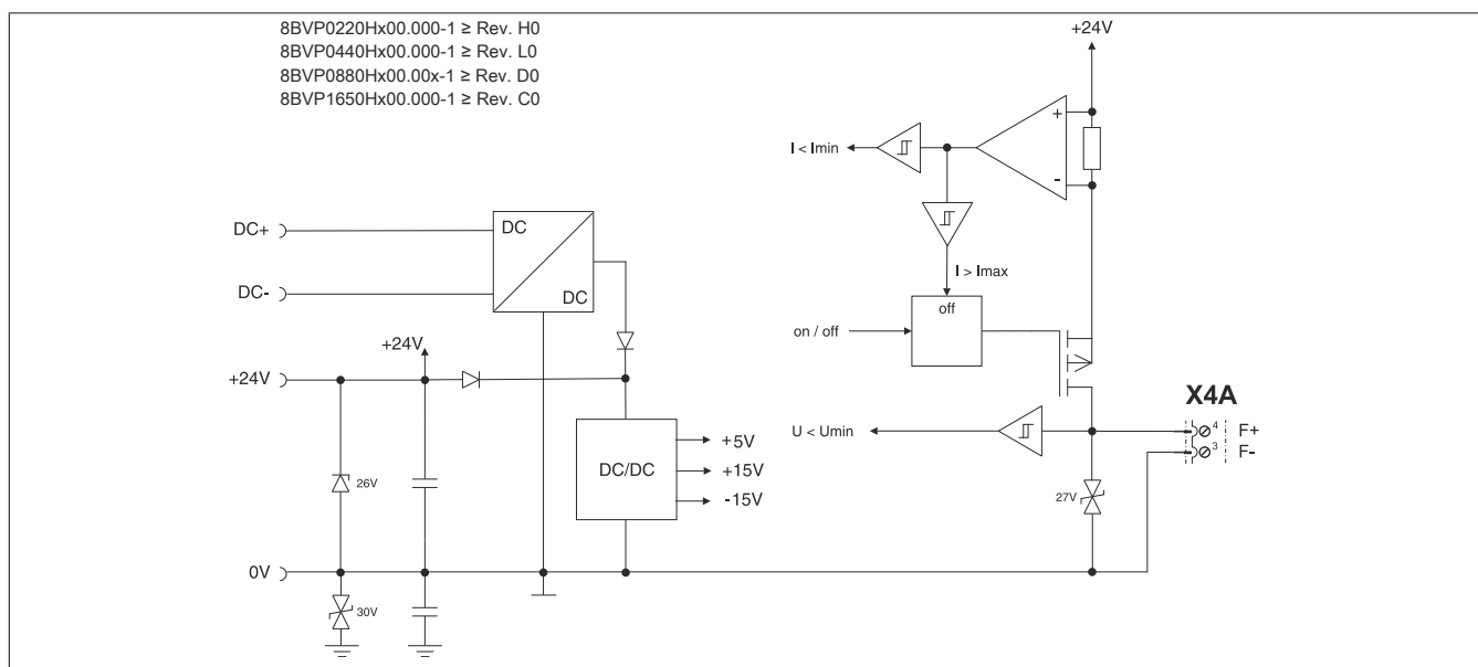
Figure 8: Internal 24 V generation and control of 8BVF fan
