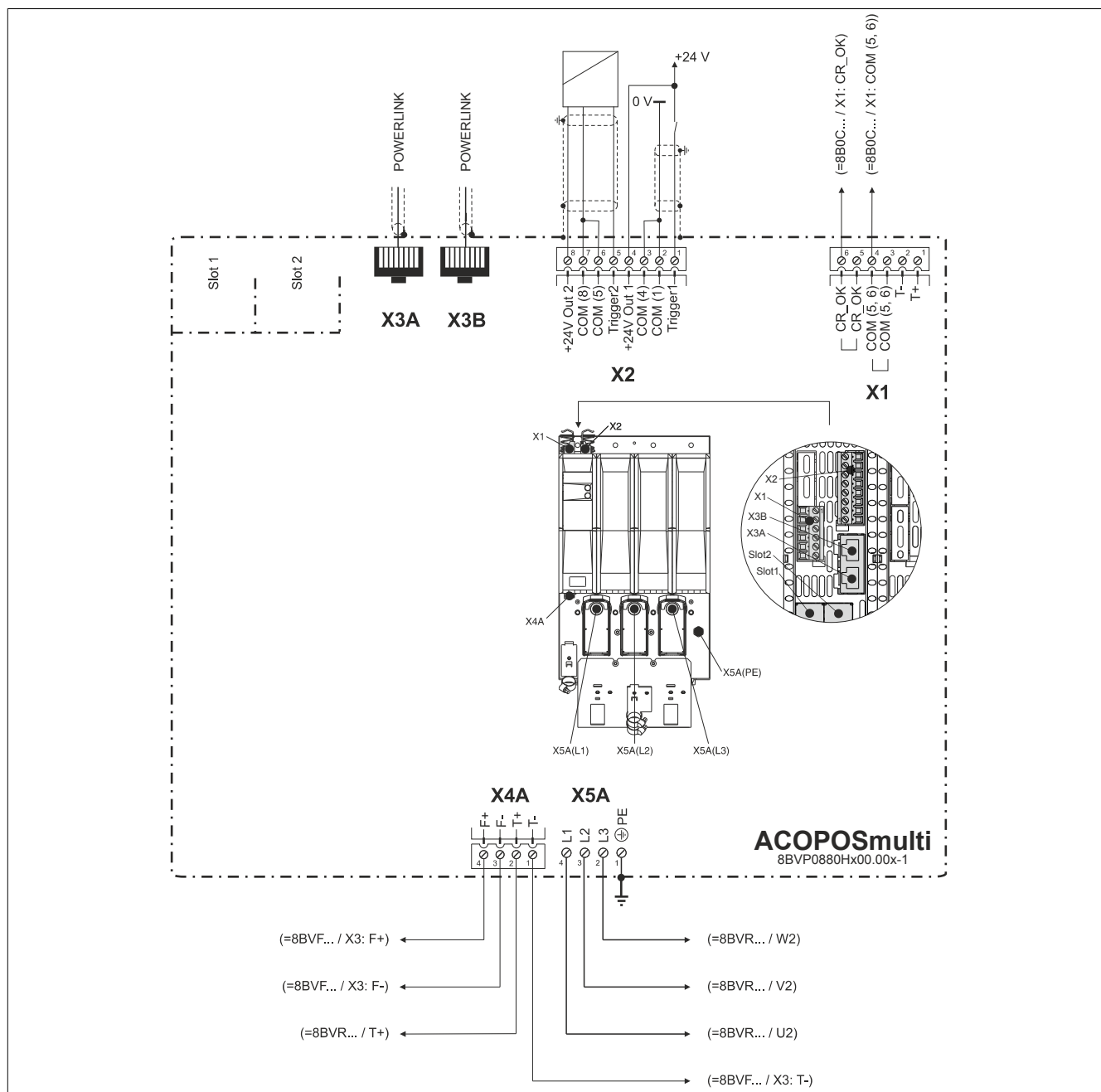
Figure 3: 8BVP0880Hx00.00x-1 - Pinout overview
