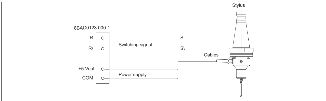
Figure 2: Connection example for cabled styli with 5 V power supply and TTL output signals
