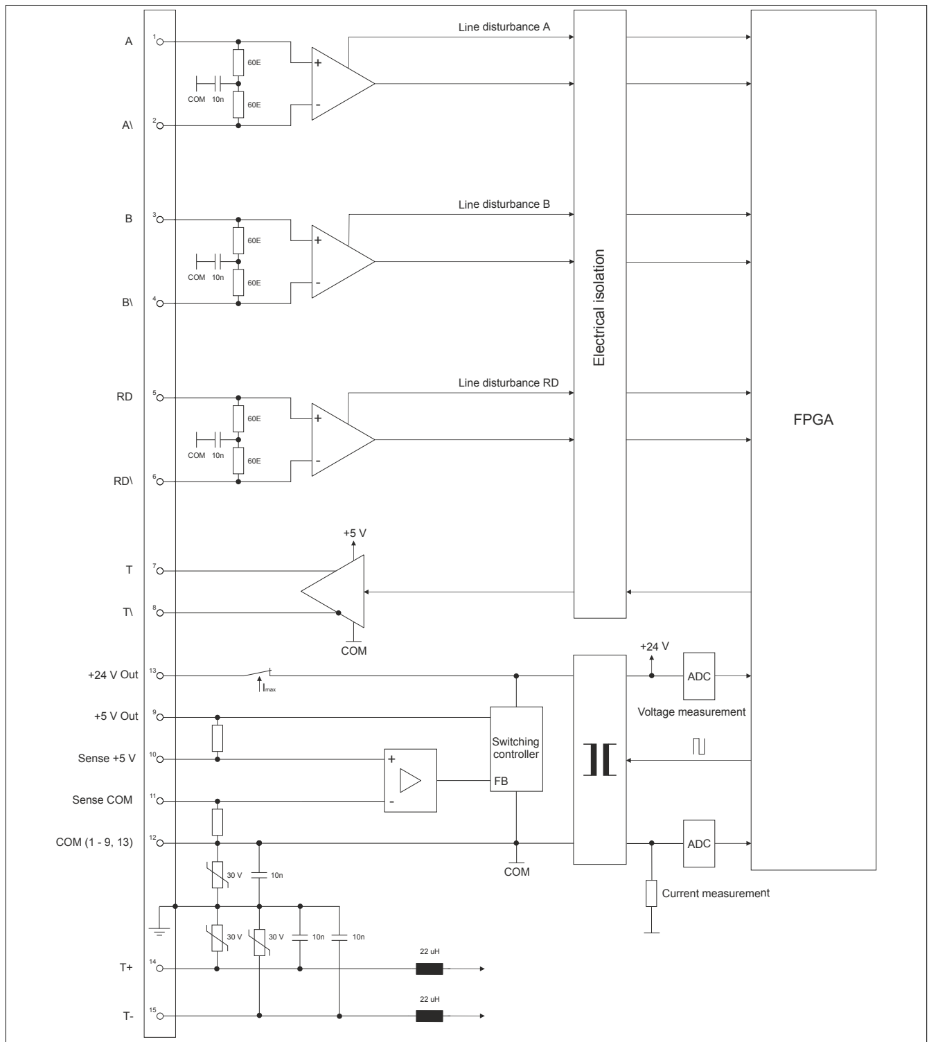
Figure 1: Incremental/SSI encoder interface 8BAC0123.000-1 - Input/Output circuit diagram
